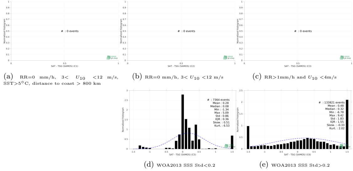
Figure 13: Normalized histogram of \Delta SSS (SMAP SSS L4 OI v1 - 7 Days (IPRC) - TSG (SAMOS)) for 5 different subdatasets corresponding to: RR=0 mm/h, 3 < U_{10} < 12 m/s, SST >5^{\circ}\text{C} , distance to coast > 800 km (a), RR=0 mm/h, 3 < U_{10} < 12 m/s (b), RR >1 mm/h and U_{10} < 4 m/s (c), WOA2013 SSS Std <0.2 (d), WOA2013 SSS Std >0.2 (e).
