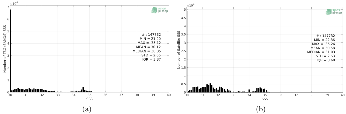
Figure 2: Histograms of SSS from TSG (SAMOS) (a) and SMAP SSS L4 OI v1 - 7day (IPRC) (b) considering all match-up pairs per bins of 0.1 over the Arctic Ocean Pi-MEP region and for the full satellite product period.
