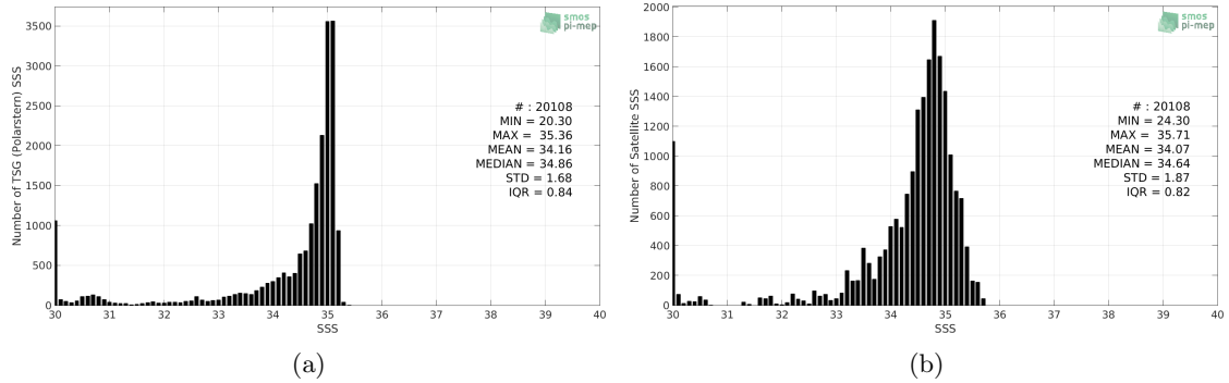
Figure 2: Histograms of SSS from TSG (Polarstern) (a) and SMAP SSS L4 OI v1 - 7 Days (IPRC) (b) considering all match-up pairs per bins of 0.1 over the Arctic Ocean Pi-MEP region and for the full satellite product period.
