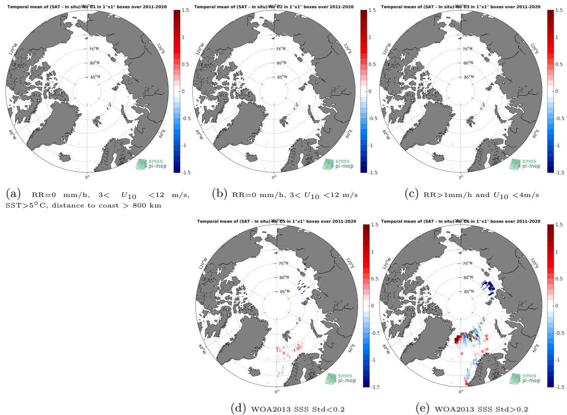
Figure 12: Temporal mean gridded over spatial boxes of size 1^{\circ}\times 1^{\circ} of \Delta\text{SSS} (SMAP SSS L4 OI v1 - 7 Days (IPRC) - TSG (Polarstern)) for 5 different subdatasets corresponding to:RR=0 mm/h, 3 < U_{10} < 12 m/s, SST > 5^{\circ}\text{C} , distance to coast > 800 km (a), RR=0 mm/h, 3 < U_{10} < 12 m/s (b), RR > 1 mm/h and U_{10} < 4 m/s (c), WOA2013 SSS Std < 0.2 (d), WOA2013 SSS Std > 0.2 (e).
