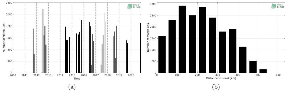
Figure 1: Number of match-ups between TSG (Polarstern) and SMAP SSS L4 OI v1 - 7 Days (IPRC) SSS as a function of time (a) and as function of the distance to coast (b) over the Arctic Ocean Pi-MEP region and for the full satellite product period.
