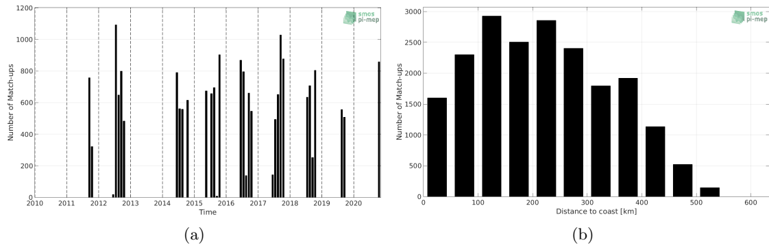
Figure 1: Number of match-ups between TSG (Polarstern) and SMAP SSS L4 OI v1 - 7day (IPRC) SSS as a function of time (a) and as function of the distance to coast (b) over the Arctic Ocean Pi-MEP region and for the full satellite product period.
