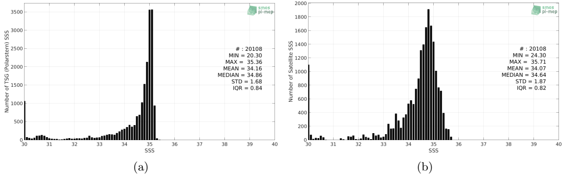
Figure 2: Histograms of SSS from TSG (Polarstern) (a) and SMAP SSS L4 OI v1 - 7day (IPRC) (b) considering all match-up pairs per bins of 0.1 over the Arctic Ocean Pi-MEP region and for the full satellite product period.
