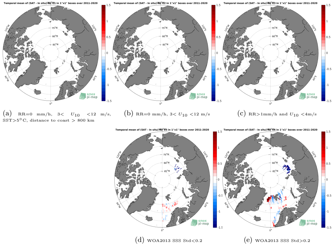
Figure 12: Temporal mean gridded over spatial boxes of size 1^{\circ}\times 1^{\circ} of \Delta\text{SSS} (SMAP SSS L4 OI v1 - 7day (IPRC) - TSG (Polarstern)) for 5 different subdatasets corresponding to: RR=0 mm/h, 3 < U_{10} < 12 m/s, SST > 5^{\circ}\text{C} , distance to coast > 800 km (a), RR=0 mm/h, 3 < U_{10} < 12 m/s (b), RR > 1 mm/h and U_{10} < 4 m/s (c), WOA2013 SSS Std < 0.2 (d), WOA2013 SSS Std > 0.2 (e).
