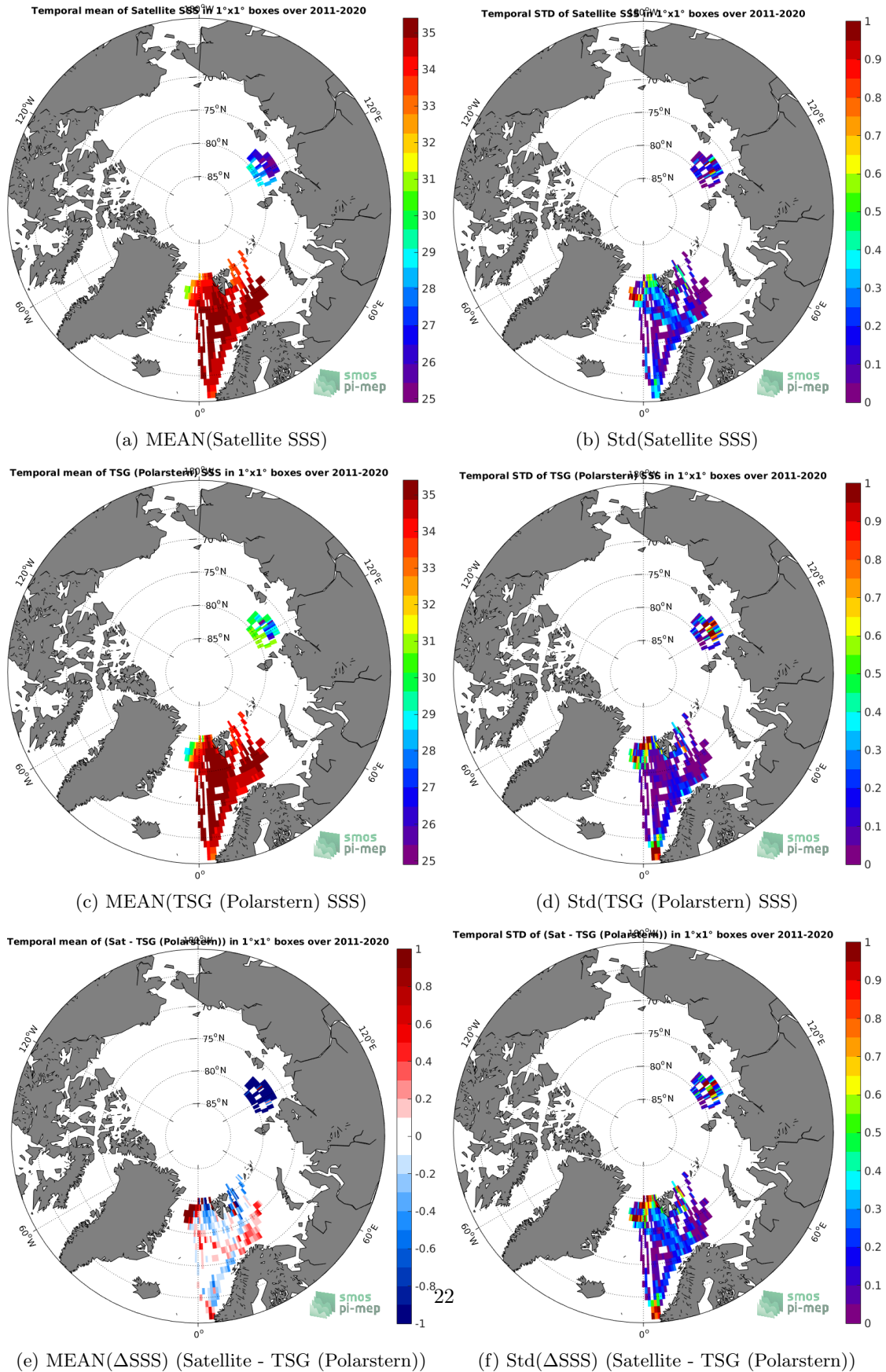
Figure 6: Temporal mean (left) and Std (right) of SSS from SMAP SSS L4 OI v1 - 7day (IPRC) (top), TSG (Polarstern) (middle), and of \Delta SSS (Satellite - TSG (Polarstern)). Only match-up pairs are used to generate these maps.
