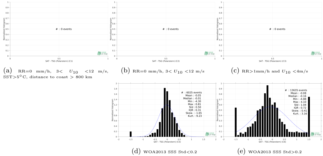
Figure 13: Normalized histogram of \Delta SSS (SMAP SSS L4 OI v1 - 7day (IPRC) - TSG (Polarstern)) for 5 different subdatasets corresponding to: RR=0 mm/h, 3 < U_{10} < 12 m/s, SST > 5°C, distance to coast > 800 km (a), RR=0 mm/h, 3 < U_{10} < 12 m/s (b), RR > 1mm/h and U_{10} < 4 m/s (c), WOA2013 SSS Std < 0.2 (d), WOA2013 SSS Std > 0.2 (e).
