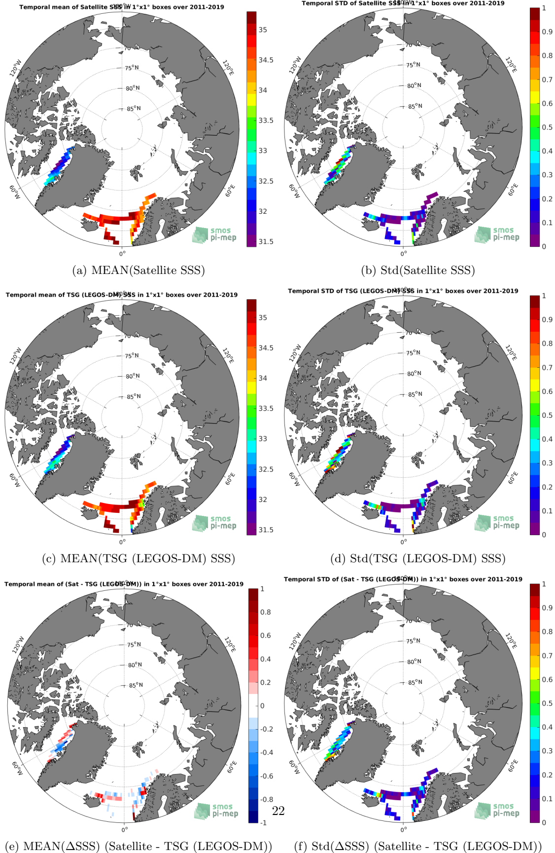
Figure 6: Temporal mean (left) and Std (right) of SSS from SMAP SSS L4 OI v1 - 7 Days (IPRC) (top), TSG (LEGOS-DM) (middle), and of \Delta SSS (Satellite - TSG (LEGOS-DM)). Only match-up pairs are used to generate these maps.
