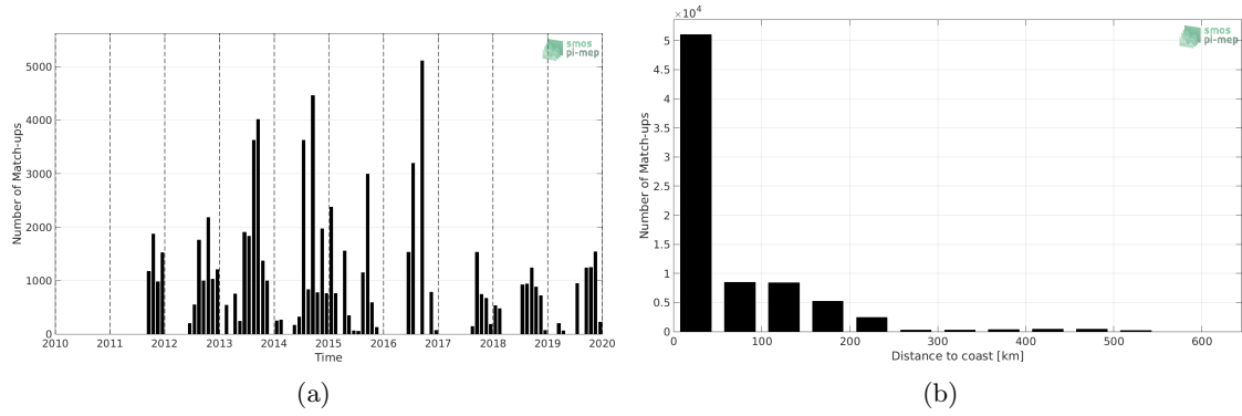
Figure 1: Number of match-ups between TSG (LEGOS-DM) and SMAP SSS L4 OI v1 - 7 Days (IPRC) SSS as a function of time (a) and as function of the distance to coast (b) over the Arctic Ocean Pi-MEP region and for the full satellite product period.
