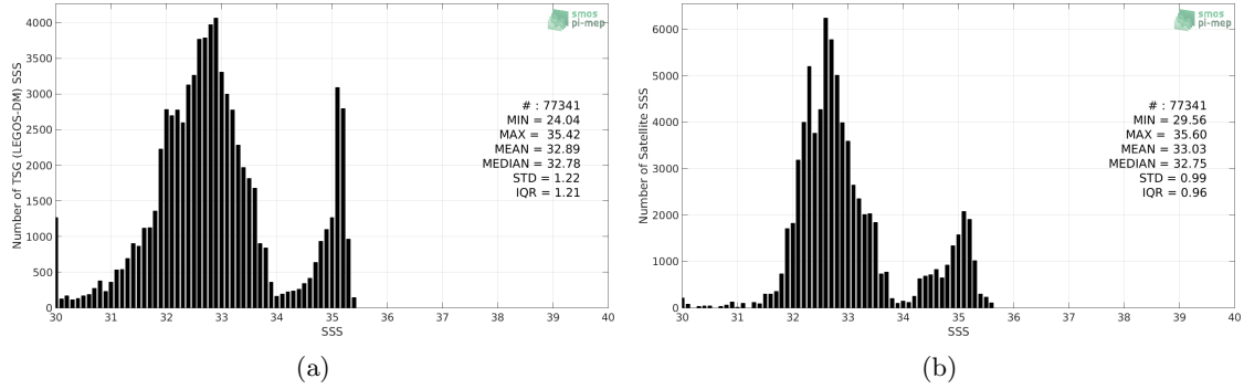
Figure 2: Histograms of SSS from TSG (LEGOS-DM) (a) and SMAP SSS L4 OI v1 - 7 Days (IPRC) (b) considering all match-up pairs per bins of 0.1 over the Arctic Ocean Pi-MEP region and for the full satellite product period.
