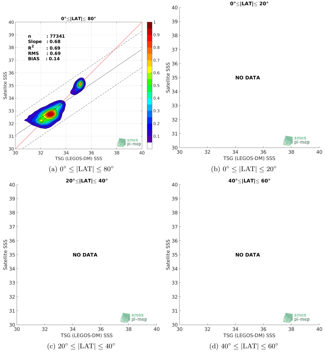
Figure 9: Contour maps of the concentration of SMAP SSS L4 OI v1 - 7 Days (IPRC) SSS (y-axis) versus TSG (LEGOS-DM) SSS (x-axis) at match-up pairs for different latitude bands. For each plot, the red line shows x=y . The black thin and dashed lines indicate a linear fit through the data cloud and the \pm 95\% confidence levels, respectively. The number match-up pairs n , the slope and R^2 coefficient of the linear fit, the root mean square (RMS) and the mean bias between satellite and in situ data are indicated for each latitude band in each plots.
