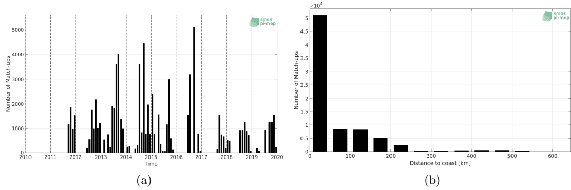
Figure 1: Number of match-ups between TSG (LEGOS-DM) and SMAP SSS L4 OI v1 - 7day (IPRC) SSS as a function of time (a) and as function of the distance to coast (b) over the Arctic Ocean Pi-MEP region and for the full satellite product period.
