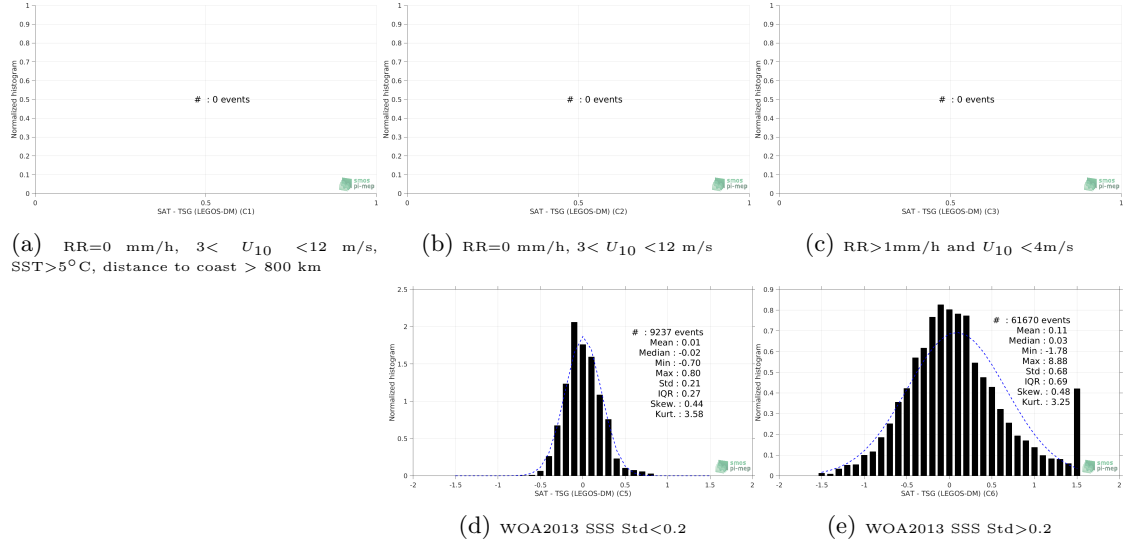
Figure 13: Normalized histogram of \Delta\text{SSS} (SMAP SSS L4 OI v1 - 7day (IPRC) - TSG (LEGOS-DM)) for 5 different subdatasets corresponding to: RR=0 mm/h, 3 < U_{10} < 12 m/s, SST > 5^\circ\text{C} , distance to coast > 800 km (a), RR=0 mm/h, 3 < U_{10} < 12 m/s (b), RR > 1 mm/h and U_{10} < 4 m/s (c), WOA2013 SSS Std < 0.2 (d), WOA2013 SSS Std > 0.2 (e).
