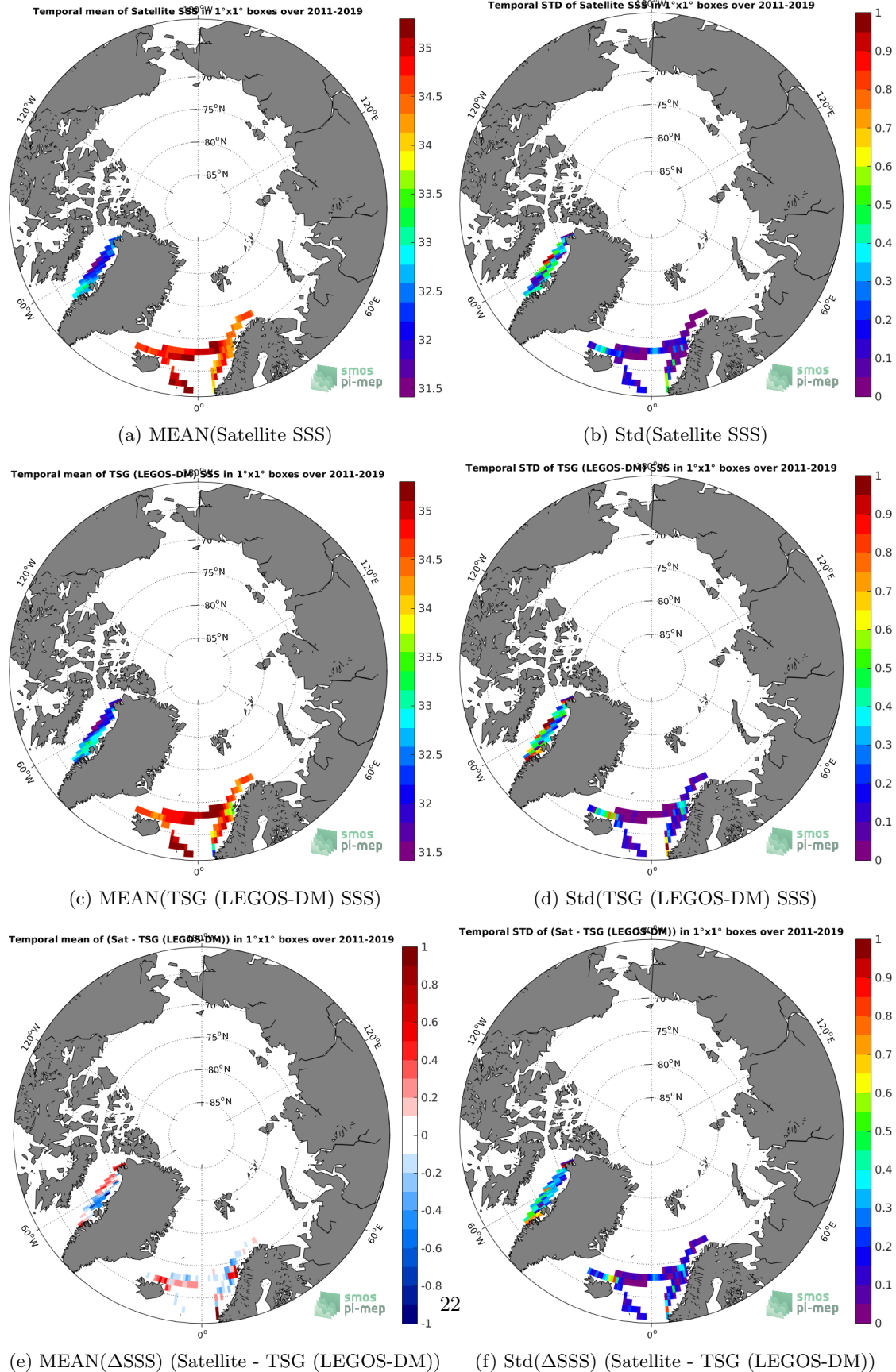
Figure 6: Temporal mean (left) and Std (right) of SSS from SMAP SSS L4 OI v1 - 7day (IPRC) (top), TSG (LEGOS-DM) (middle), and of \Delta SSS (Satellite - TSG (LEGOS-DM)). Only match-up pairs are used to generate these maps.
