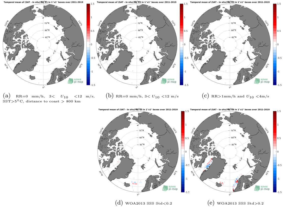
Figure 12: Temporal mean gridded over spatial boxes of size 1^{\circ}\times 1^{\circ} of \Delta\text{SSS} (SMAP SSS L4 OI v1 - 7day (IPRC) - TSG (LEGOS-DM)) for 5 different subdatasets corresponding to: RR=0 mm/h, 3 < U_{10} < 12 m/s, SST >5^{\circ}\text{C} , distance to coast > 800 km (a), RR=0 mm/h, 3 < U_{10} < 12 m/s (b), RR >1 mm/h and U_{10} < 4 m/s (c), WOA2013 SSS Std <0.2 (d), WOA2013 SSS Std >0.2 (e).
