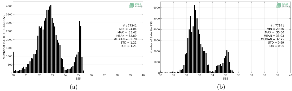
Figure 2: Histograms of SSS from TSG (LEGOS-DM) (a) and SMAP SSS L4 OI v1 - 7day (IPRC) (b) considering all match-up pairs per bins of 0.1 over the Arctic Ocean Pi-MEP region and for the full satellite product period.
