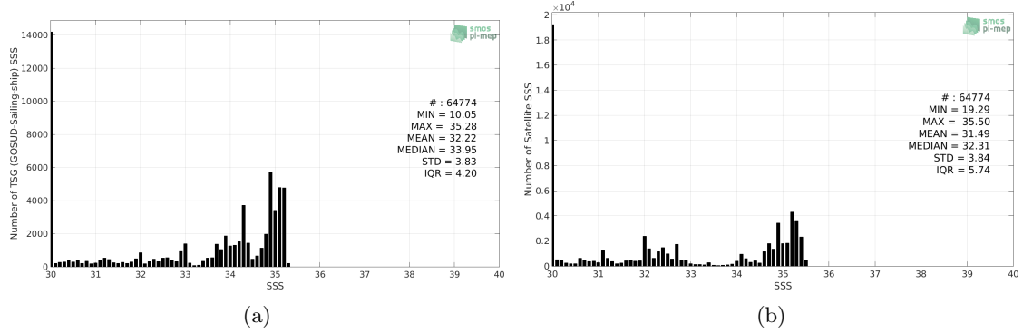
Figure 2: Histograms of SSS from TSG (GOSUD-Sailing-ship) (a) and SMAP SSS L4 OI v1 - 7 Days (IPRC) (b) considering all match-up pairs per bins of 0.1 over the Arctic Ocean Pi-MEP region and for the full satellite product period.
