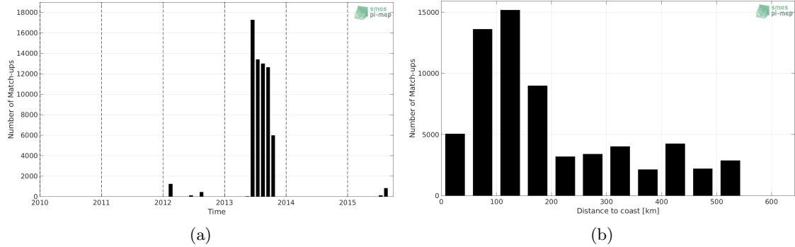
Figure 1: Number of match-ups between TSG (GOSUD-Sailing-ship) and SMAP SSS L4 OI v1 - 7 Days (IPRC) SSS as a function of time (a) and as function of the distance to coast (b) over the Arctic Ocean Pi-MEP region and for the full satellite product period.
