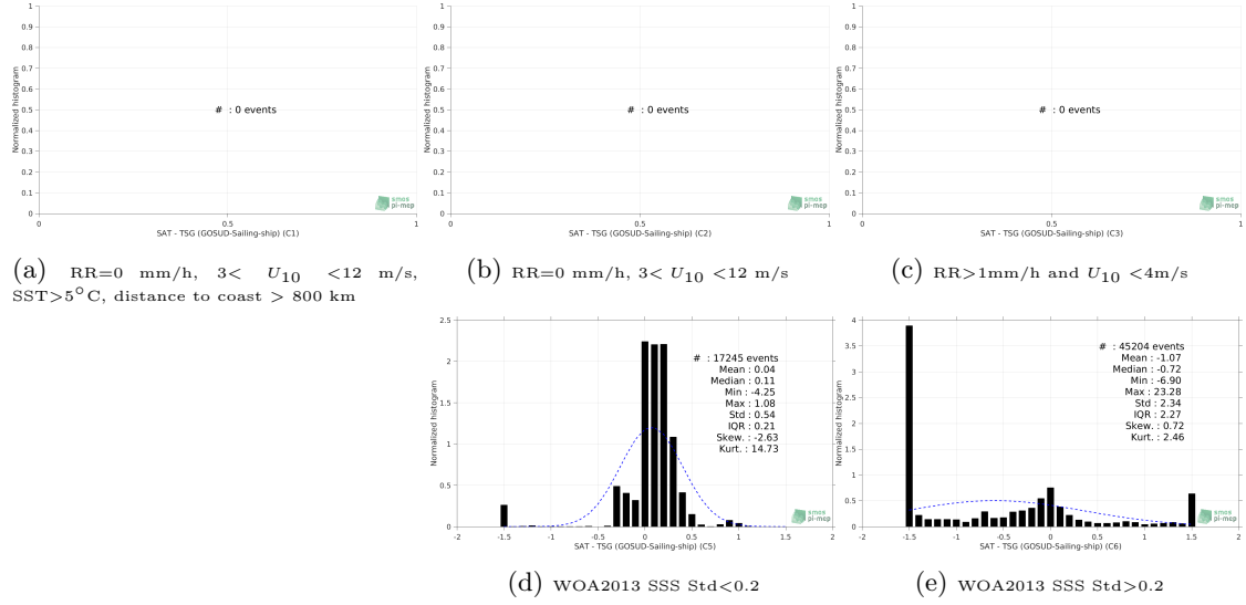
Figure 13: Normalized histogram of \Delta\text{SSS} (SMAP SSS L4 OI v1 - 7 Days (IPRC) - TSG (GOSUD-Sailing-ship)) for 5 different subdatasets corresponding to: RR=0 mm/h, 3 < U_{10} < 12 m/s, SST > 5^\circ\text{C} , distance to coast > 800 km (a), RR=0 mm/h, 3 < U_{10} < 12 m/s (b), RR > 1\text{mm/h} and U_{10} < 4\text{m/s} (c), WOA2013 SSS Std<0.2 (d), WOA2013 SSS Std>0.2 (e).
