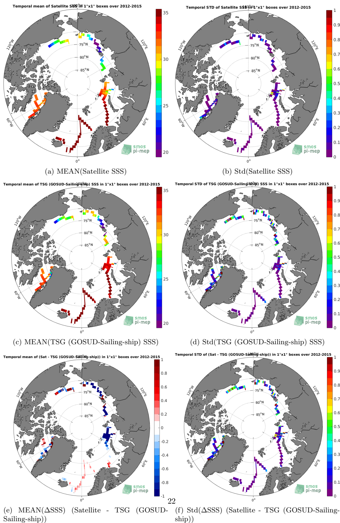
Figure 6: Temporal mean (left) and Std (right) of SSS from SMAP SSS L4 OI v1 - 7 Days (IPRC) (top), TSG (GOSUD-Sailing-ship) (middle), and of \Delta SSS (Satellite - TSG (GOSUD-Sailing-ship)). Only match-up pairs are used to generate these maps.
