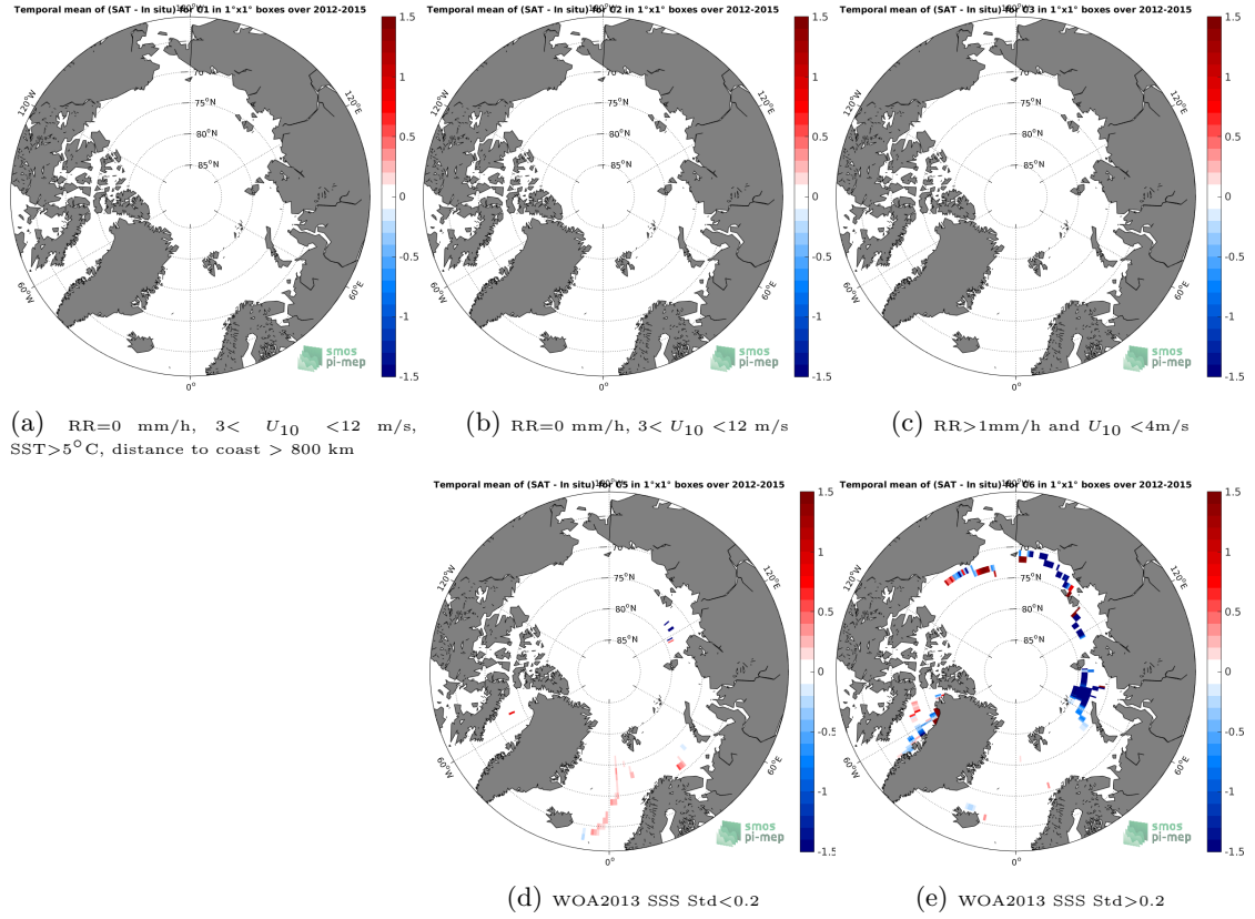
Figure 12: Temporal mean gridded over spatial boxes of size 1^\circ \times 1^\circ of \Delta SSS (SMAP SSS L4 OI v1 - 7 Days (IPRC) - TSG (GOSUD-Sailing-ship)) for 5 different subdatasets corresponding to: RR=0 mm/h, 3 < U_{10} < 12 m/s, SST > 5^\circ\text{C} , distance to coast > 800 km (a), RR=0 mm/h, 3 < U_{10} < 12 m/s (b), RR > 1 mm/h and U_{10} < 4 m/s (c), WOA2013 SSS Std < 0.2 (d), WOA2013 SSS Std > 0.2 (e).
