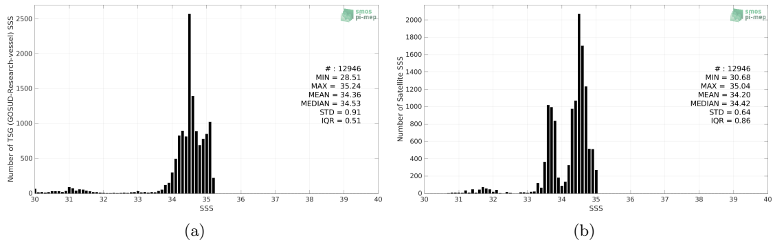
Figure 2: Histograms of SSS from TSG (GOSUD-Research-vessel) (a) and SMAP SSS L4 OI v1 - 7 Days (IPRC) (b) considering all match-up pairs per bins of 0.1 over the Arctic Ocean Pi-MEP region and for the full satellite product period.
