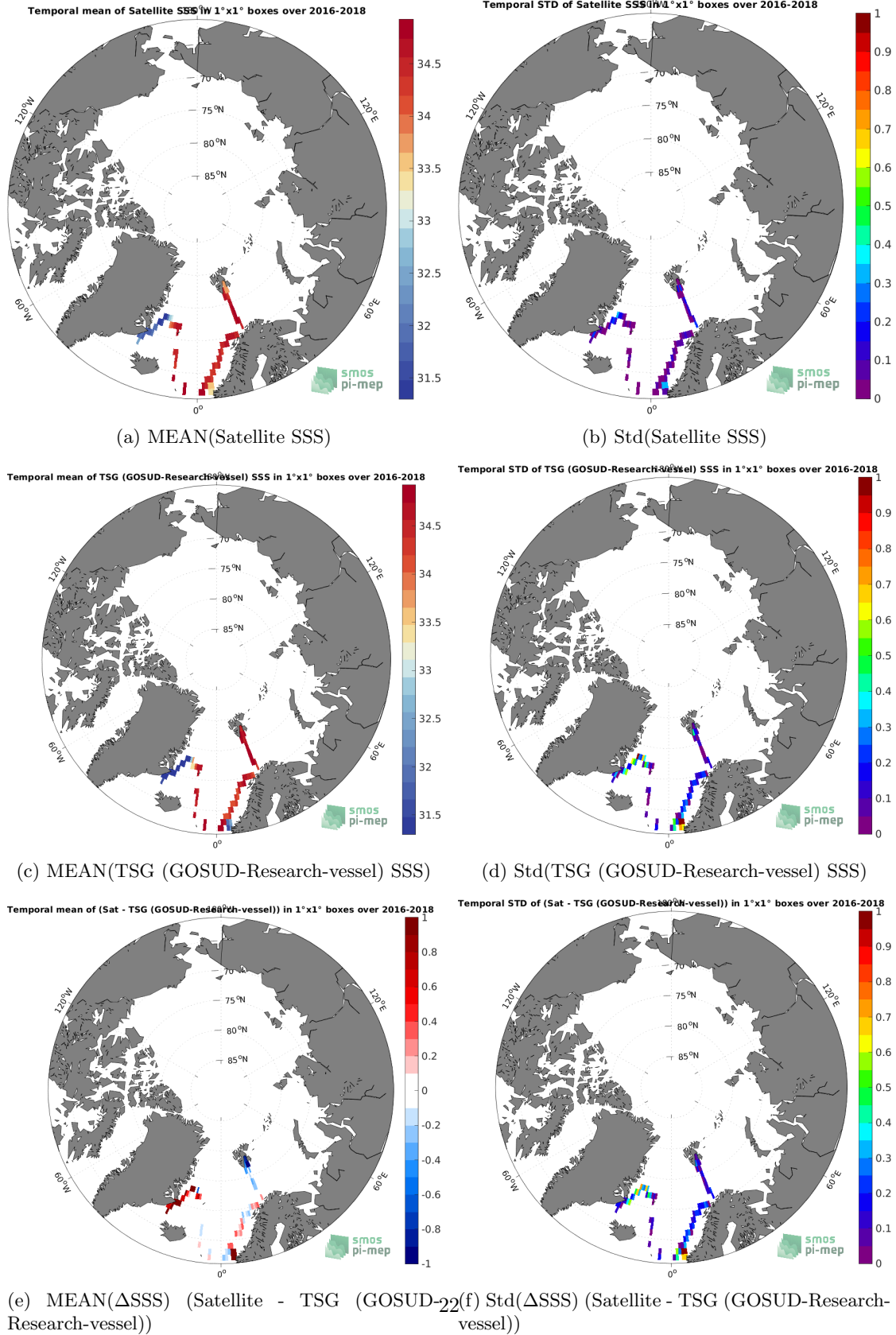
Figure 6: Temporal mean (left) and Std (right) of SSS from SMAP SSS L4 OI v1 - 7 Days (IPRC) (top), TSG (GOSUD-Research-vessel) (middle), and of \Delta SSS (Satellite - TSG (GOSUD-Research-vessel)). Only match-up pairs are used to generate these maps.
