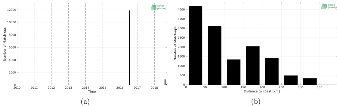
Figure 1: Number of match-ups between TSG (GOSUD-Research-vessel) and SMAP SSS L4 OI v1 - 7 Days (IPRC) SSS as a function of time (a) and as function of the distance to coast (b) over the Arctic Ocean Pi-MEP region and for the full satellite product period.
