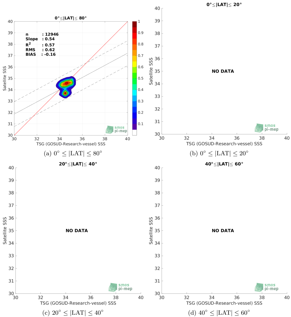
Figure 9: Contour maps of the concentration of SMAP SSS L4 OI v1 - 7 Days (IPRC) SSS (y-axis) versus TSG (GOSUD-Research-vessel) SSS (x-axis) at match-up pairs for different latitude bands. For each plot, the red line shows x=y . The black thin and dashed lines indicate a linear fit through the data cloud and the \pm 95\% confidence levels, respectively. The number match-up pairs n , the slope and R^2 coefficient of the linear fit, the root mean square (RMS) and the mean bias between satellite and in situ data are indicated for each latitude band in each plots.
