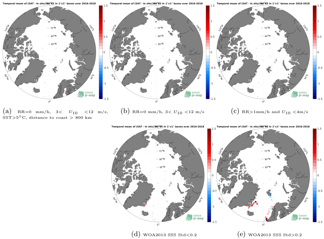
Figure 12: Temporal mean gridded over spatial boxes of size 1^\circ \times 1^\circ of \Delta SSS (SMAP SSS L4 OI v1 - 7 Days (IPRC) - TSG (GOSUD-Research-vessel)) for 5 different subdatasets corresponding to: RR=0 mm/h, 3 < U_{10} < 12 m/s, SST>5°C, distance to coast > 800 km (a), RR=0 mm/h, 3 < U_{10} < 12 m/s (b), RR>1mm/h and U_{10} < 4 m/s (c), WOA2013 SSS Std<0.2 (d), WOA2013 SSS Std>0.2 (e).
