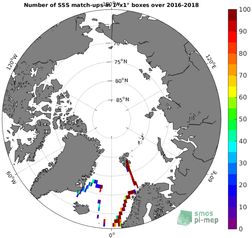
Figure 4: Number of SSS match-ups between TSG (GOSUD-Research-vessel) SSS and the SMAP SSS L4 OI v1 - 7day (IPRC) SSS product for the Arctic Ocean Pi-MEP region over 1°x1° boxes and for the full satellite product period.
