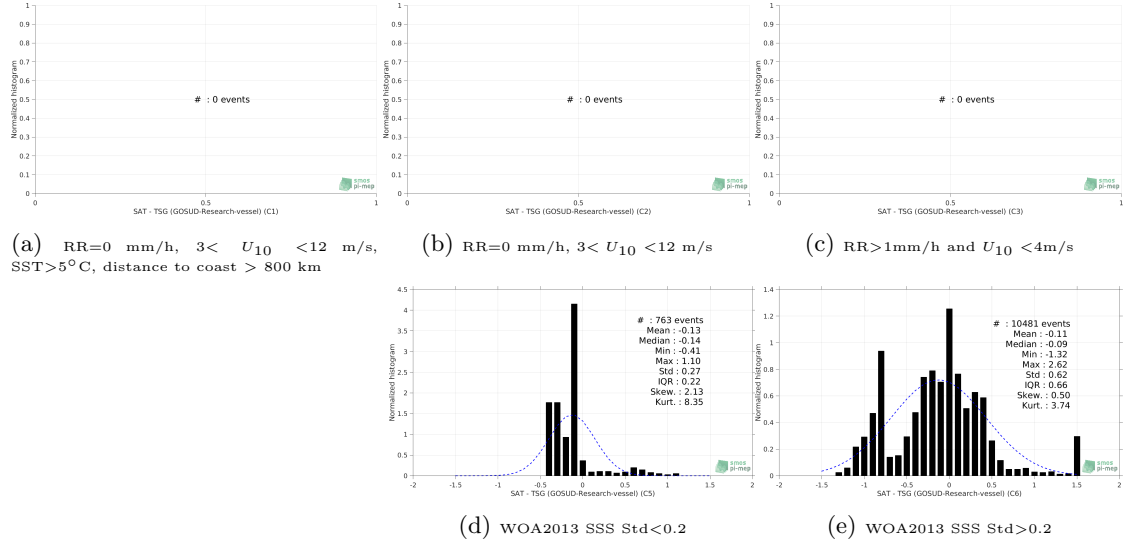
Figure 13: Normalized histogram of \Delta SSS (SMAP SSS L4 OI v1 - 7day (IPRC) - TSG (GOSUD-Research-vessel)) for 5 different subdatasets corresponding to: RR=0 mm/h, 3 < U_{10} < 12 m/s, SST >5^{\circ} C, distance to coast > 800 km (a), RR=0 mm/h, 3 < U_{10} < 12 m/s (b), RR >1 mm/h and U_{10} < 4 m/s (c), WOA2013 SSS Std <0.2 (d), WOA2013 SSS Std >0.2 (e).
