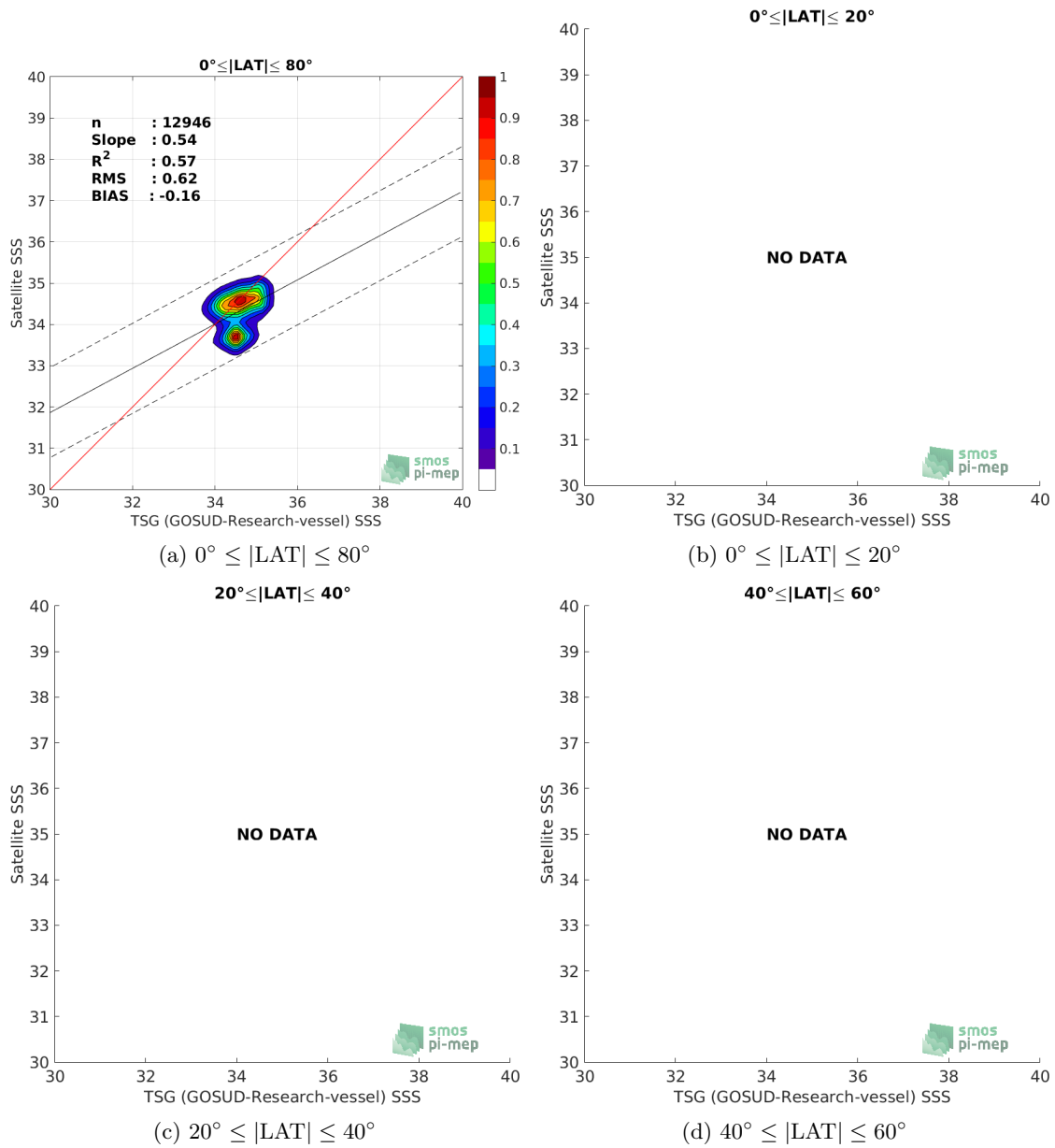
Figure 9: Contour maps of the concentration of SMAP SSS L4 OI v1 - 7day (IPRC) SSS (y-axis) versus TSG (GOSUD-Research-vessel) SSS (x-axis) at match-up pairs for different latitude bands. For each plot, the red line shows x=y . The black thin and dashed lines indicate a linear fit through the data cloud and the \pm 95\% confidence levels, respectively. The number match-up pairs n , the slope and R^2 coefficient of the linear fit, the root mean square (RMS) and the mean bias between satellite and in situ data are indicated for each latitude band in each plots.
