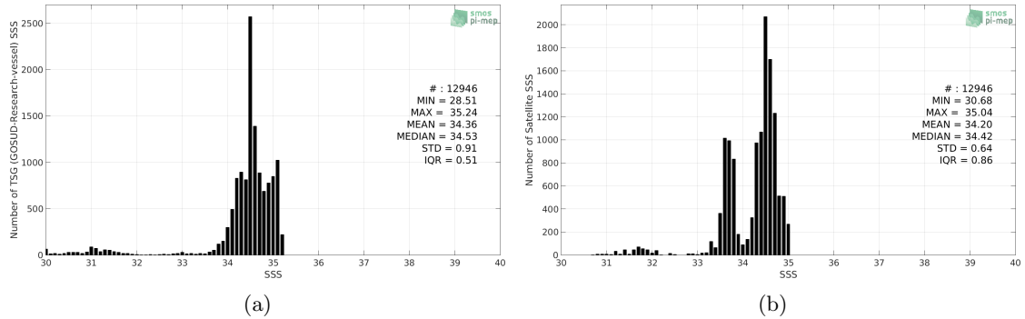
Figure 2: Histograms of SSS from TSG (GOSUD-Research-vessel) (a) and SMAP SSS L4 OI v1 - 7day (IPRC) (b) considering all match-up pairs per bins of 0.1 over the Arctic Ocean Pi-MEP region and for the full satellite product period.
