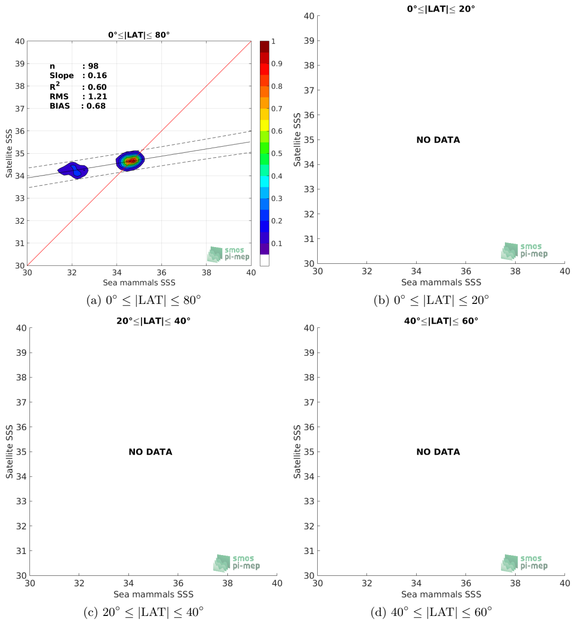
Figure 9: Contour maps of the concentration of SMAP SSS L4 OI v1 - 7 Days (IPRC) SSS (y-axis) versus Marine mammals SSS (x-axis) at match-up pairs for different latitude bands. For each plot, the red line shows x=y . The black thin and dashed lines indicate a linear fit through the data cloud and the \pm 95\% confidence levels, respectively. The number match-up pairs n , the slope and R^2 coefficient of the linear fit, the root mean square (RMS) and the mean bias between satellite and in situ data are indicated for each latitude band in each plots.
