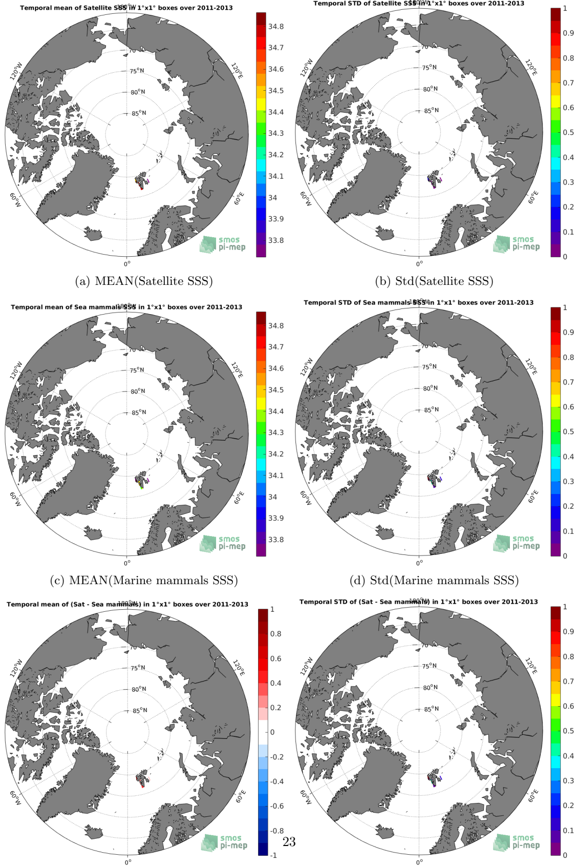
(e) MEAN( \Delta SSS) (Satellite - Marine mammals)
