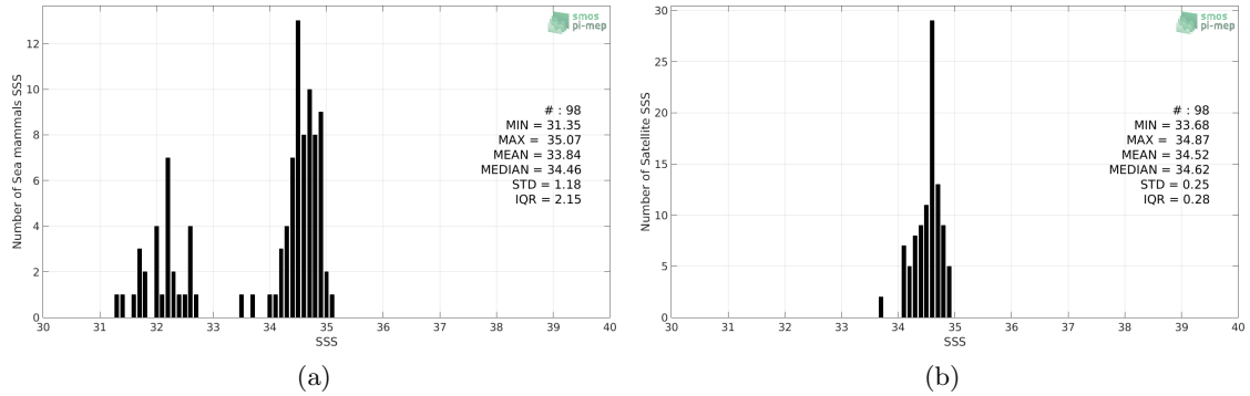
Figure 2: Histograms of SSS from Marine mammals (a) and SMAP SSS L4 OI v1 - 7 Days (IPRC) (b) considering all match-up pairs per bins of 0.1 over the Arctic Ocean Pi-MEP region and for the full satellite product period.
