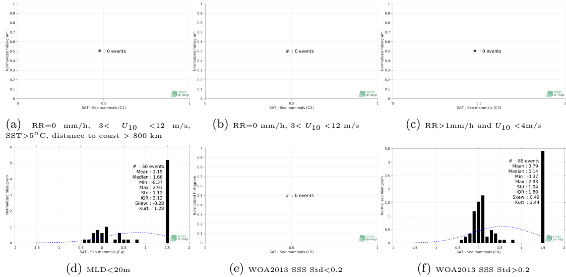
Figure 13: Normalized histogram of \Delta SSS (SMAP SSS L4 OI v1 - 7 Days (IPRC) - Marine mammals) for 6 different subdatasets corresponding to: RR=0 mm/h, 3 < U_{10} < 12 m/s, SST > 5°C, distance to coast > 800 km (a), RR=0 mm/h, 3 < U_{10} < 12 m/s (b), RR > 1mm/h and U_{10} < 4 m/s (c), MLD < 20m (d), WOA2013 SSS Std < 0.2 (e), WOA2013 SSS Std > 0.2 (f).
