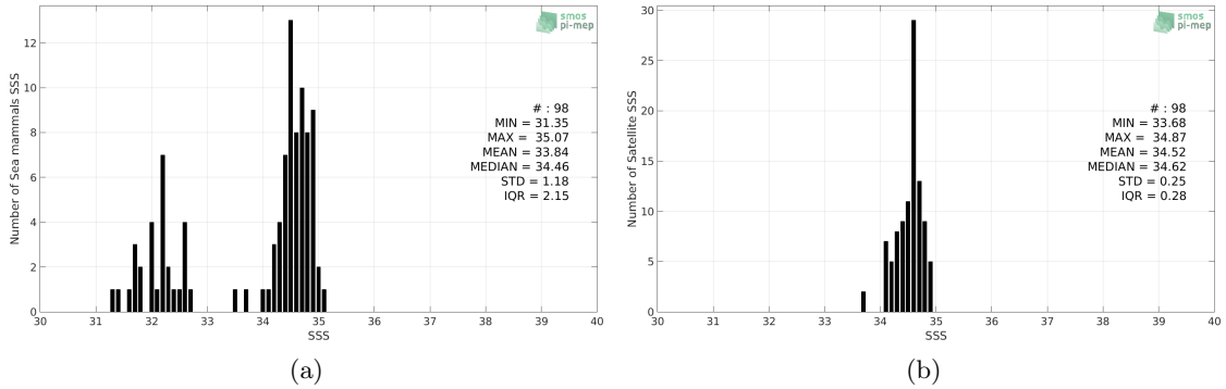
Figure 2: Histograms of SSS from Sea mammals (a) and SMAP SSS L4 OI v1 - 7day (IPRC) (b) considering all match-up pairs per bins of 0.1 over the Arctic Ocean Pi-MEP region and for the full satellite product period.
