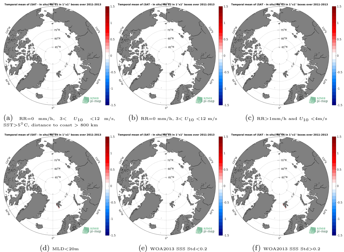
Figure 12: Temporal mean gridded over spatial boxes of size 1^{\circ}\times 1^{\circ} of \Delta\text{SSS} (SMAP SSS L4 OI v1 - 7day (IPRC) - Sea mammals) for 6 different subdatasets corresponding to:RR=0 mm/h, 3 < U_{10} < 12 m/s, SST > 5^{\circ}\text{C} , distance to coast > 800 km (a), RR=0 mm/h, 3 < U_{10} < 12 m/s (b), RR > 1 mm/h and U_{10} < 4 m/s (c),MLD < 20\text{m} (d),WOA2013 SSS Std < 0.2 (e),WOA2013 SSS Std > 0.2 (f).
