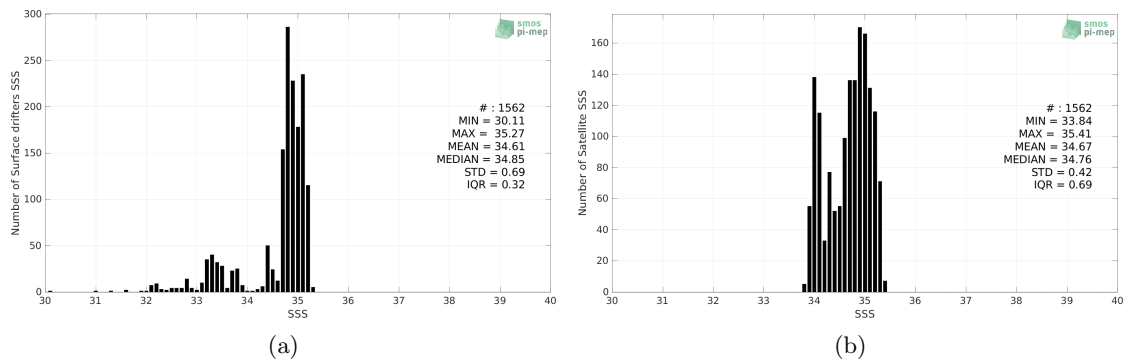
Figure 2: Histograms of SSS from Surface drifters (a) and SMAP SSS L4 OI v1 - 7 Days (IPRC) (b) considering all match-up pairs per bins of 0.1 over the Arctic Ocean Pi-MEP region and for the full satellite product period.
