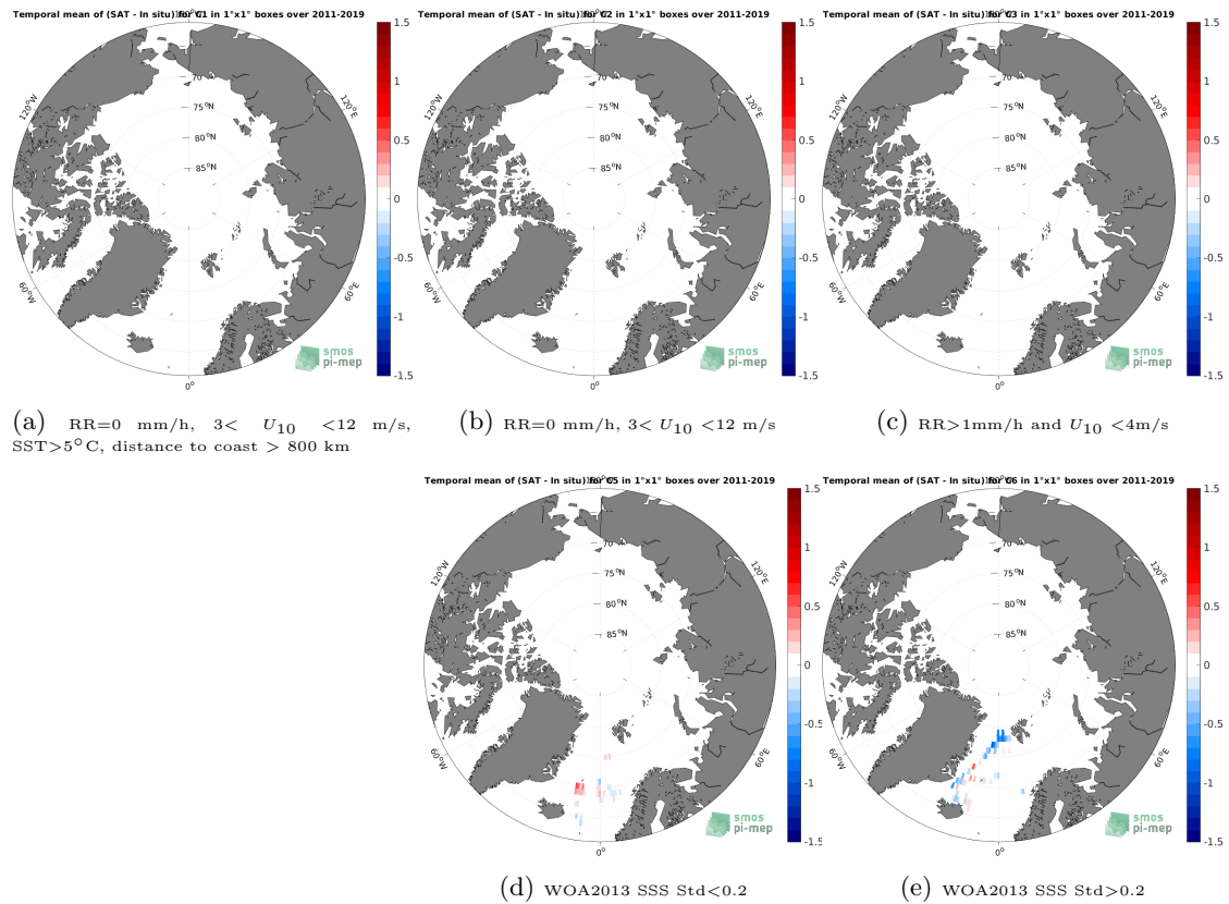
Figure 11: Temporal mean gridded over spatial boxes of size 1^{\circ}\times 1^{\circ} of \Delta\text{SSS} (SMAP SSS L4 OI v1 - 7 Days (IPRC) - Surface drifters) for 5 different subdatasets corresponding to:RR=0 mm/h, 3 < U_{10} < 12 m/s, SST > 5^{\circ}\text{C} , distance to coast > 800 km (a), RR=0 mm/h, 3 < U_{10} < 12 m/s (b), RR > 1 mm/h and U_{10} < 4 m/s (c), WOA2013 SSS Std < 0.2 (d), WOA2013 SSS Std > 0.2 (e).
