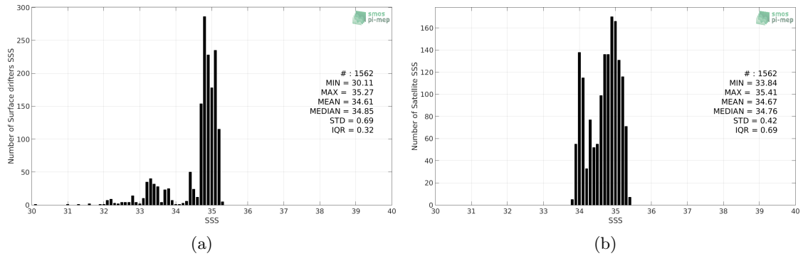
Figure 2: Histograms of SSS from Surface drifters (a) and SMAP SSS L4 OI v1 - 7day (IPRC) (b) considering all match-up pairs per bins of 0.1 over the Arctic Ocean Pi-MEP region and for the full satellite product period.
