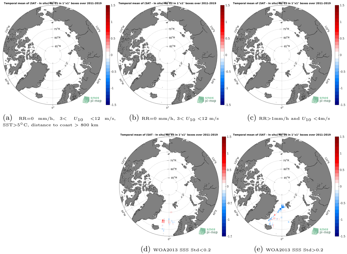
Figure 11: Temporal mean gridded over spatial boxes of size 1^{\circ}\times 1^{\circ} of \Delta\text{SSS} (SMAP SSS L4 OI v1 - 7day (IPRC) - Surface drifters) for 5 different subdatasets corresponding to:RR=0 mm/h, 3 < U_{10} < 12 m/s, SST > 5^{\circ}\text{C} , distance to coast > 800 km (a), RR=0 mm/h, 3 < U_{10} < 12 m/s (b), RR > 1 mm/h and U_{10} < 4 m/s (c), WOA2013 SSS Std < 0.2 (d), WOA2013 SSS Std > 0.2 (e).
