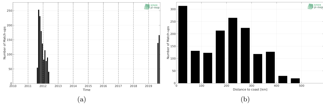
Figure 1: Number of match-ups between Surface drifters and SMAP SSS L4 OI v1 - 7day (IPRC) SSS as a function of time (a) and as function of the distance to coast (b) over the Arctic Ocean Pi-MEP region and for the full satellite product period.
