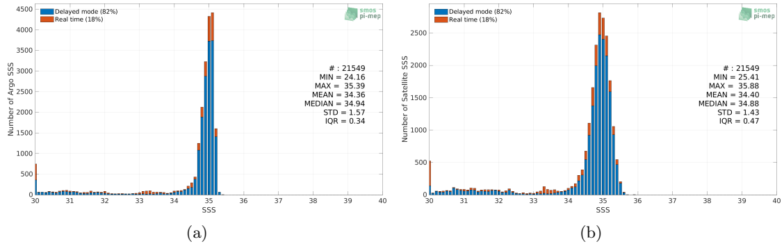
Figure 2: Histograms of SSS from Argo (a) and SMAP SSS L4 OI v1 - 7 Days (IPRC) (b) considering all match-up pairs per bins of 0.1 over the Arctic Ocean Pi-MEP region and for the full satellite product period.
