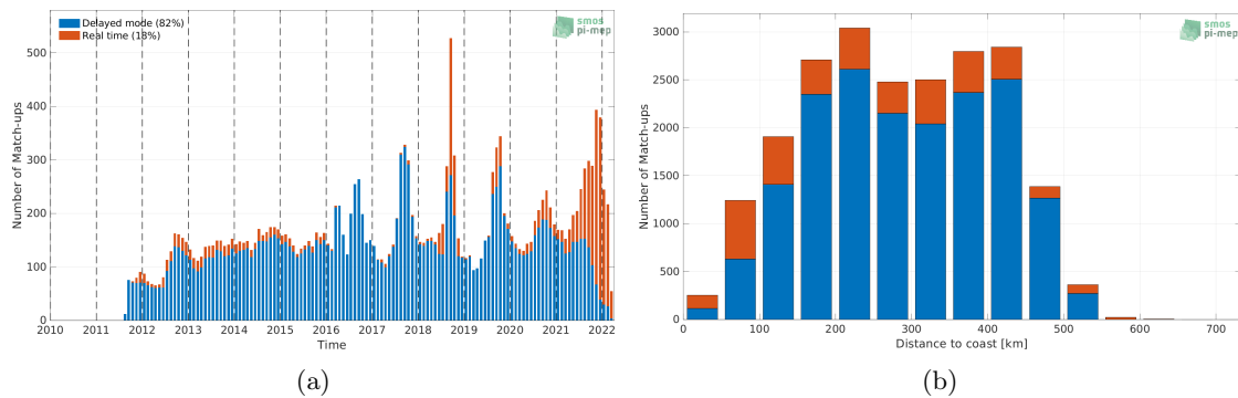
Figure 1: Number of match-ups between Argo and SMAP SSS L4 OI v1 - 7 Days (IPRC) SSS as a function of time (a) and as function of the distance to coast (b) over the Arctic Ocean Pi-MEP region and for the full satellite product period.
