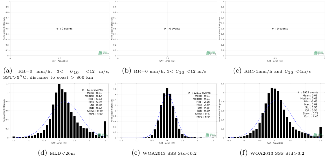
Figure 13: Normalized histogram of \Delta SSS (SMAP SSS L4 OI v1 - 7 Days (IPRC) - Argo) for 6 different subdatasets corresponding to: RR=0 mm/h, 3 < U_{10} < 12 m/s, SST > 5°C, distance to coast > 800 km (a), RR=0 mm/h, 3 < U_{10} < 12 m/s (b), RR > 1mm/h and U_{10} < 4 m/s (c), MLD < 20m (d), WOA2013 SSS Std < 0.2 (e), WOA2013 SSS Std > 0.2 (f).
