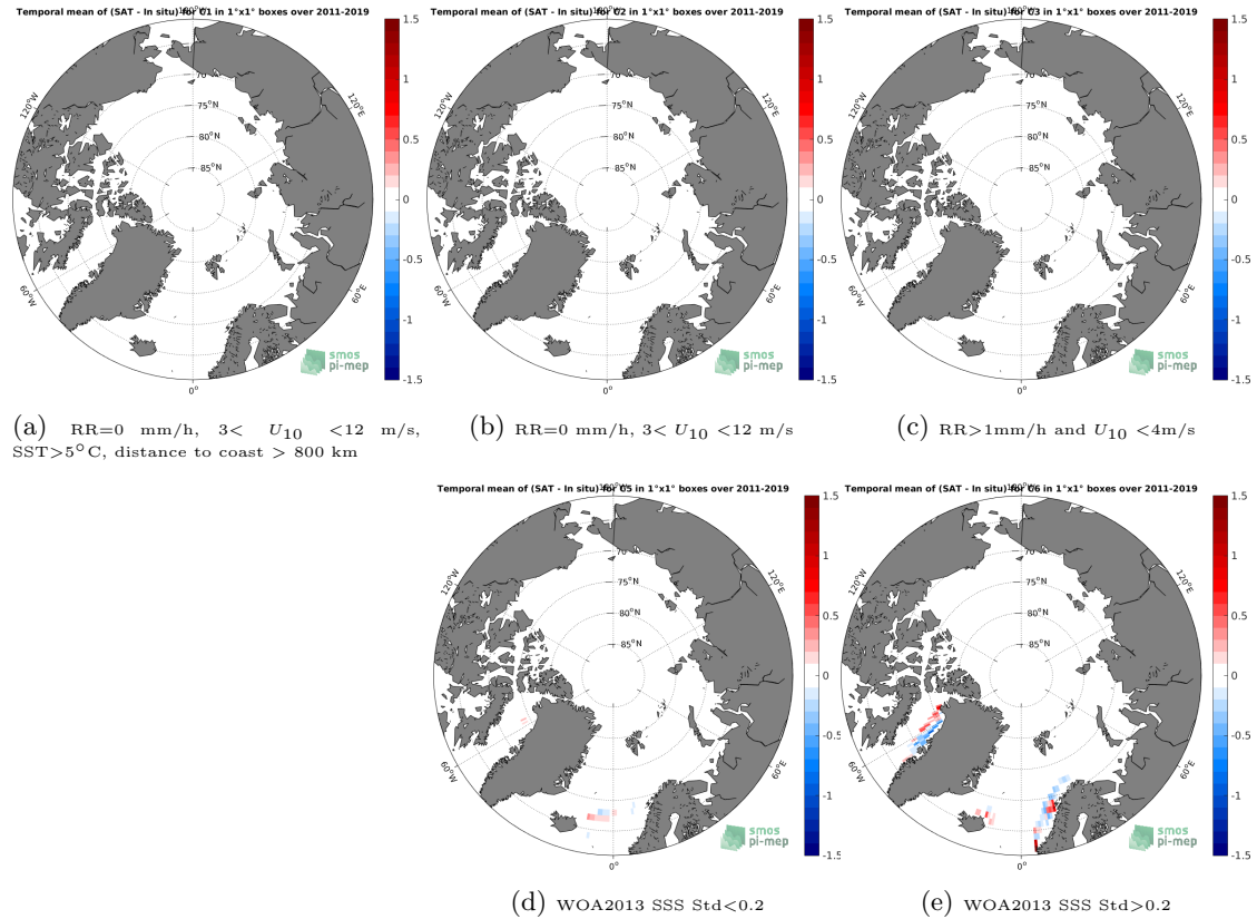
Figure 12: Temporal mean gridded over spatial boxes of size 1^{\circ}\times 1^{\circ} of \Delta\text{SSS} (SMAP SSS L4 OI v1 - Monthly (IPRC) - TSG (LEGOS-DM)) for 5 different subdatasets corresponding to:RR=0 mm/h, 3 < U_{10} < 12 m/s, SST > 5^{\circ}\text{C} , distance to coast > 800 km (a), RR=0 mm/h, 3 < U_{10} < 12 m/s (b), RR > 1 mm/h and U_{10} < 4 m/s (c), WOA2013 SSS Std < 0.2 (d), WOA2013 SSS Std > 0.2 (e).
