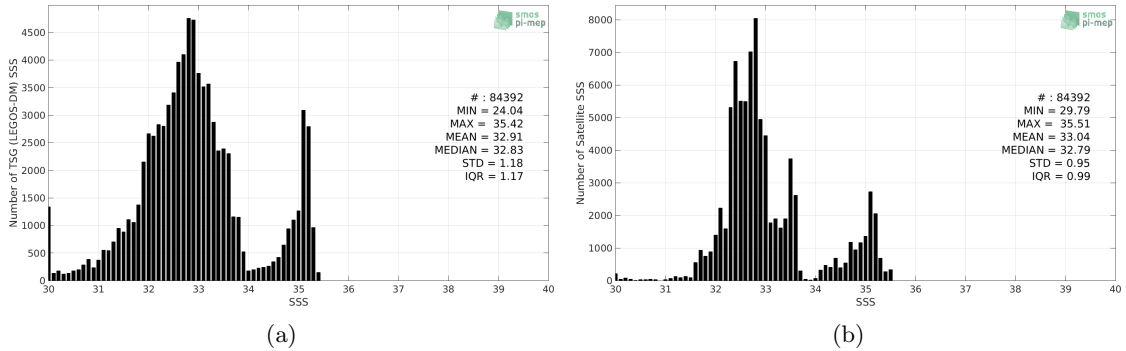
Figure 2: Histograms of SSS from TSG (LEGOS-DM) (a) and SMAP SSS L4 OI v1 - Monthly (IPRC) (b) considering all match-up pairs per bins of 0.1 over the Arctic Ocean Pi-MEP region and for the full satellite product period.
