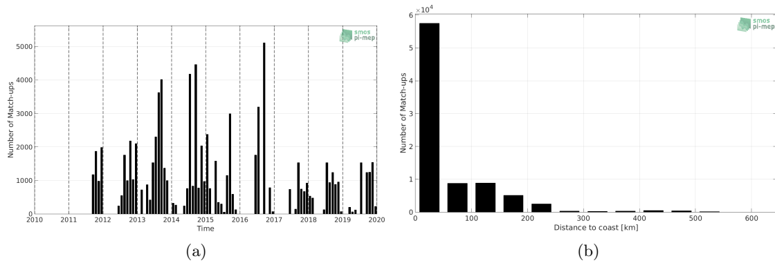
Figure 1: Number of match-ups between TSG (LEGOS-DM) and SMAP SSS L4 OI v1 - Monthly (IPRC) SSS as a function of time (a) and as function of the distance to coast (b) over the Arctic Ocean Pi-MEP region and for the full satellite product period.
