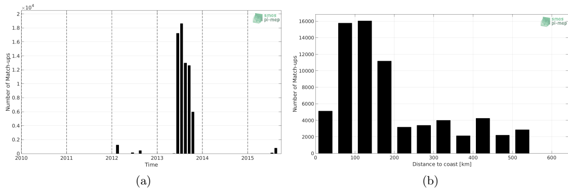
Figure 1: Number of match-ups between TSG (GOSUD-Sailing-ship) and SMAP SSS L4 OI v1 - Monthly (IPRC) SSS as a function of time (a) and as function of the distance to coast (b) over the Arctic Ocean Pi-MEP region and for the full satellite product period.
