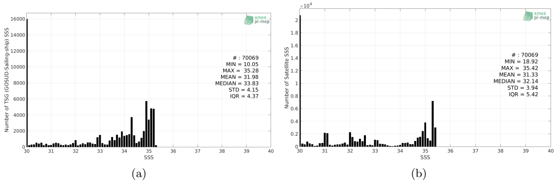
Figure 2: Histograms of SSS from TSG (GOSUD-Sailing-ship) (a) and SMAP SSS L4 OI v1 - Monthly (IPRC) (b) considering all match-up pairs per bins of 0.1 over the Arctic Ocean Pi-MEP region and for the full satellite product period.
