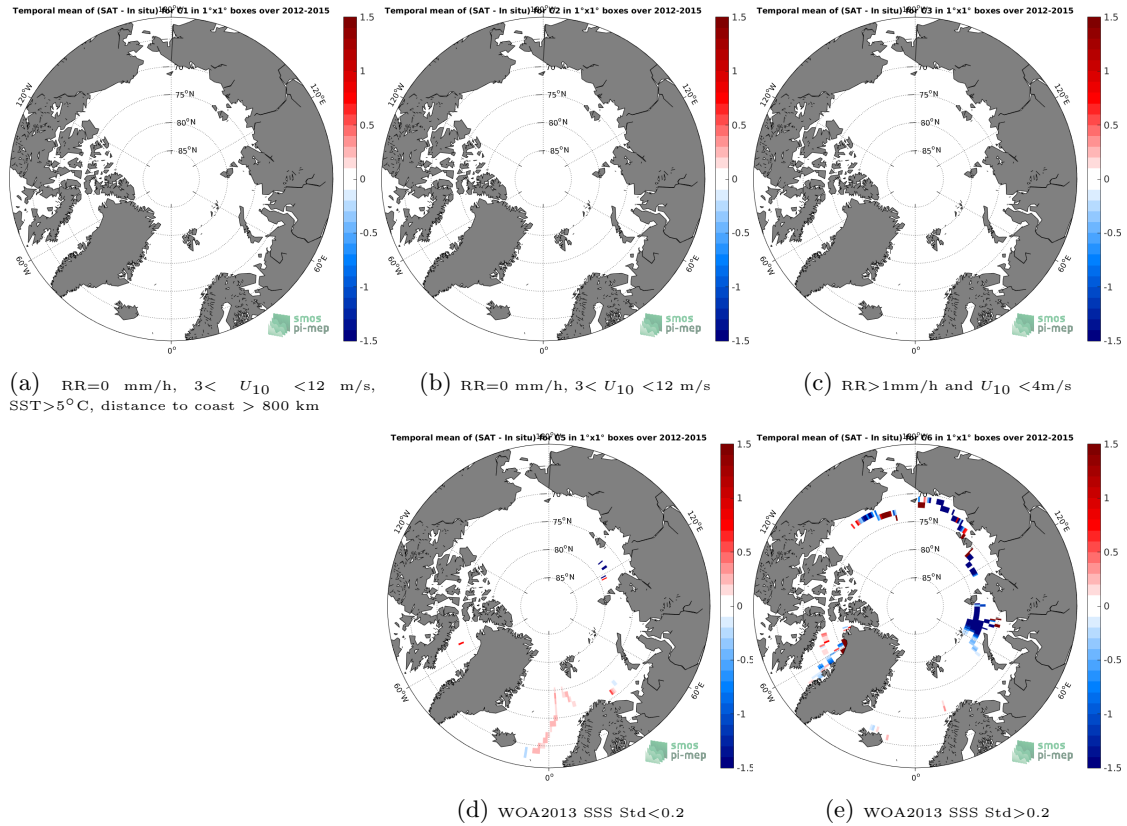
Figure 12: Temporal mean gridded over spatial boxes of size 1^\circ \times 1^\circ of \Delta SSS (SMAP SSS L4 OI v1 - Monthly (IPRC) - TSG (GOSUD-Sailing-ship)) for 5 different subdatasets corresponding to: RR=0 mm/h, 3 < U_{10} < 12 m/s, SST > 5°C, distance to coast > 800 km (a), RR=0 mm/h, 3 < U_{10} < 12 m/s (b), RR > 1mm/h and U_{10} < 4 m/s (c), WOA2013 SSS Std < 0.2 (d), WOA2013 SSS Std > 0.2 (e).
