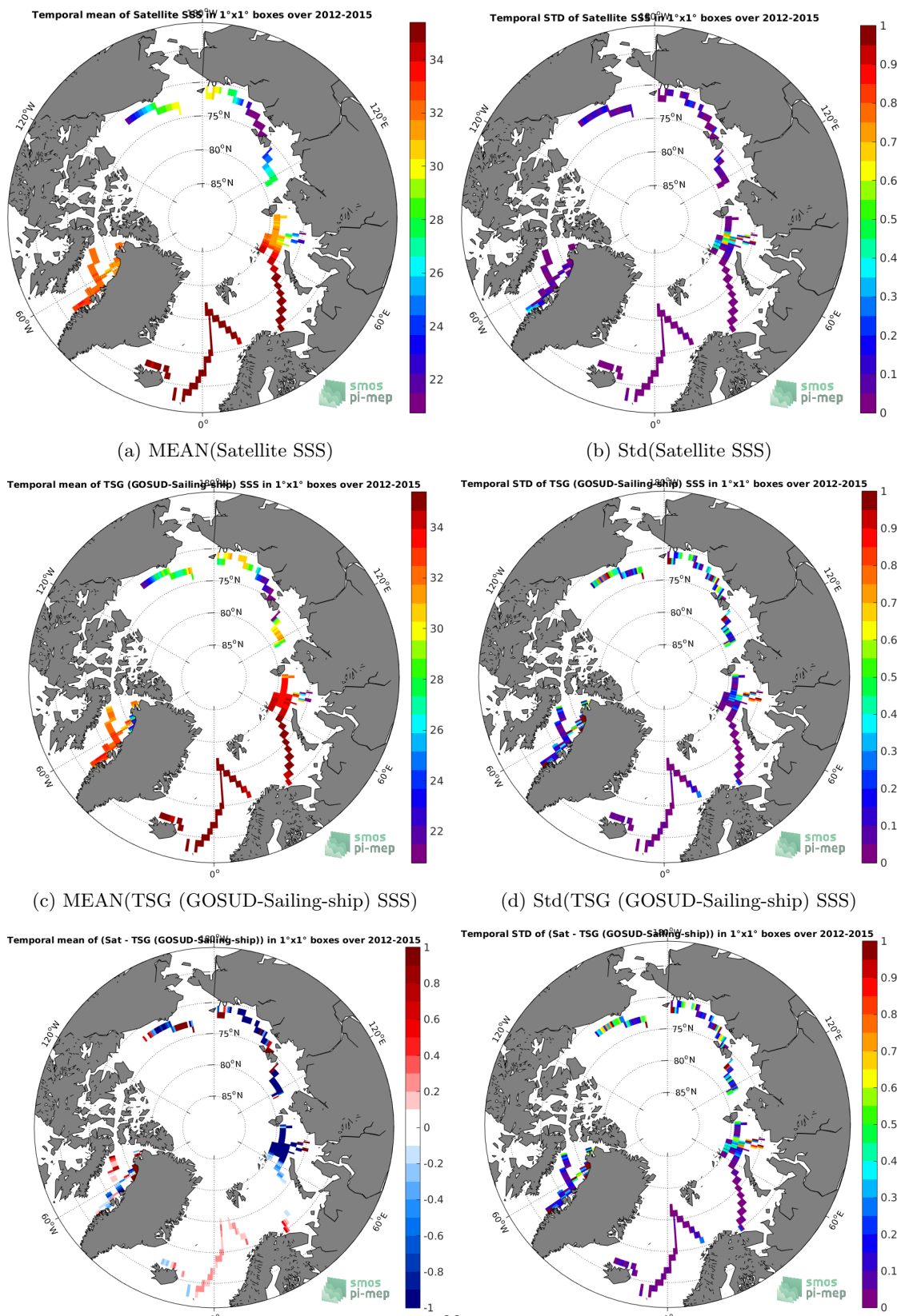
(e) MEAN( \Delta SSS (Satellite - TSG (GOSUD-Sailing-ship)))
