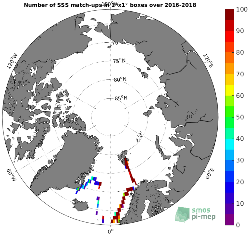
Figure 4: Number of SSS match-ups between TSG (GOSUD-Research-vessel) SSS and the SMAP SSS L4 OI v1 - Monthly (IPRC) SSS product for the Arctic Ocean Pi-MEP region over 1^\circ \times 1^\circ boxes and for the full satellite product period.
