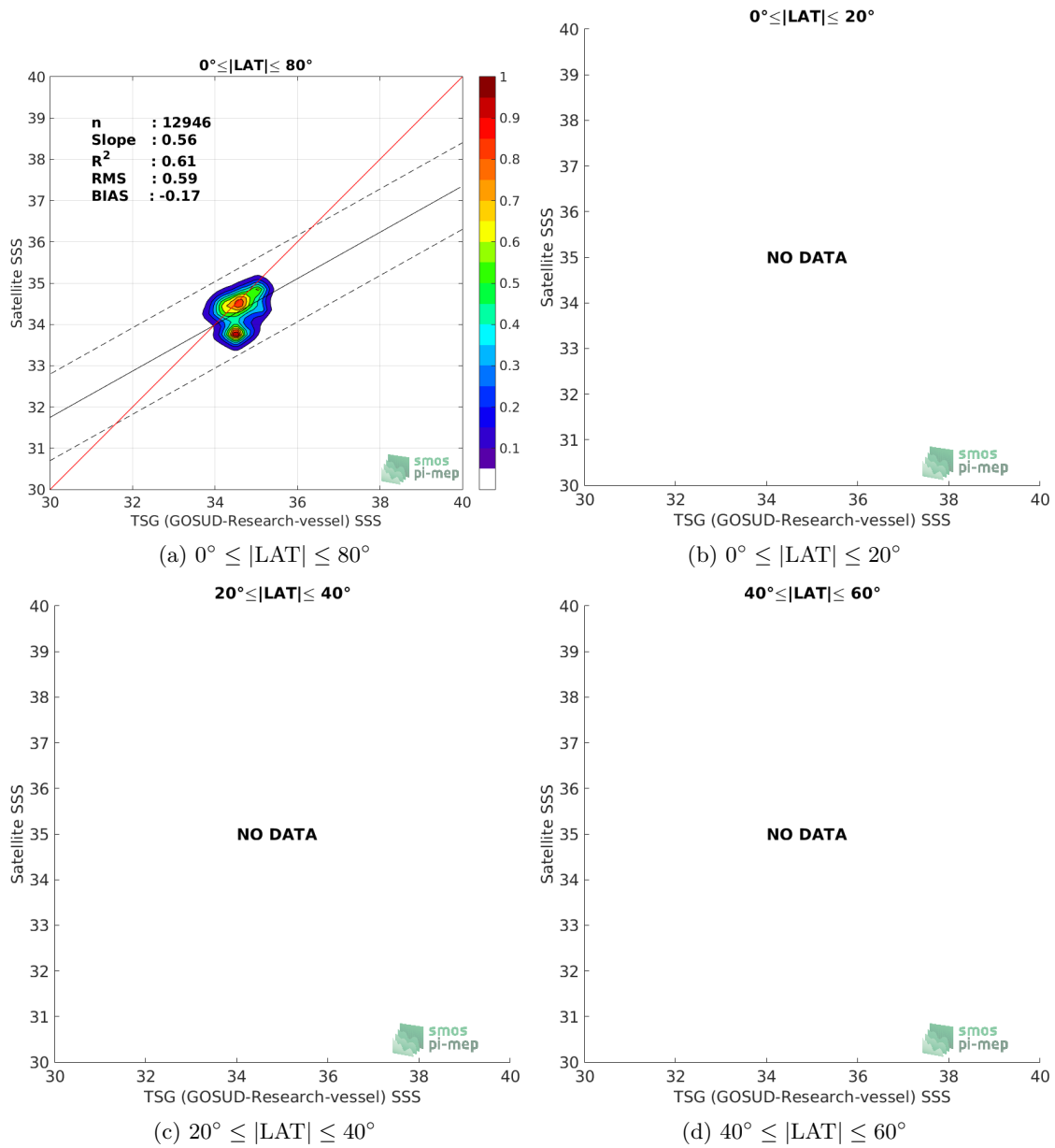
Figure 9: Contour maps of the concentration of SMAP SSS L4 OI v1 - Monthly (IPRC) SSS (y-axis) versus TSG (GOSUD-Research-vessel) SSS (x-axis) at match-up pairs for different latitude bands. For each plot, the red line shows x=y . The black thin and dashed lines indicate a linear fit through the data cloud and the \pm 95\% confidence levels, respectively. The number match-up pairs n , the slope and R^2 coefficient of the linear fit, the root mean square (RMS) and the mean bias between satellite and in situ data are indicated for each latitude band in each plots.
