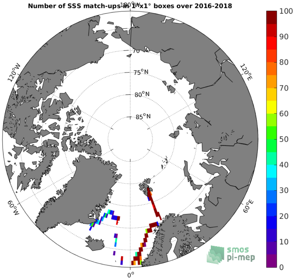
Figure 4: Number of SSS match-ups between TSG (GOSUD-Research-vessel) SSS and the SMAP SSS L4 OI v1 - Monthly (IPRC) SSS product for the Arctic Ocean Pi-MEP region over 1°x1° boxes and for the full satellite product period.
