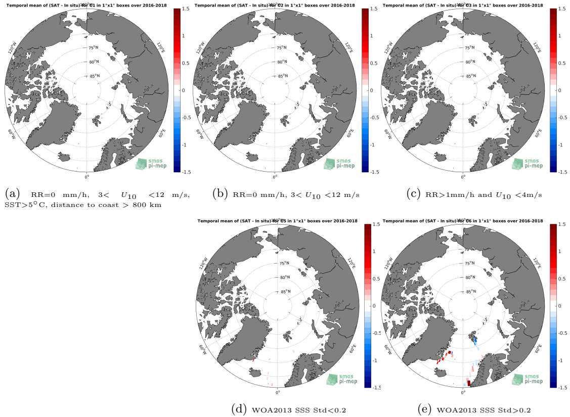
Figure 12: Temporal mean gridded over spatial boxes of size 1°x1° of \Delta SSS (SMAP SSS L4 OI v1 - Monthly (IPRC) - TSG (GOSUD-Research-vessel)) for 5 different subdatasets corresponding to:RR=0 mm/h, 3 < U_{10} < 12 m/s, SST>5°C, distance to coast > 800 km (a), RR=0 mm/h, 3 < U_{10} < 12 m/s (b), RR>1mm/h and U_{10} < 4 m/s (c), WOA2013 SSS Std<0.2 (d), WOA2013 SSS Std>0.2 (e).
