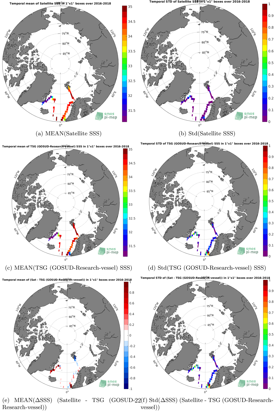
Figure 6: Temporal mean (left) and Std (right) of SSS from SMAP SSS L4 OI v1 - Monthly (IPRC) (top), TSG (GOSUD-Research-vessel) (middle), and of \Delta SSS (Satellite - TSG (GOSUD-Research-vessel)). Only match-up pairs are used to generate these maps.
