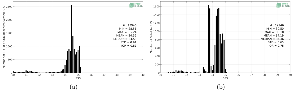
Figure 2: Histograms of SSS from TSG (GOSUD-Research-vessel) (a) and SMAP SSS L4 OI v1 - Monthly (IPRC) (b) considering all match-up pairs per bins of 0.1 over the Arctic Ocean Pi-MEP region and for the full satellite product period.
