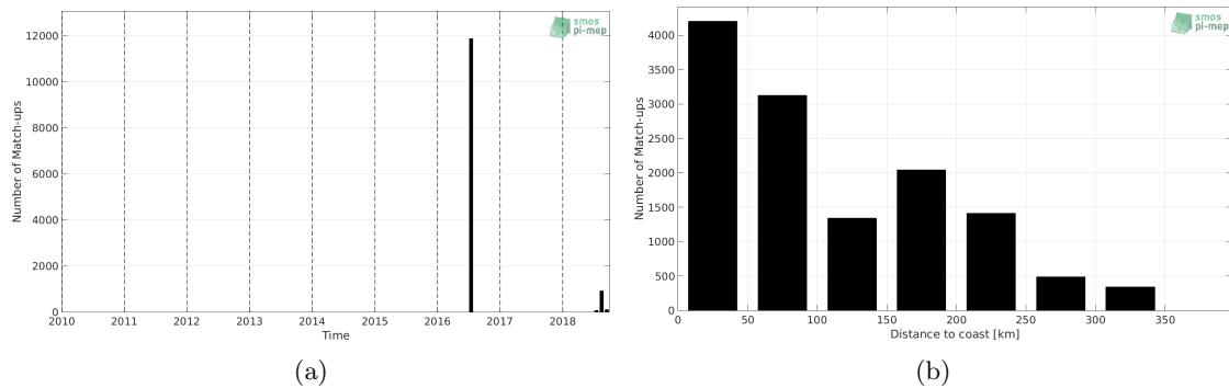
Figure 1: Number of match-ups between TSG (GOSUD-Research-vessel) and SMAP SSS L4 OI v1 - Monthly (IPRC) SSS as a function of time (a) and as function of the distance to coast (b) over the Arctic Ocean Pi-MEP region and for the full satellite product period.
