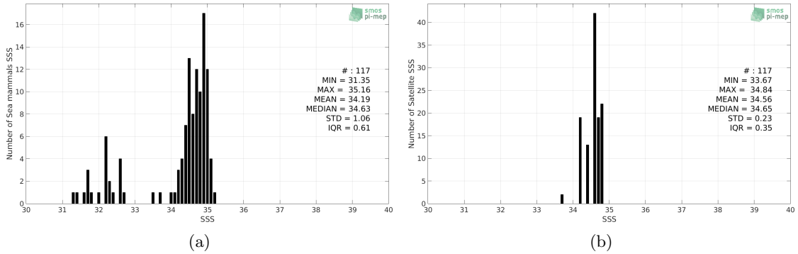
Figure 2: Histograms of SSS from Sea mammals (a) and SMAP SSS L4 OI v1 - Monthly (IPRC) (b) considering all match-up pairs per bins of 0.1 over the Arctic Ocean Pi-MEP region and for the full satellite product period.
