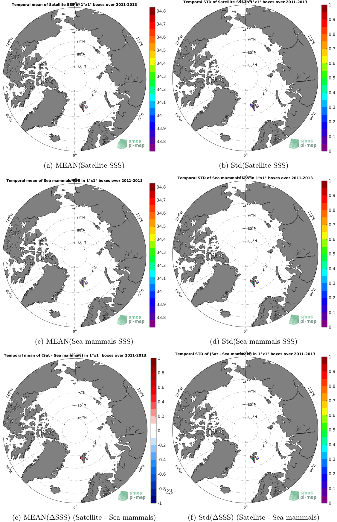
Figure 6: Temporal mean (left) and Std (right) of SSS from SMAP SSS L4 OI v1 - Monthly (IPRC) (top), Sea mammals (middle), and of \Delta SSS (Satellite - Sea mammals). Only match-up pairs are used to generate these maps.
