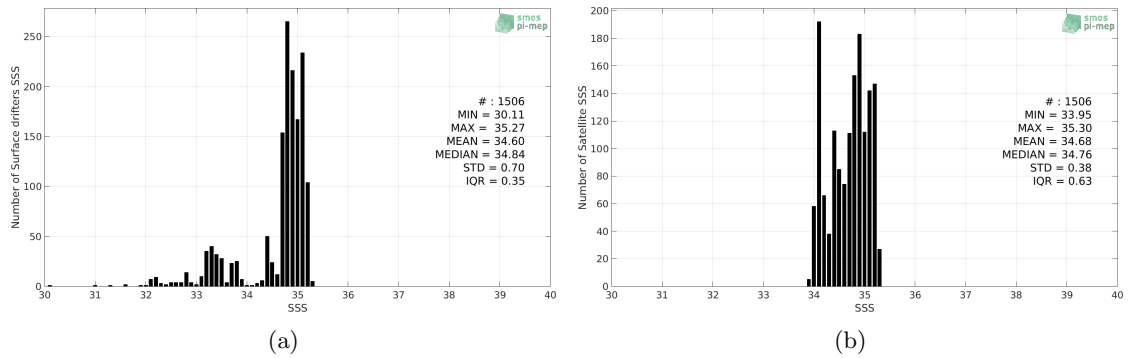
Figure 2: Histograms of SSS from Surface drifters (a) and SMAP SSS L4 OI v1 - Monthly (IPRC) (b) considering all match-up pairs per bins of 0.1 over the Arctic Ocean Pi-MEP region and for the full satellite product period.
