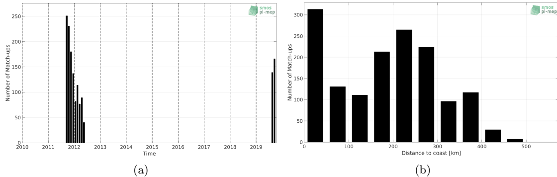
Figure 1: Number of match-ups between Surface drifters and SMAP SSS L4 OI v1 - Monthly (IPRC) SSS as a function of time (a) and as function of the distance to coast (b) over the Arctic Ocean Pi-MEP region and for the full satellite product period.
