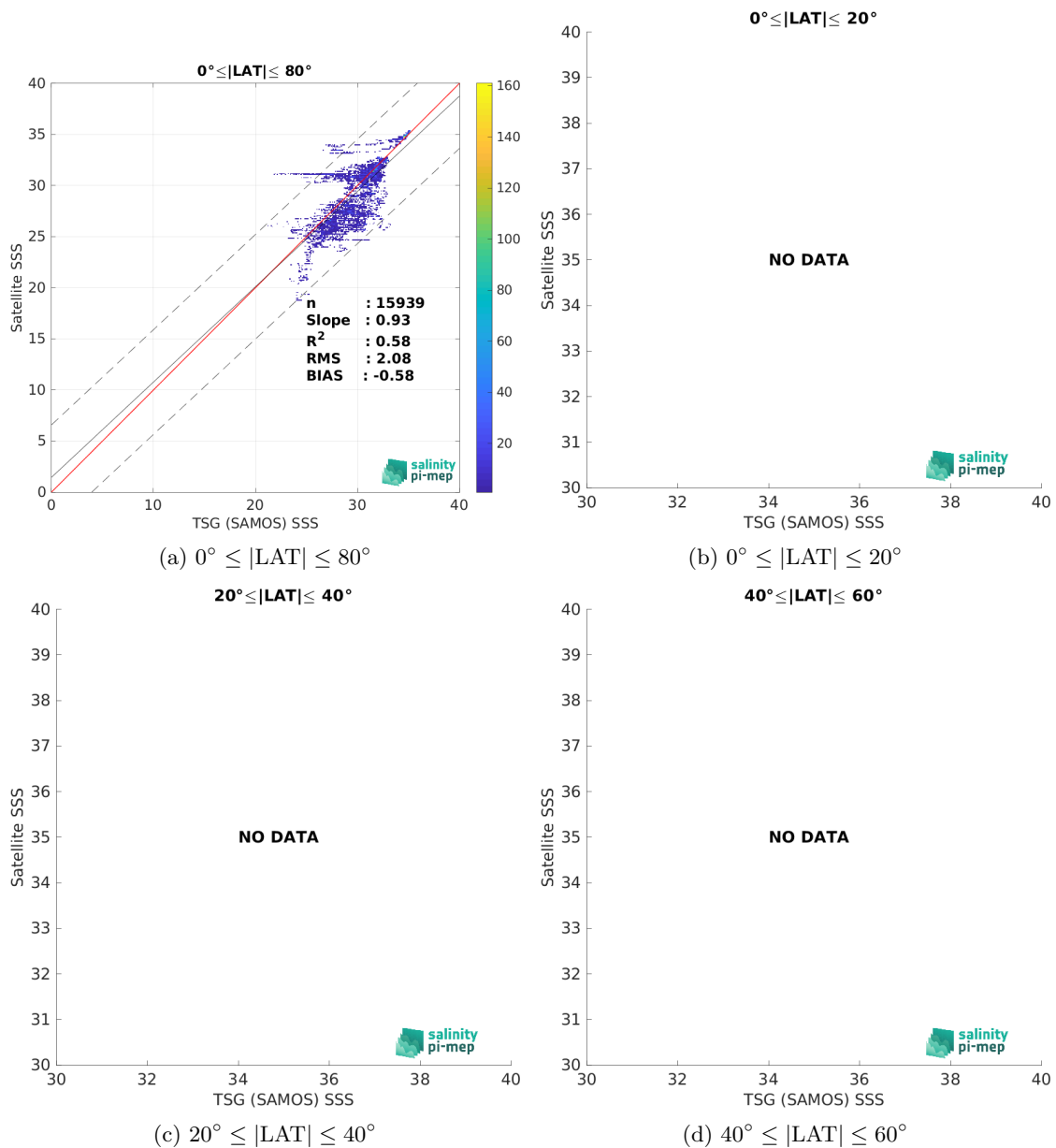
Figure 10: Contour maps of the concentration of SMAP SSS L4 OI v3 - Monthly (ESR) SSS (y-axis) versus TSG (SAMOS) SSS (x-axis) at match-up pairs for different latitude bands. For each plot, the red line shows x=y . The black thin and dashed lines indicate a linear fit through the data cloud and the \pm 95\% confidence levels, respectively. The number match-up pairs n , the slope and R^2 coefficient of the linear fit, the root mean square (RMS) and the mean bias between satellite and in situ data are indicated for each latitude band in each plots.
