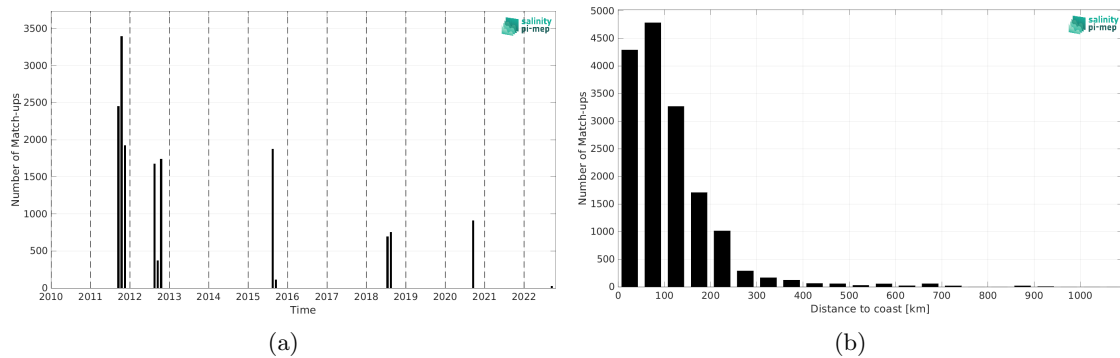
Figure 2: Number of match-ups between TSG (SAMOS) and SMAP SSS L4 OI v3 - Monthly (ESR) SSS as a function of time (a) and as function of the distance to coast (b) over the Arctic Ocean Pi-MEP region and for the full satellite product period.
