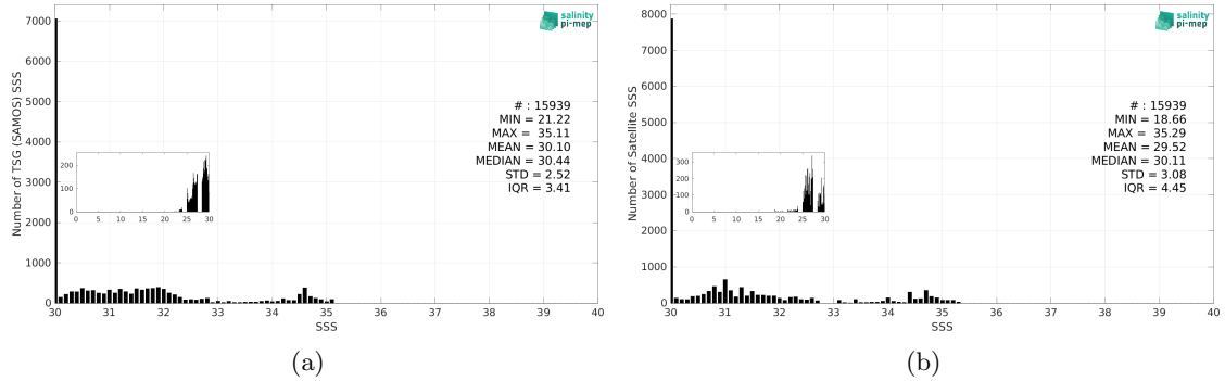
Figure 3: Histograms of SSS from TSG (SAMOS) (a) and SMAP SSS L4 OI v3 - Monthly (ESR) (b) considering all match-up pairs per bins of 0.1 over the Arctic Ocean Pi-MEP region and for the full satellite product period.
