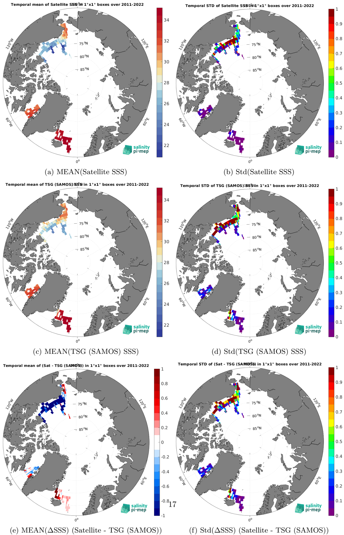
Figure 7: Temporal mean (left) and Std (right) of SSS from SMAP SSS L4 OI v3 - Monthly (ESR) (top), TSG (SAMOS) (middle), and of \Delta SSS (Satellite - TSG (SAMOS)). Only match-up pairs are used to generate these maps.
