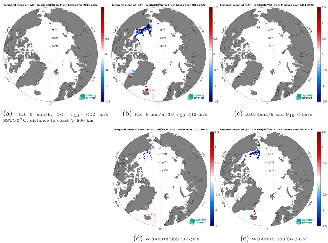
Figure 14: Temporal mean gridded over spatial boxes of size 1^\circ \times 1^\circ of \Delta SSS (SMAP SSS L4 OI v3 - Monthly (ESR) - TSG (SAMOS)) for 5 different subdatasets corresponding to:RR=0 mm/h, 3 < U_{10} < 12 m/s, SST > 5^\circ\text{C} , distance to coast > 800 km (a), RR=0 mm/h, 3 < U_{10} < 12 m/s (b), RR > 1 mm/h and U_{10} < 4 m/s (c), WOA2013 SSS Std < 0.2 (d), WOA2013 SSS Std > 0.2 (e).
