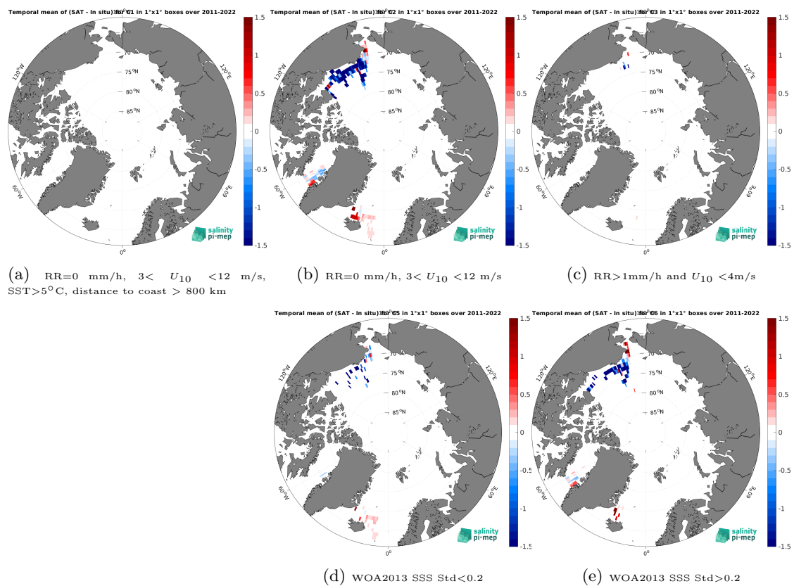
Figure 14: Temporal mean gridded over spatial boxes of size 1^\circ \times 1^\circ of \Delta\text{SSS} (SMAP SSS L4 OI v3 - Monthly (ESR) - TSG (SAMOS)) for 5 different subdatasets corresponding to:RR=0 mm/h, 3 < U_{10} < 12 m/s, SST > 5^\circ\text{C} , distance to coast > 800 km (a), RR=0 mm/h, 3 < U_{10} < 12 m/s (b), RR > 1 mm/h and U_{10} < 4 m/s (c), WOA2013 SSS Std < 0.2 (d), WOA2013 SSS Std > 0.2 (e).
