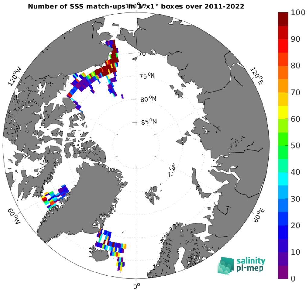
Figure 5: Number of SSS match-ups between TSG (SAMOS) SSS and the SMAP SSS L4 OI v3 - Monthly (ESR) SSS product for the Arctic Ocean Pi-MEP region over 1^\circ \times 1^\circ boxes and for the full satellite product period.
