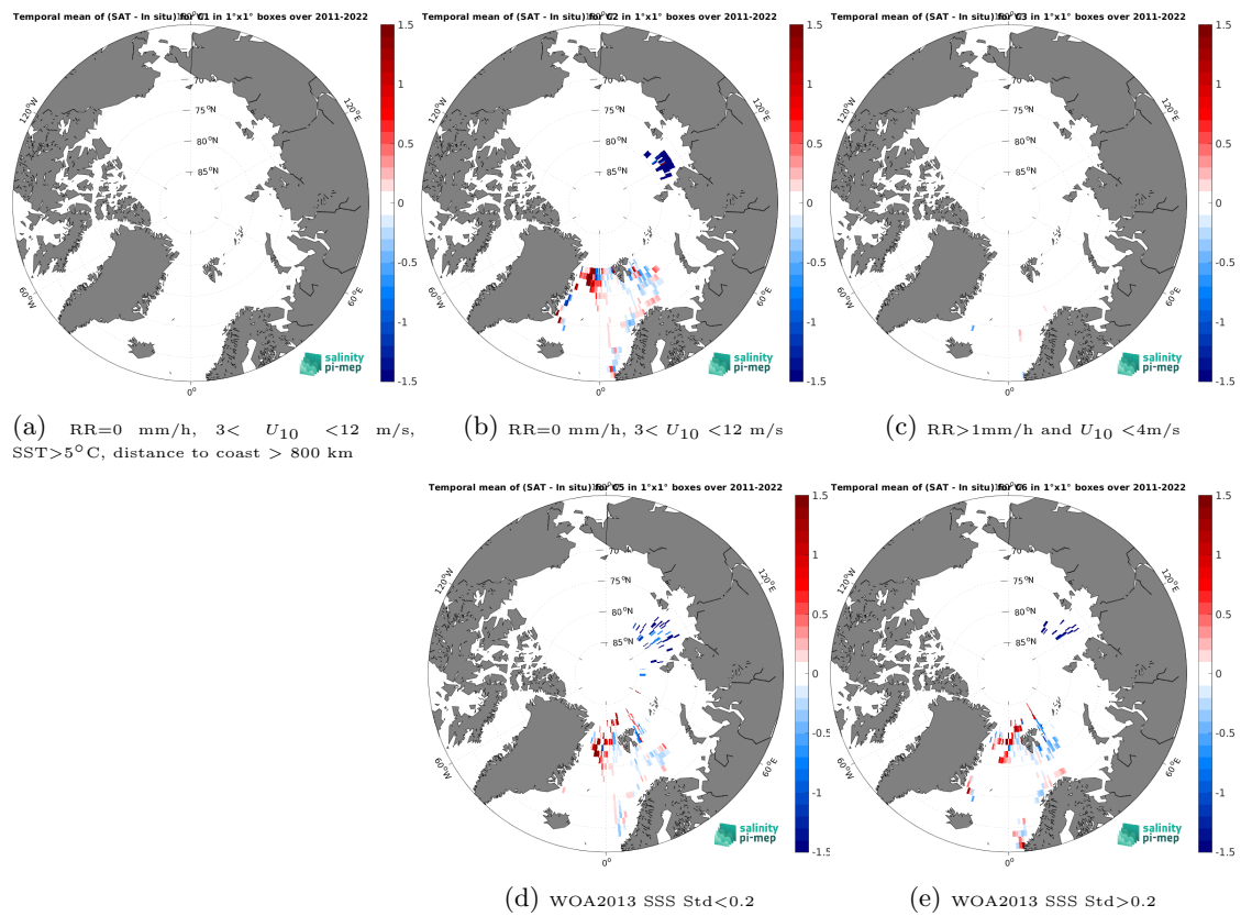
Figure 14: Temporal mean gridded over spatial boxes of size 1^\circ \times 1^\circ of \Delta SSS (SMAP SSS L4 OI v3 - Monthly (ESR) - TSG (Polarstern)) for 5 different subdatasets corresponding to:RR=0 mm/h, 3 < U_{10} < 12 m/s, SST > 5^\circ\text{C} , distance to coast > 800 km (a), RR=0 mm/h, 3 < U_{10} < 12 m/s (b), RR > 1 mm/h and U_{10} < 4 m/s (c), WOA2013 SSS Std < 0.2 (d), WOA2013 SSS Std > 0.2 (e).
