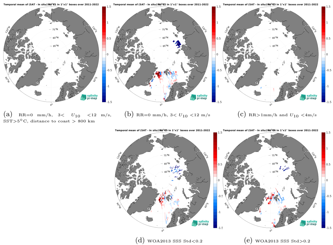
Figure 14: Temporal mean gridded over spatial boxes of size 1^\circ \times 1^\circ of \Delta\text{SSS} (SMAP SSS L4 OI v3 - Monthly (ESR) - TSG (Polarstern)) for 5 different subdatasets corresponding to:RR=0 mm/h, 3 < U_{10} < 12 m/s, SST >5^\circ\text{C} , distance to coast > 800 km (a), RR=0 mm/h, 3 < U_{10} < 12 m/s (b), RR >1 mm/h and U_{10} < 4 m/s (c), WOA2013 SSS Std <0.2 (d), WOA2013 SSS Std >0.2 (e).
