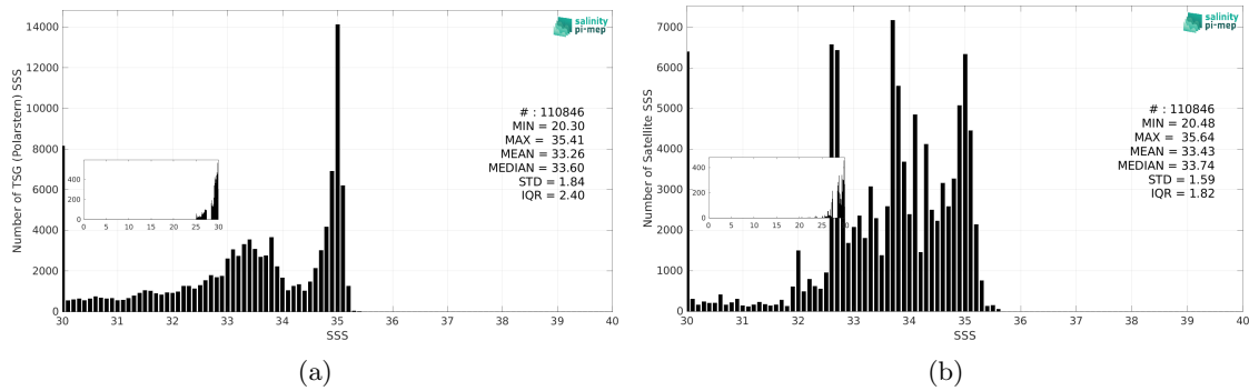
Figure 3: Histograms of SSS from TSG (Polarstern) (a) and SMAP SSS L4 OI v3 - Monthly (ESR) (b) considering all match-up pairs per bins of 0.1 over the Arctic Ocean Pi-MEP region and for the full satellite product period.
