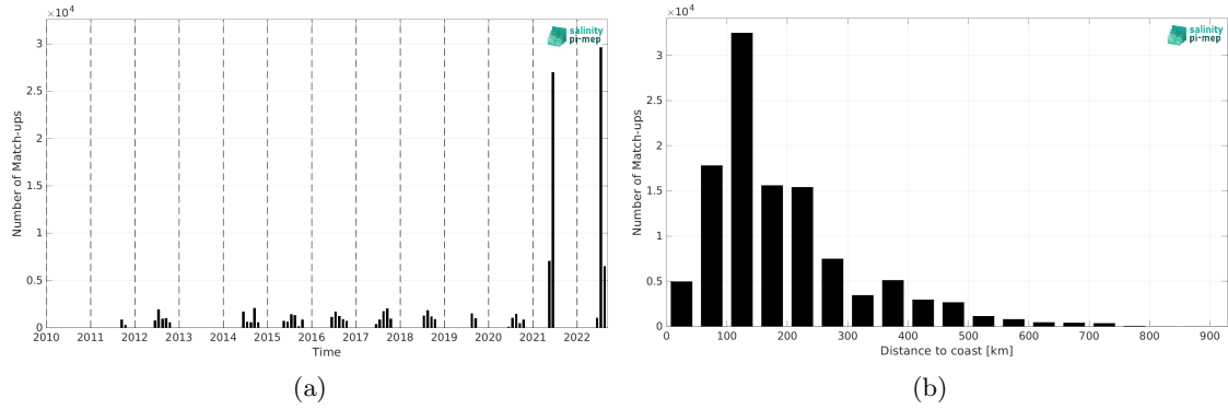
Figure 2: Number of match-ups between TSG (Polarstern) and SMAP SSS L4 OI v3 - Monthly (ESR) SSS as a function of time (a) and as function of the distance to coast (b) over the Arctic Ocean Pi-MEP region and for the full satellite product period.
