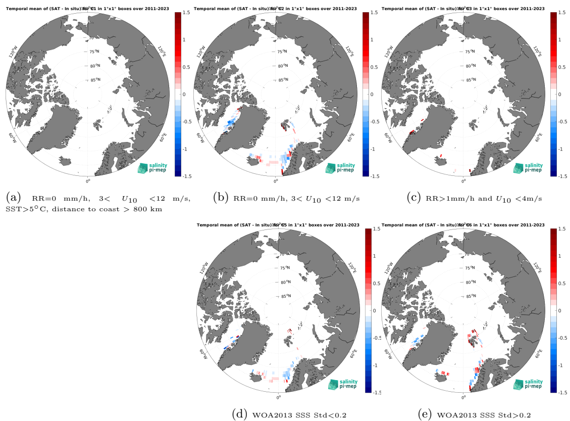
Figure 14: Temporal mean gridded over spatial boxes of size 1^\circ \times 1^\circ of \Delta SSS (SMAP SSS L4 OI v3 - Monthly (ESR) - TSG (LEGOS-DM)) for 5 different subdatasets corresponding to:RR=0 mm/h, 3 < U_{10} < 12 m/s, SST > 5^\circ\text{C} , distance to coast > 800 km (a), RR=0 mm/h, 3 < U_{10} < 12 m/s (b), RR > 1 mm/h and U_{10} < 4 m/s (c), WOA2013 SSS Std < 0.2 (d), WOA2013 SSS Std > 0.2 (e).
