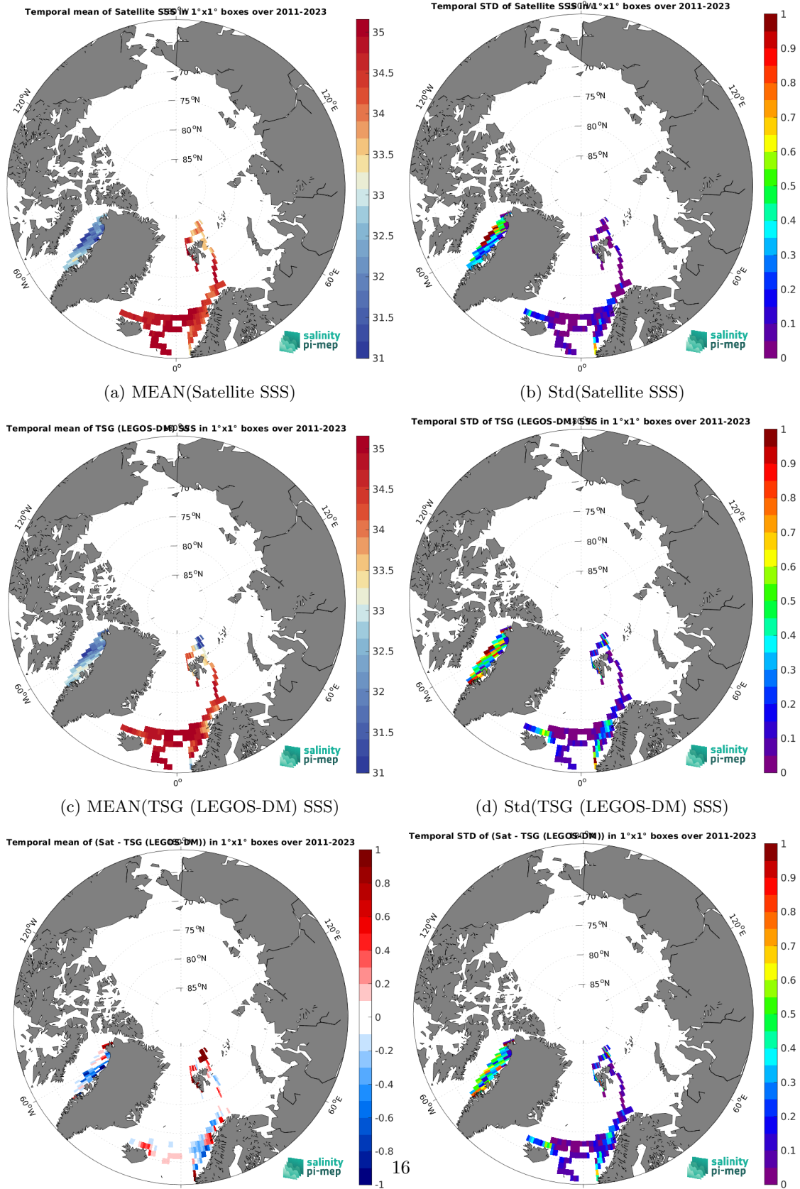
(e) MEAN( \Delta SSS) (Satellite - TSG (LEGOS-DM)) (f) Std( \Delta SSS) (Satellite - TSG (LEGOS-DM)) Figure 7: Temporal mean (left) and Std (right) of SSS from SMAP SSS L4 OI v3 - Monthly (ESR) (top), TSG (LEGOS-DM) (middle), and of \Delta SSS (Satellite - TSG (LEGOS-DM)). Only match-up pairs are used to generate these maps.
