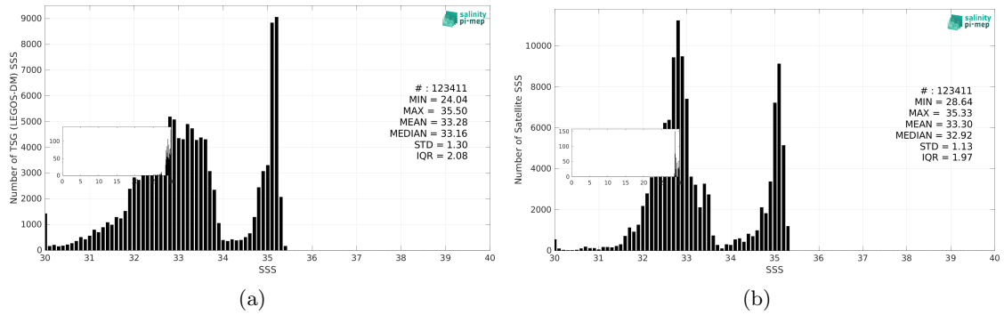
Figure 3: Histograms of SSS from TSG (LEGOS-DM) (a) and SMAP SSS L4 OI v3 - Monthly (ESR) (b) considering all match-up pairs per bins of 0.1 over the Arctic Ocean Pi-MEP region and for the full satellite product period.
