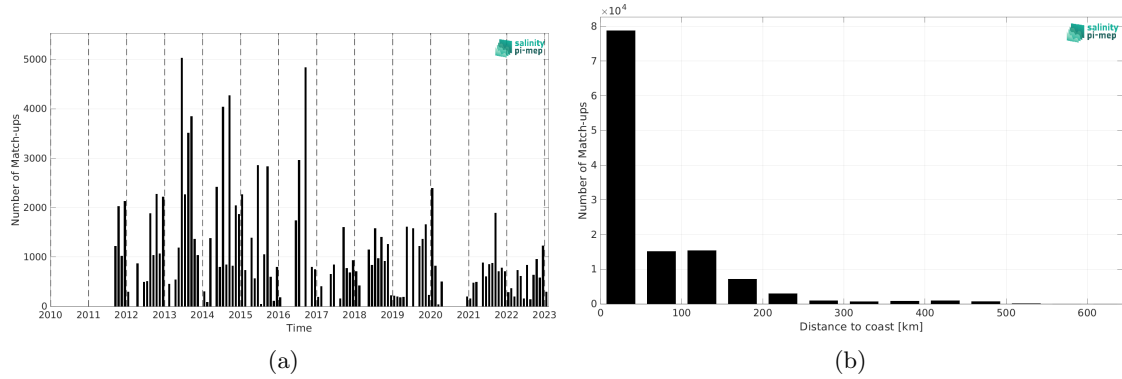
Figure 2: Number of match-ups between TSG (LEGOS-DM) and SMAP SSS L4 OI v3 - Monthly (ESR) SSS as a function of time (a) and as function of the distance to coast (b) over the Arctic Ocean Pi-MEP region and for the full satellite product period.
