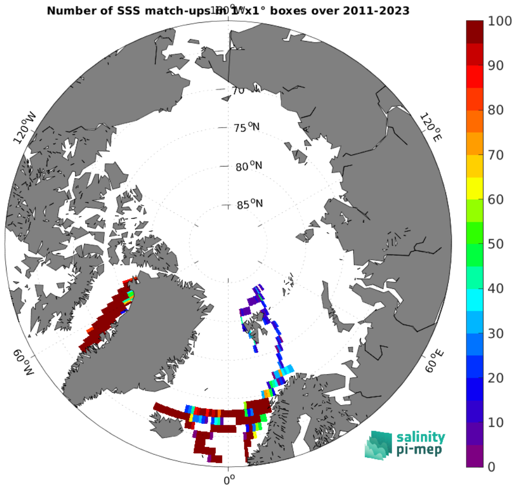
Figure 5: Number of SSS match-ups between TSG (LEGOS-DM) SSS and the SMAP SSS L4 OI v3 - Monthly (ESR) SSS product for the Arctic Ocean Pi-MEP region over 1^\circ \times 1^\circ boxes and for the full satellite product period.
