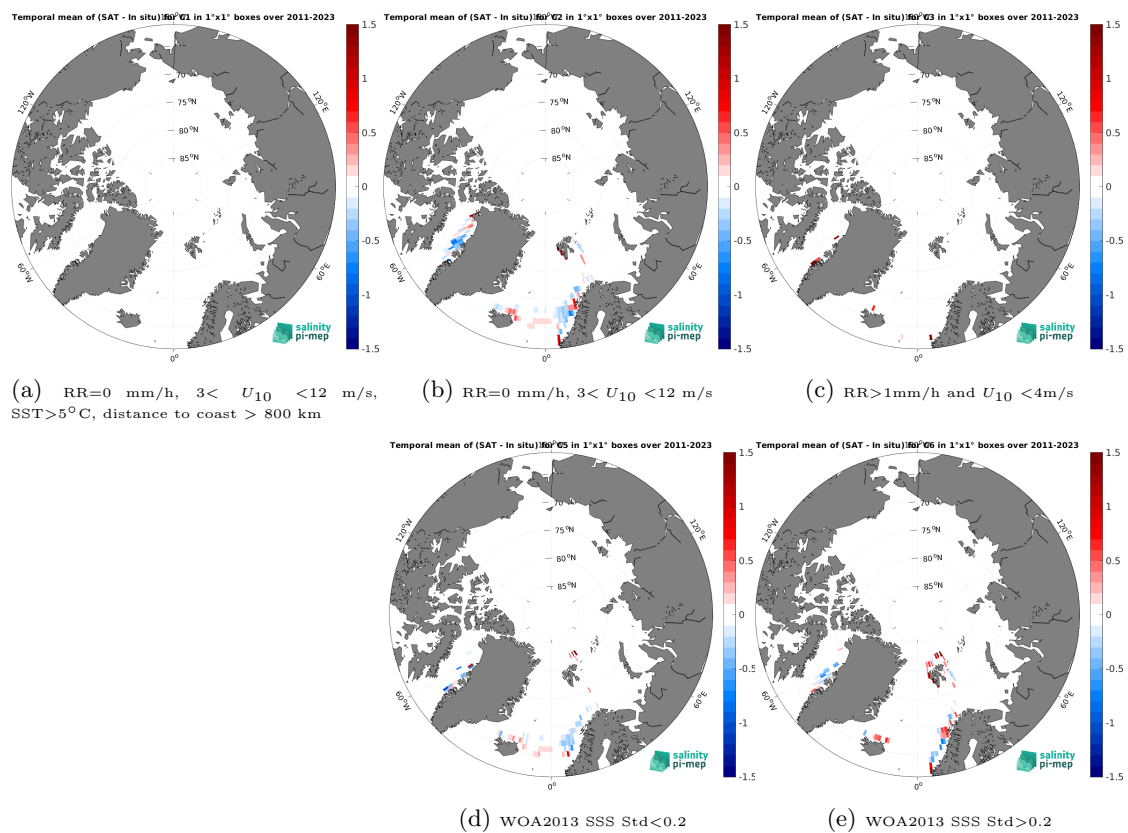
Figure 14: Temporal mean gridded over spatial boxes of size 1^\circ \times 1^\circ of \Delta\text{SSS} (SMAP SSS L4 OI v3 - Monthly (ESR) - TSG (LEGOS-DM)) for 5 different subdatasets corresponding to:RR=0 mm/h, 3 < U_{10} < 12 m/s, SST > 5°C, distance to coast > 800 km (a), RR=0 mm/h, 3 < U_{10} < 12 m/s (b), RR > 1mm/h and U_{10} < 4 m/s (c), WOA2013 SSS Std < 0.2 (d), WOA2013 SSS Std > 0.2 (e).
