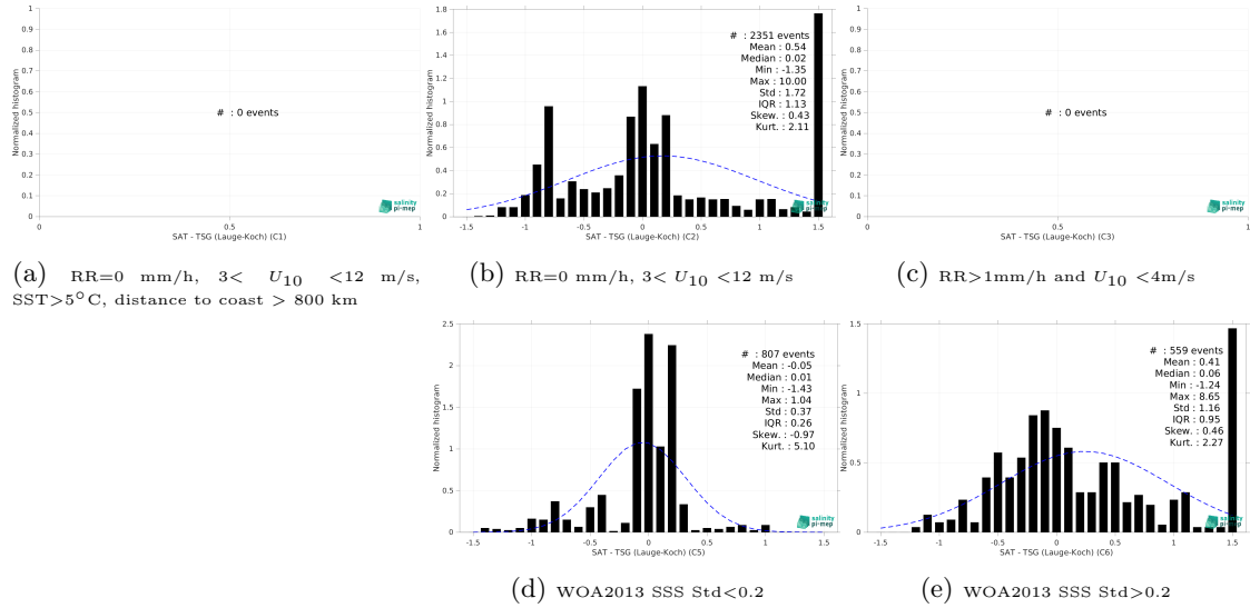
Figure 15: Normalized histogram of \Delta SSS (SMAP SSS L4 OI v3 - Monthly (ESR) - TSG (Lauge-Koch)) for 5 different subdatasets corresponding to: RR=0 mm/h, 3 < U_{10} < 12 m/s, SST > 5°C, distance to coast > 800 km (a), RR=0 mm/h, 3 < U_{10} < 12 m/s (b), RR > 1mm/h and U_{10} < 4 m/s (c), WOA2013 SSS Std < 0.2 (d), WOA2013 SSS Std > 0.2 (e).
