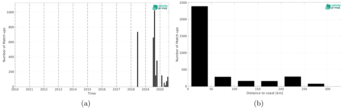
Figure 2: Number of match-ups between TSG (Lauge-Koch) and SMAP SSS L4 OI v3 - Monthly (ESR) SSS as a function of time (a) and as function of the distance to coast (b) over the Arctic Ocean Pi-MEP region and for the full satellite product period.
