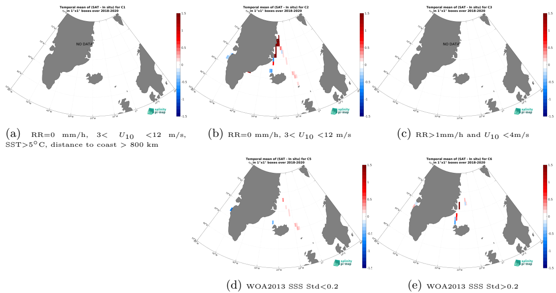
Figure 14: Temporal mean gridded over spatial boxes of size 1^\circ \times 1^\circ of \Delta SSS (SMAP SSS L4 OI v3 - Monthly (ESR) - TSG (Lauge-Koch)) for 5 different subdatasets corresponding to: RR=0 mm/h, 3 < U_{10} < 12 m/s, SST > 5^\circ\text{C} , distance to coast > 800 km (a), RR=0 mm/h, 3 < U_{10} < 12 m/s (b), RR > 1 mm/h and U_{10} < 4 m/s (c), WOA2013 SSS Std < 0.2 (d), WOA2013 SSS Std > 0.2 (e).
