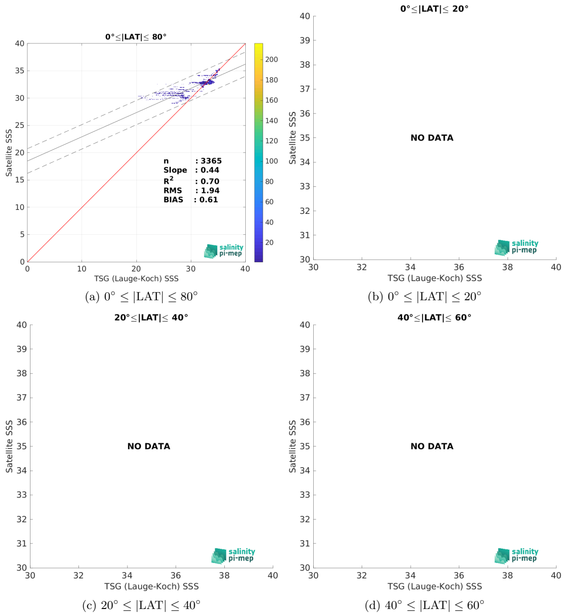
Figure 10: Contour maps of the concentration of SMAP SSS L4 OI v3 - Monthly (ESR) SSS (y-axis) versus TSG (Lauge-Koch) SSS (x-axis) at match-up pairs for different latitude bands. For each plot, the red line shows x=y . The black thin and dashed lines indicate a linear fit through the data cloud and the \pm 95\% confidence levels, respectively. The number match-up pairs n , the slope and R^2 coefficient of the linear fit, the root mean square (RMS) and the mean bias between satellite and in situ data are indicated for each latitude band in each plots.
