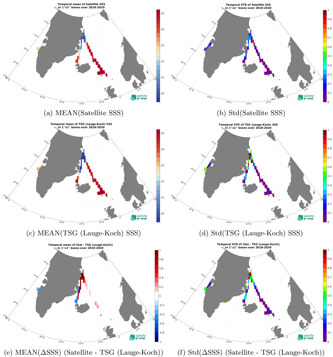
Figure 7: Temporal mean (left) and Std (right) of SSS from SMAP SSS L4 OI v3 - Monthly (ESR) (top), TSG (Lauge-Koch) (middle), and of \Delta SSS (Satellite - TSG (Lauge-Koch)). Only match-up pairs are used to generate these maps.
