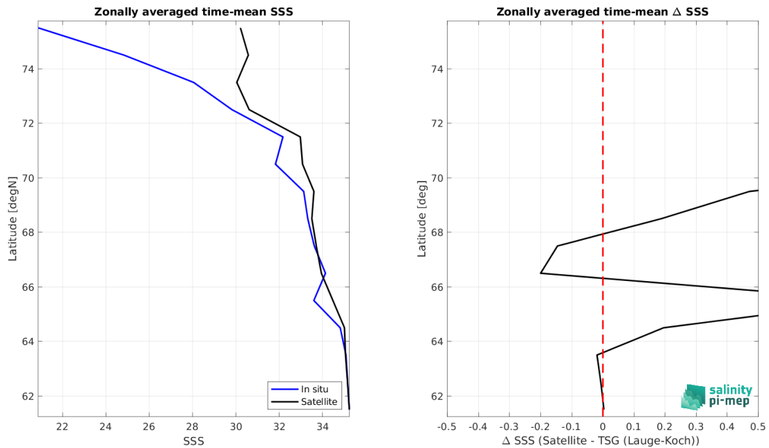
Figure 9: Left panel: Zonal mean SSS from SMAP SSS L4 OI v3 - Monthly (ESR) satellite product (black) and from TSG (Lauge-Koch) (blue). Right panel: Zonal mean of \Delta SSS (Satellite - TSG (Lauge-Koch)) for all the collected Pi-MEP match-up pairs estimated over the full satellite product period.
