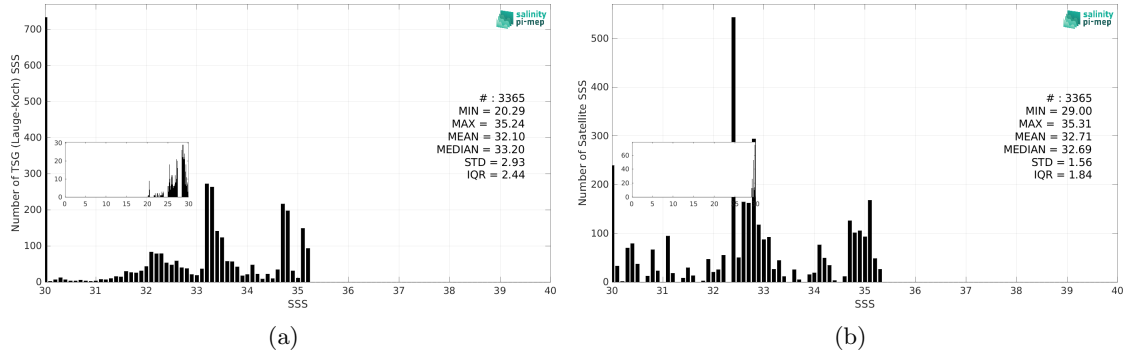
Figure 3: Histograms of SSS from TSG (Lauge-Koch) (a) and SMAP SSS L4 OI v3 - Monthly (ESR) (b) considering all match-up pairs per bins of 0.1 over the Arctic Ocean Pi-MEP region and for the full satellite product period.
