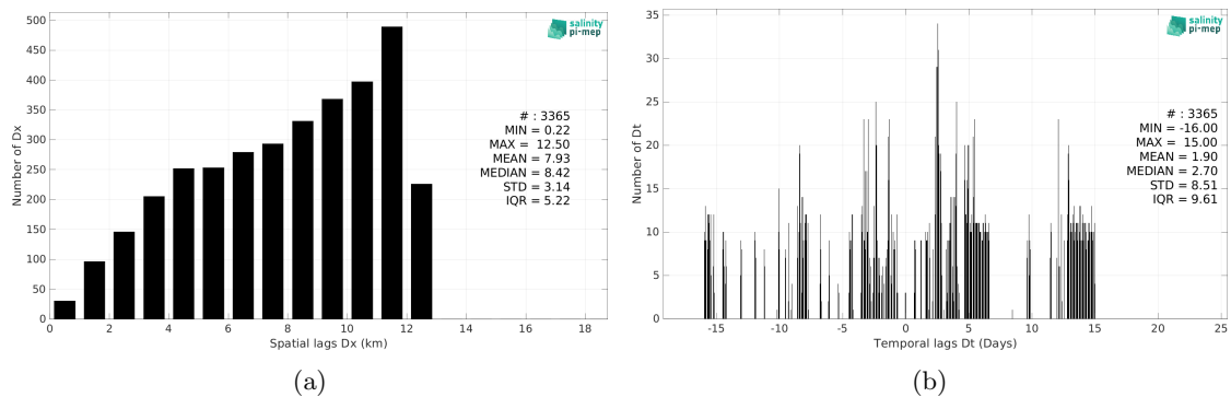
Figure 6: Histograms of the spatial (a) and temporal (b) lags between the location/time of the TSG (Lauge-Koch) measurement and the date of the corresponding SMAP SSS L4 OI v3 - Monthly (ESR) SSS pixel.
