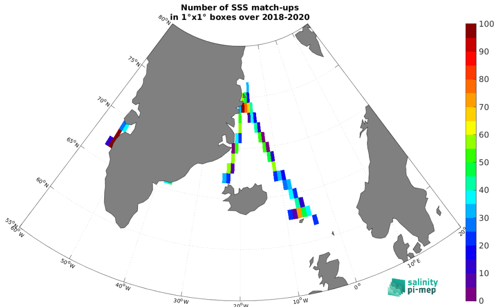
Figure 5: Number of SSS match-ups between TSG (Lauge-Koch) SSS and the SMAP SSS L4 OI v3 - Monthly (ESR) SSS product for the Arctic Ocean Pi-MEP region over 1^\circ \times 1^\circ boxes and for the full satellite product period.
