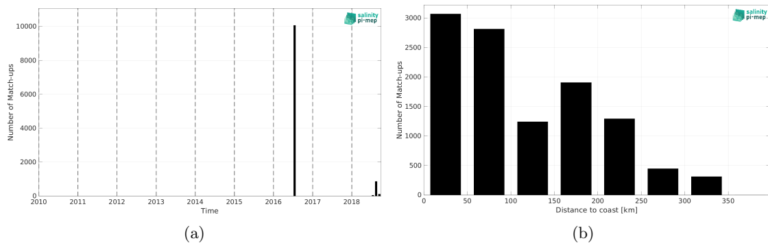
Figure 2: Number of match-ups between TSG (GOSUD-Research-vessel) and SMAP SSS L4 OI v3 - Monthly (ESR) SSS as a function of time (a) and as function of the distance to coast (b) over the Arctic Ocean Pi-MEP region and for the full satellite product period.
