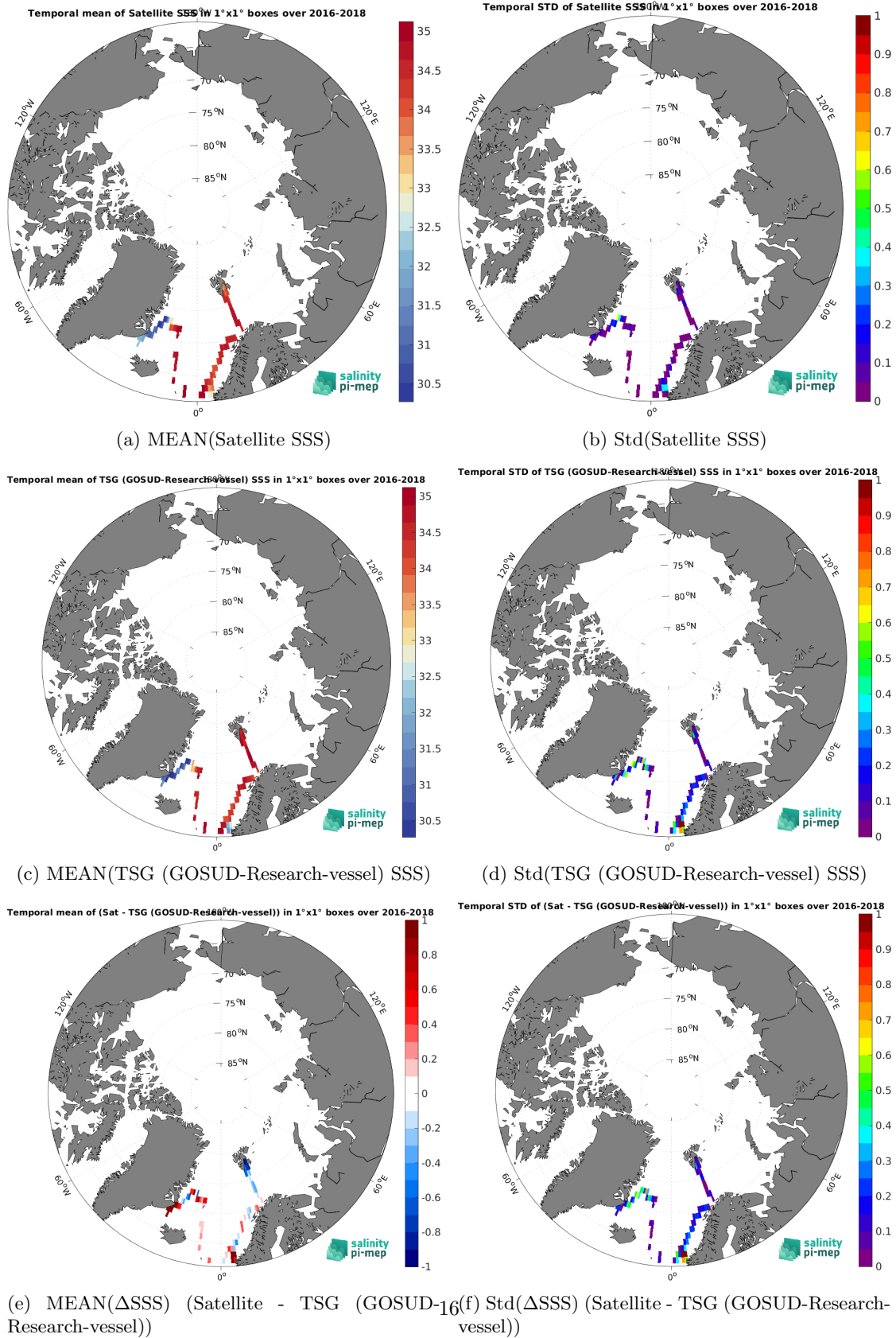
Figure 7: Temporal mean (left) and Std (right) of SSS from SMAP SSS L4 OI v3 - Monthly (ESR) (top), TSG (GOSUD-Research-vessel) (middle), and of \Delta SSS (Satellite - TSG (GOSUD-Research-vessel)). Only match-up pairs are used to generate these maps.
