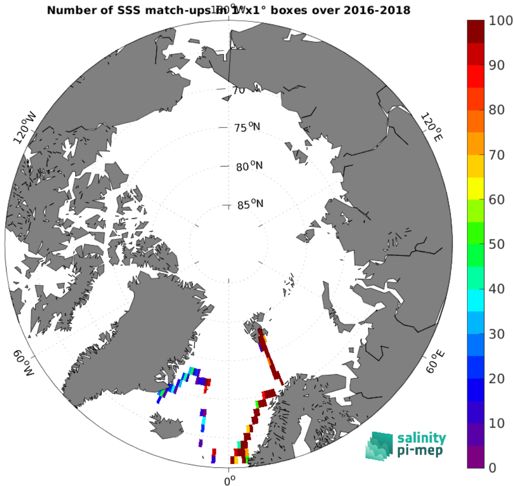
Figure 5: Number of SSS match-ups between TSG (GOSUD-Research-vessel) SSS and the SMAP SSS L4 OI v3 - Monthly (ESR) SSS product for the Arctic Ocean Pi-MEP region over 1^\circ \times 1^\circ boxes and for the full satellite product period.
