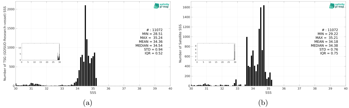
Figure 3: Histograms of SSS from TSG (GOSUD-Research-vessel) (a) and SMAP SSS L4 OI v3 - Monthly (ESR) (b) considering all match-up pairs per bins of 0.1 over the Arctic Ocean Pi-MEP region and for the full satellite product period.
