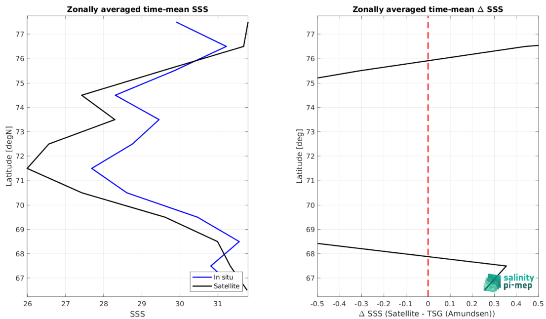
Figure 9: Left panel: Zonal mean SSS from SMAP SSS L4 OI v3 - Monthly (ESR) satellite product (black) and from TSG (Amundsen) (blue). Right panel: Zonal mean of \Delta SSS (Satellite - TSG (Amundsen)) for all the collected Pi-MEP match-up pairs estimated over the full satellite product period.
