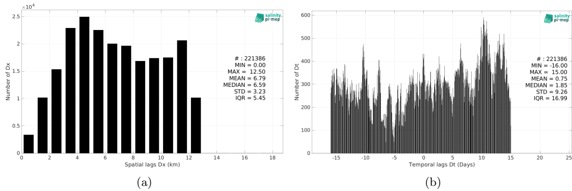
Figure 6: Histograms of the spatial (a) and temporal (b) lags between the location/time of the TSG (Amundsen) measurement and the date of the corresponding SMAP SSS L4 OI v3 - Monthly (ESR) SSS pixel.
