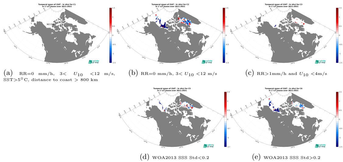
Figure 14: Temporal mean gridded over spatial boxes of size 1^\circ \times 1^\circ of \Delta SSS (SMAP SSS L4 OI v3 - Monthly (ESR) - TSG (Amundsen)) for 5 different subdatasets corresponding to:RR=0 mm/h, 3 < U_{10} < 12 m/s, SST > 5°C, distance to coast > 800 km (a), RR=0 mm/h, 3 < U_{10} < 12 m/s (b), RR > 1mm/h and U_{10} < 4 m/s (c), WOA2013 SSS Std < 0.2 (d), WOA2013 SSS Std > 0.2 (e).
