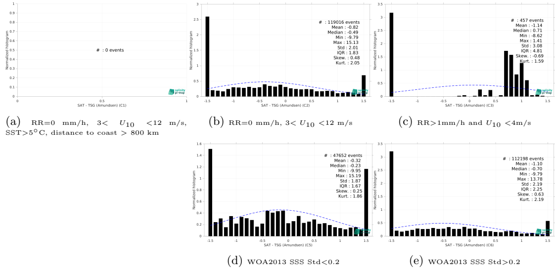
Figure 15: Normalized histogram of \Delta SSS (SMAP SSS L4 OI v3 - Monthly (ESR) - TSG (Amundsen)) for 5 different subdatasets corresponding to: RR=0 mm/h, 3 < U_{10} < 12 m/s, SST > 5°C, distance to coast > 800 km (a), RR=0 mm/h, 3 < U_{10} < 12 m/s (b), RR > 1mm/h and U_{10} < 4 m/s (c), WOA2013 SSS Std < 0.2 (d), WOA2013 SSS Std > 0.2 (e).
