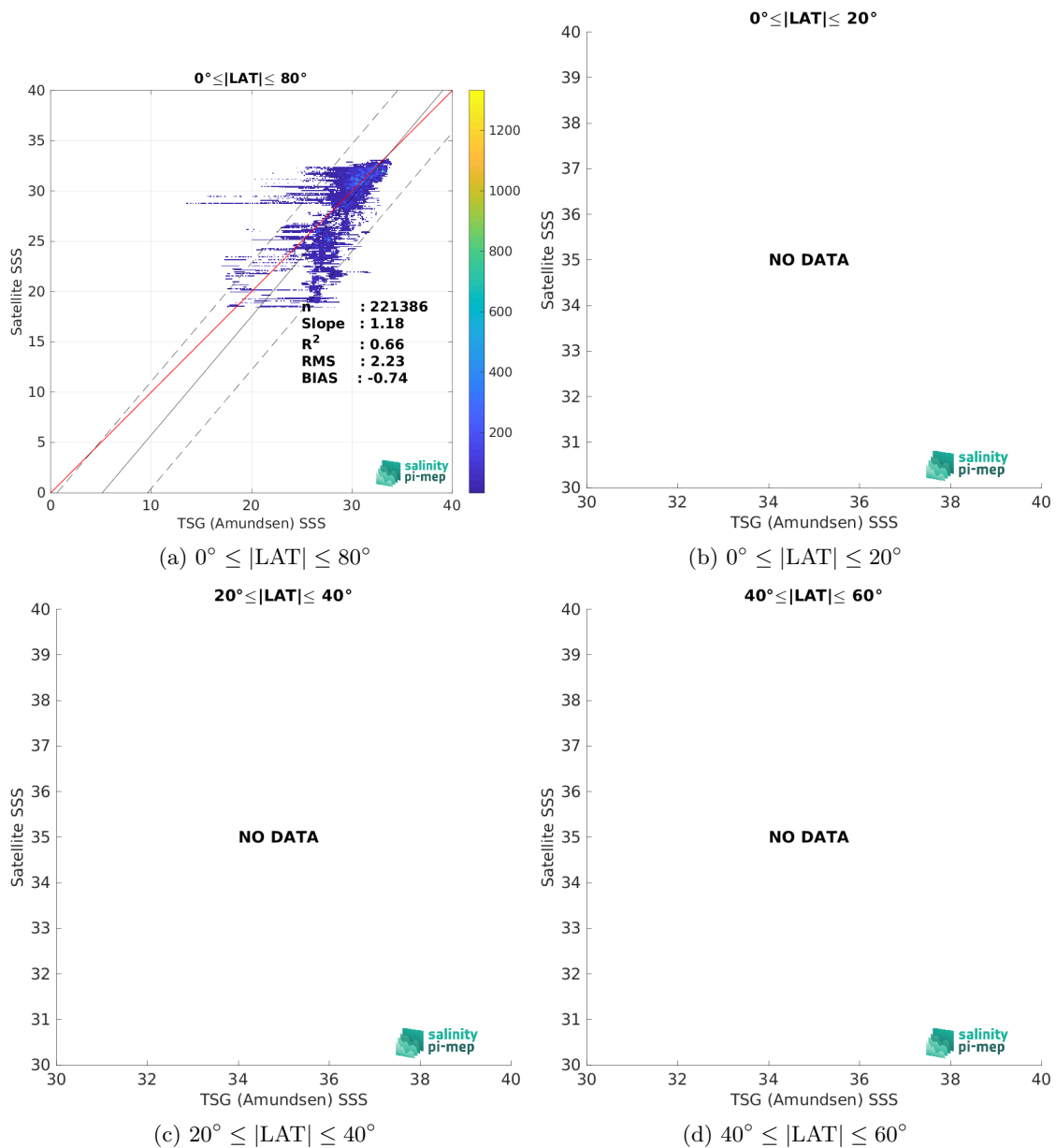
Figure 10: Contour maps of the concentration of SMAP SSS L4 OI v3 - Monthly (ESR) SSS (y-axis) versus TSG (Amundsen) SSS (x-axis) at match-up pairs for different latitude bands. For each plot, the red line shows x=y . The black thin and dashed lines indicate a linear fit through the data cloud and the \pm 95\% confidence levels, respectively. The number match-up pairs n , the slope and R^2 coefficient of the linear fit, the root mean square (RMS) and the mean bias between satellite and in situ data are indicated for each latitude band in each plots.
