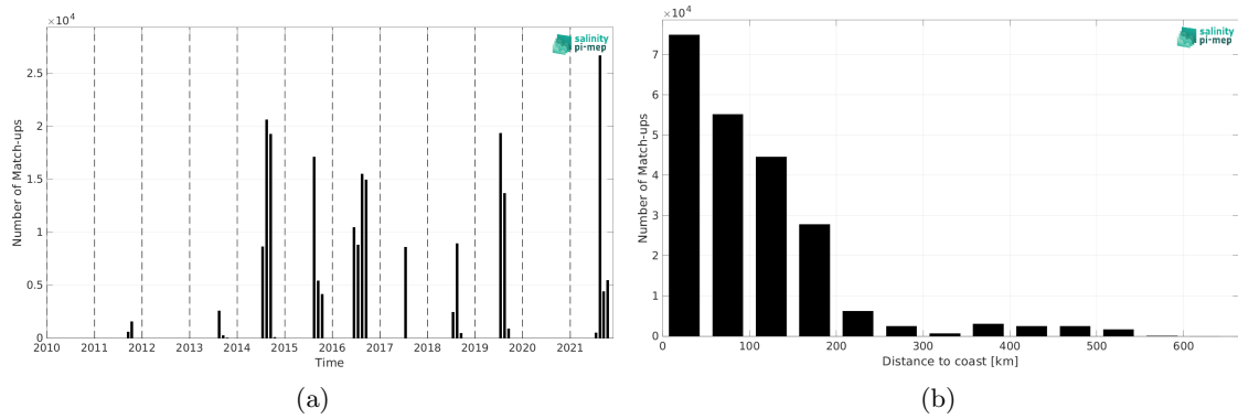
Figure 2: Number of match-ups between TSG (Amundsen) and SMAP SSS L4 OI v3 - Monthly (ESR) SSS as a function of time (a) and as function of the distance to coast (b) over the Arctic Ocean Pi-MEP region and for the full satellite product period.
