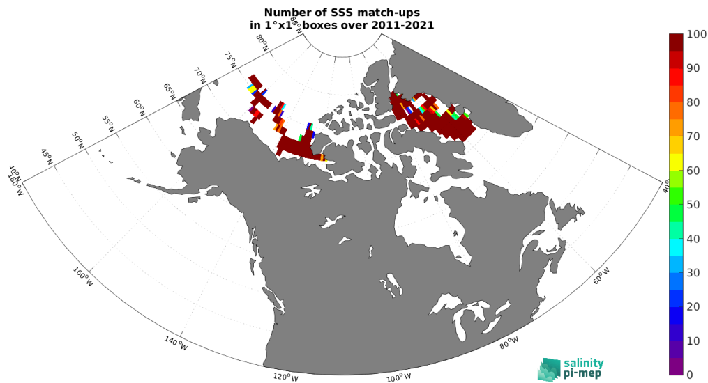
Figure 5: Number of SSS match-ups between TSG (Amundsen) SSS and the SMAP SSS L4 OI v3 - Monthly (ESR) SSS product for the Arctic Ocean Pi-MEP region over 1^\circ \times 1^\circ boxes and for the full satellite product period.
