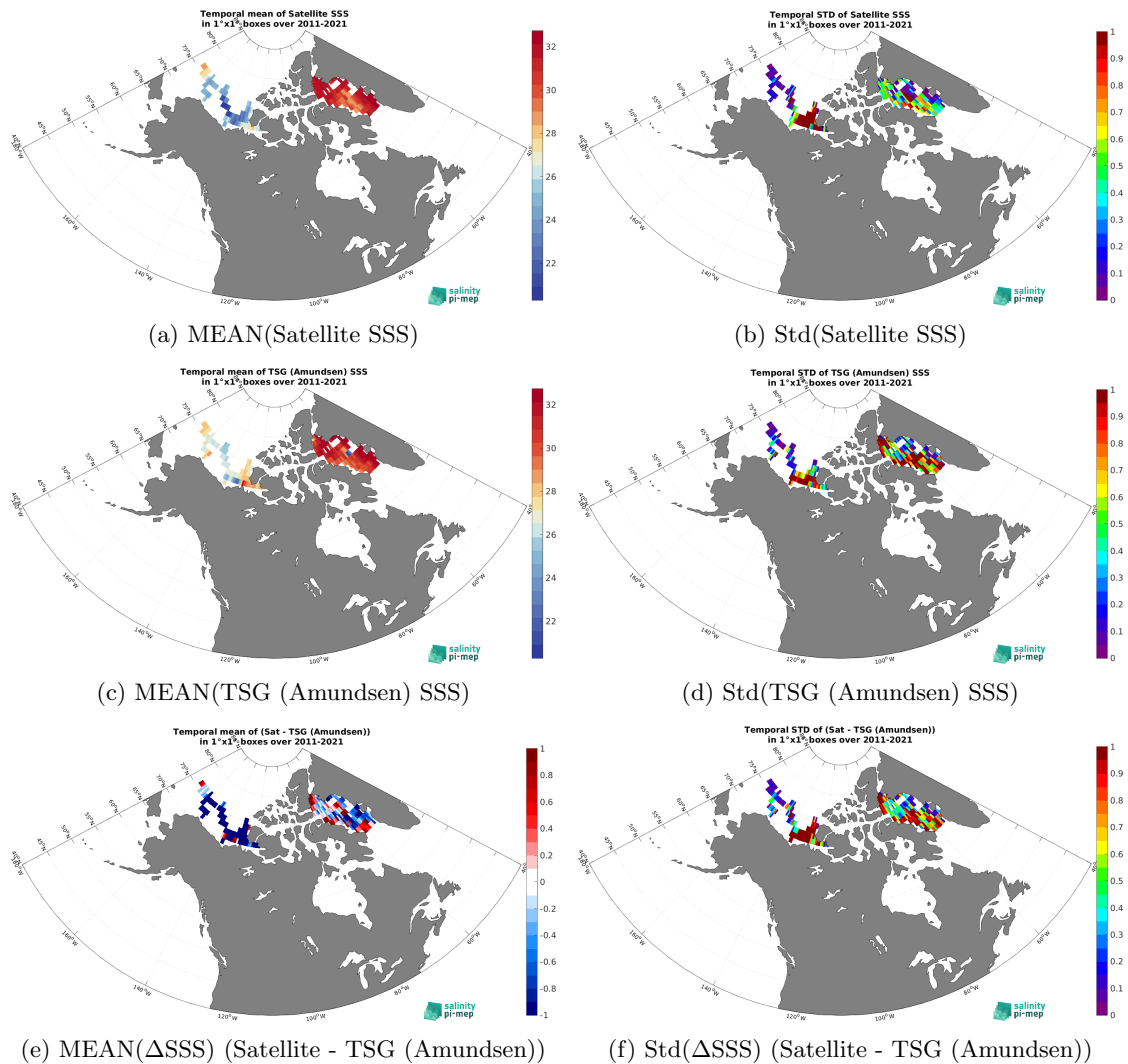
Figure 7: Temporal mean (left) and Std (right) of SSS from SMAP SSS L4 OI v3 - Monthly (ESR) (top), TSG (Amundsen) (middle), and of \Delta SSS (Satellite - TSG (Amundsen)). Only match-up pairs are used to generate these maps.
