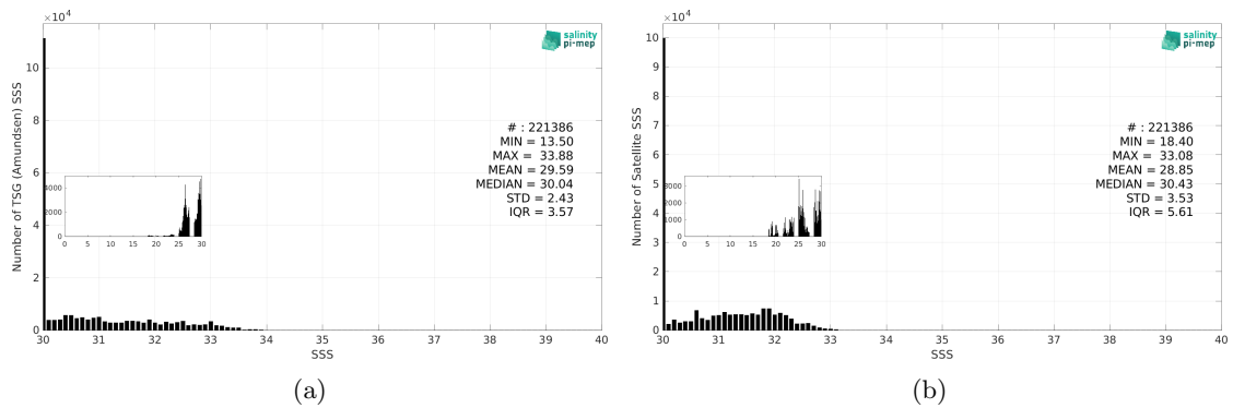
Figure 3: Histograms of SSS from TSG (Amundsen) (a) and SMAP SSS L4 OI v3 - Monthly (ESR) (b) considering all match-up pairs per bins of 0.1 over the Arctic Ocean Pi-MEP region and for the full satellite product period.
