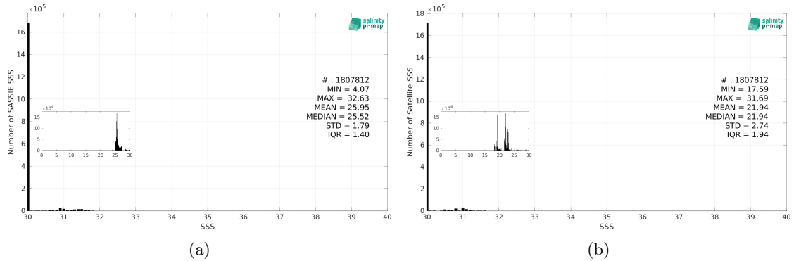
Figure 3: Histograms of SSS from SASSIE (a) and SMAP SSS L4 OI v3 - Monthly (ESR) (b) considering all match-up pairs per bins of 0.1 over the Arctic Ocean Pi-MEP region and for the full satellite product period.
