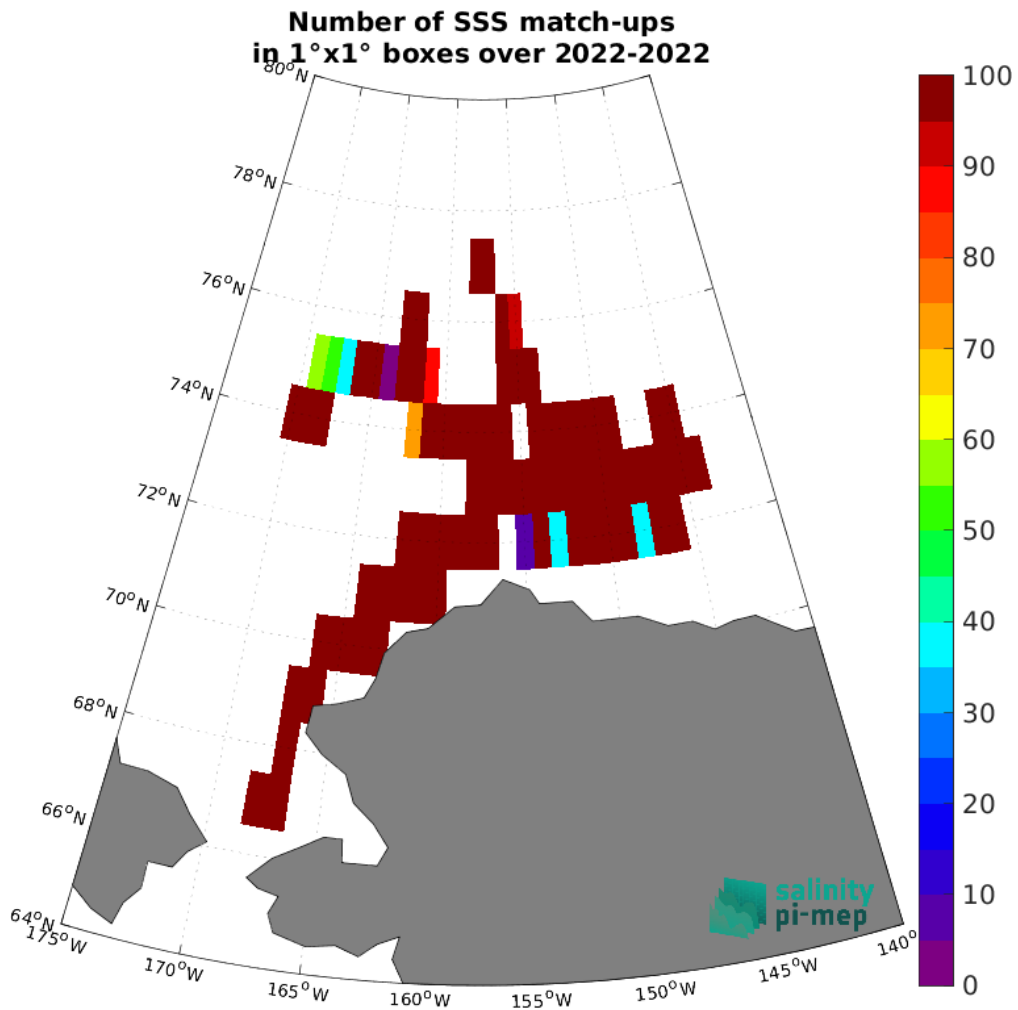
Figure 5: Number of SSS match-ups between SASSIE SSS and the SMAP SSS L4 OI v3 - Monthly (ESR) SSS product for the Arctic Ocean Pi-MEP region over 1^\circ \times 1^\circ boxes and for the full satellite product period.
