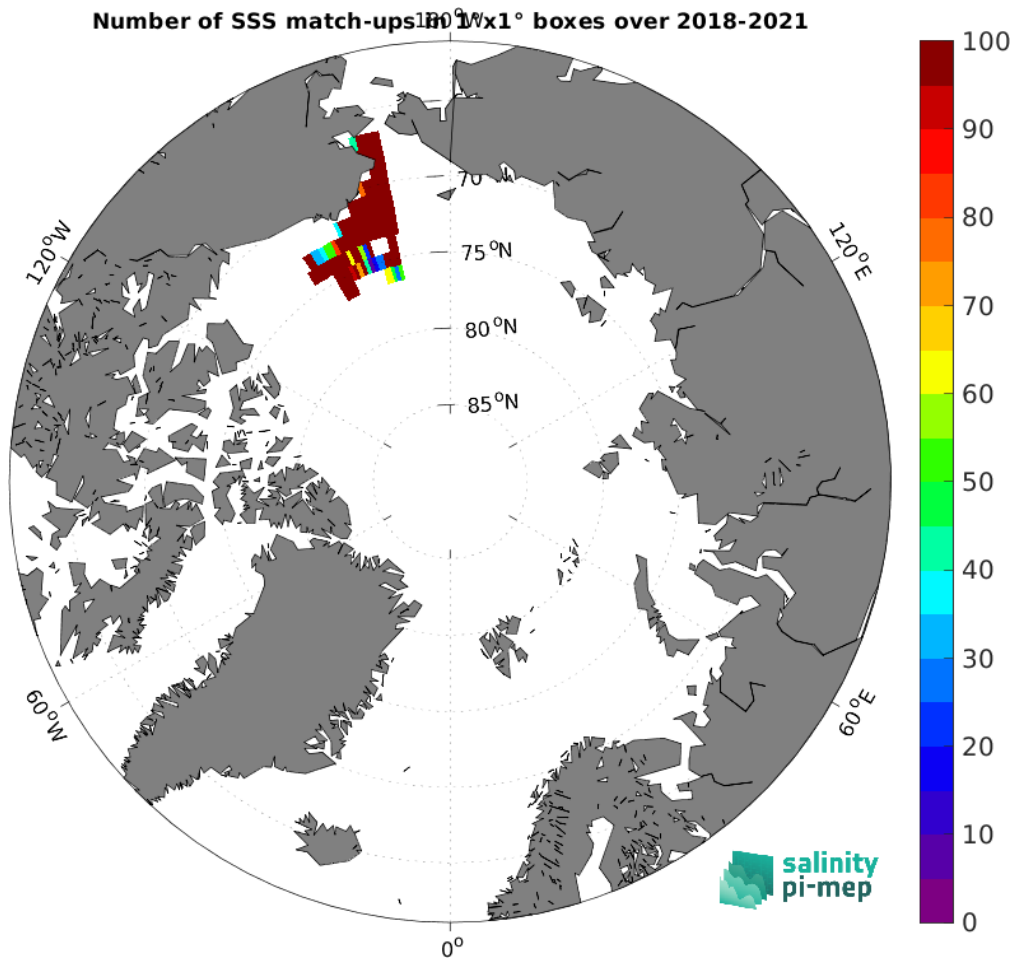
Figure 5: Number of SSS match-ups between Saildrone SSS and the SMAP SSS L4 OI v3 - Monthly (ESR) SSS product for the Arctic Ocean Pi-MEP region over 1^\circ \times 1^\circ boxes and for the full satellite product period.
