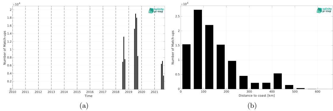
Figure 2: Number of match-ups between Sairdrone and SMAP SSS L4 OI v3 - Monthly (ESR) SSS as a function of time (a) and as function of the distance to coast (b) over the Arctic Ocean Pi-MEP region and for the full satellite product period.
