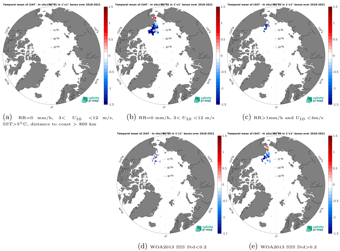
Figure 14: Temporal mean gridded over spatial boxes of size 1^\circ \times 1^\circ of \Delta SSS (SMAP SSS L4 OI v3 - Monthly (ESR) - Sailydrone) for 5 different subdatasets corresponding to:RR=0 mm/h, 3 < U_{10} < 12 m/s, SST > 5°C, distance to coast > 800 km (a), RR=0 mm/h, 3 < U_{10} < 12 m/s (b), RR > 1mm/h and U_{10} < 4 m/s (c), WOA2013 SSS Std < 0.2 (d), WOA2013 SSS Std > 0.2 (e).
