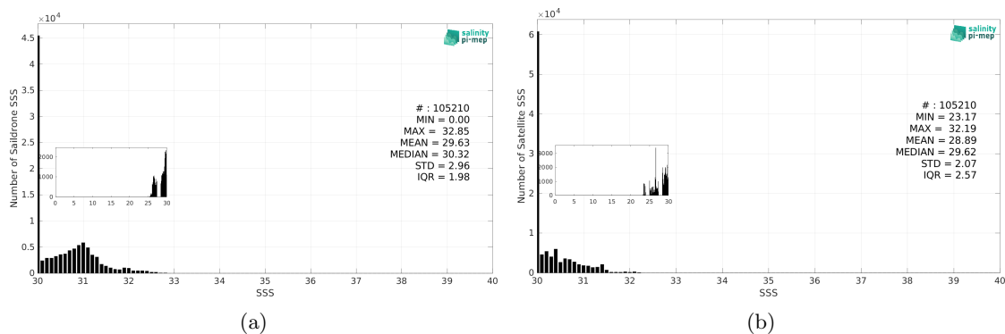
Figure 3: Histograms of SSS from Sairdrone (a) and SMAP SSS L4 OI v3 - Monthly (ESR) (b) considering all match-up pairs per bins of 0.1 over the Arctic Ocean Pi-MEP region and for the full satellite product period.
