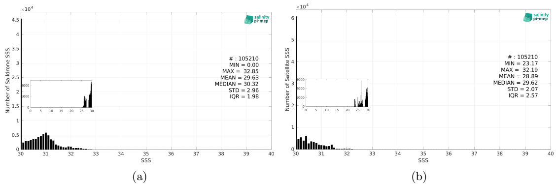
Figure 3: Histograms of SSS from Sailldrone (a) and SMAP SSS L4 OI v3 - Monthly (ESR) (b) considering all match-up pairs per bins of 0.1 over the Arctic Ocean Pi-MEP region and for the full satellite product period.
