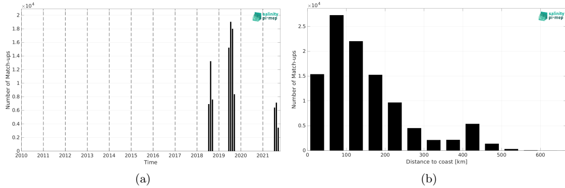
Figure 2: Number of match-ups between Sailldrone and SMAP SSS L4 OI v3 - Monthly (ESR) SSS as a function of time (a) and as function of the distance to coast (b) over the Arctic Ocean Pi-MEP region and for the full satellite product period.
