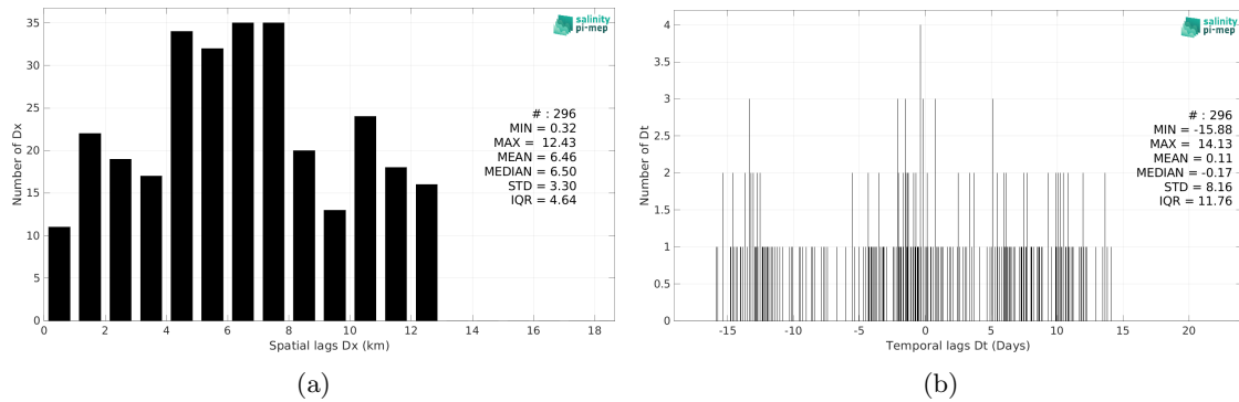
Figure 6: Histograms of the spatial (a) and temporal (b) lags between the location/time of the Marine mammals measurement and the date of the corresponding SMAP SSS L4 OI v3 - Monthly (ESR) SSS pixel.
