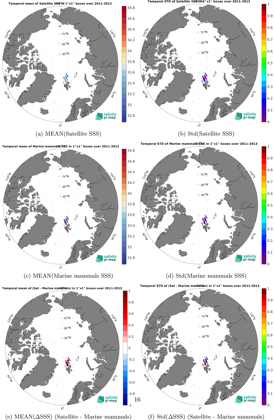
Figure 7: Temporal mean (left) and Std (right) of SSS from SMAP SSS L4 OI v3 - Monthly (ESR) (top), Marine mammals (middle), and of \Delta SSS (Satellite - Marine mammals). Only match-up pairs are used to generate these maps.
