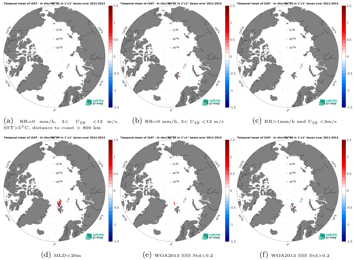
Figure 14: Temporal mean gridded over spatial boxes of size 1^\circ \times 1^\circ of \Delta SSS (SMAP SSS L4 OI v3 - Monthly (ESR) - Marine mammals) for 6 different subdatasets corresponding to:RR=0 mm/h, 3 < U_{10} < 12 m/s, SST>5°C, distance to coast > 800 km (a), RR=0 mm/h, 3 < U_{10} < 12 m/s (b), RR>1mm/h and U_{10} < 4 m/s (c),MLD<20m (d),WOA2013 SSS Std<0.2 (e),WOA2013 SSS Std>0.2 (f).
