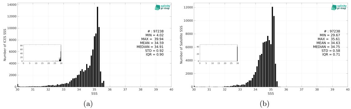
Figure 3: Histograms of SSS from ICES (a) and SMAP SSS L4 OI v3 - Monthly (ESR) (b) considering all match-up pairs per bins of 0.1 over the Arctic Ocean Pi-MEP region and for the full satellite product period.
