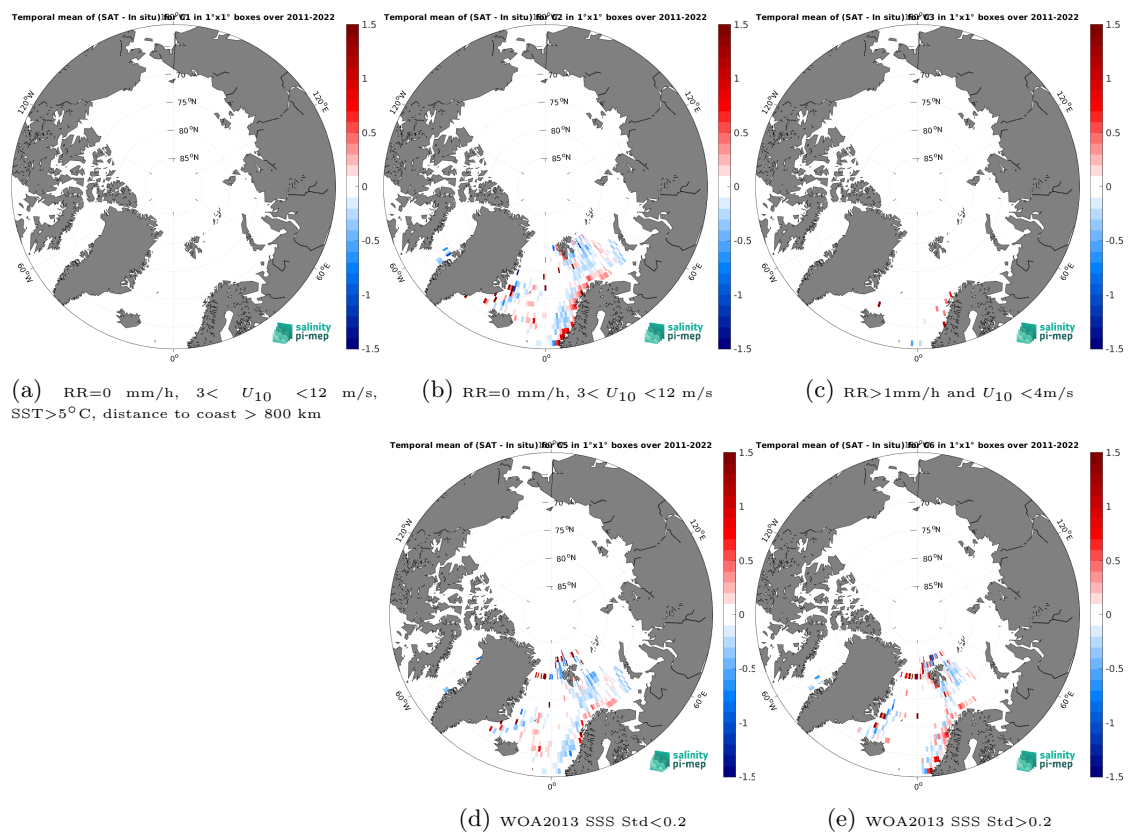
Figure 14: Temporal mean gridded over spatial boxes of size 1^\circ \times 1^\circ of \Delta SSS (SMAP SSS L4 OI v3 - Monthly (ESR) - ICES) for 5 different subdatasets corresponding to: RR=0 mm/h, 3 < U_{10} < 12 m/s, SST > 5°C, distance to coast > 800 km (a), RR=0 mm/h, 3 < U_{10} < 12 m/s (b), RR > 1mm/h and U_{10} < 4 m/s (c), WOA2013 SSS Std < 0.2 (d), WOA2013 SSS Std > 0.2 (e).
