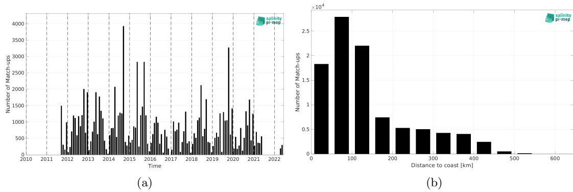
Figure 2: Number of match-ups between ICES and SMAP SSS L4 OI v3 - Monthly (ESR) SSS as a function of time (a) and as function of the distance to coast (b) over the Arctic Ocean Pi-MEP region and for the full satellite product period.
