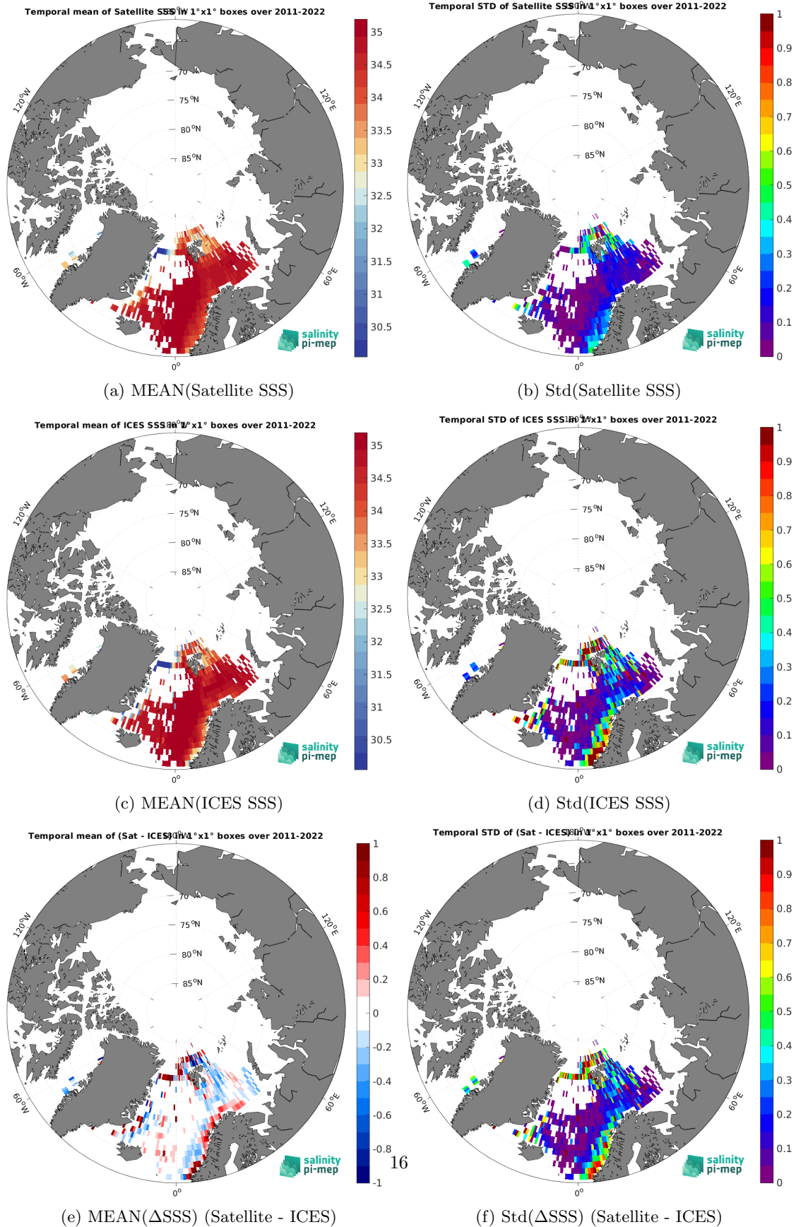
Figure 7: Temporal mean (left) and Std (right) of SSS from SMAP SSS L4 OI v3 - Monthly (ESR) (top), ICES (middle), and of \Delta SSS (Satellite - ICES). Only match-up pairs are used to generate these maps.
