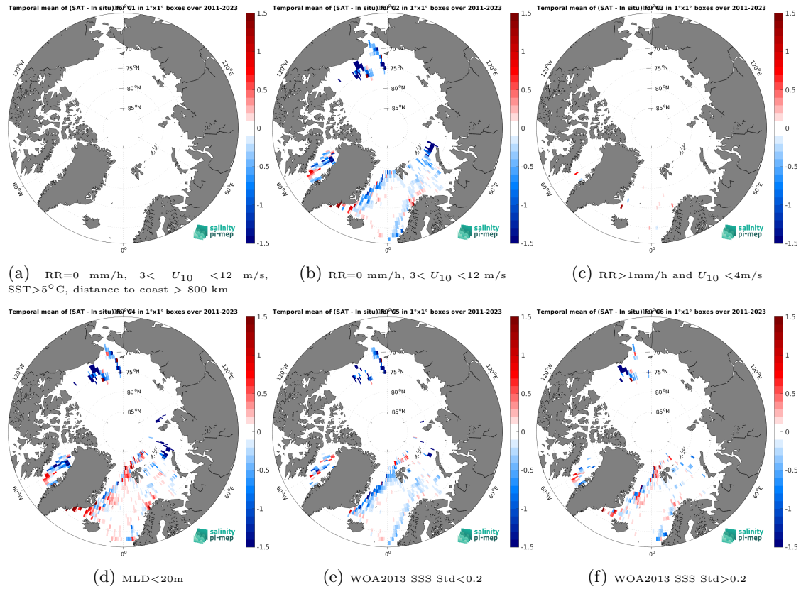
Figure 14: Temporal mean gridded over spatial boxes of size 1^\circ \times 1^\circ of \Delta\text{SSS} (SMAP SSS L4 OI v3 - Monthly (ESR) - Argo) for 6 different subdatasets corresponding to:RR=0 mm/h, 3 < U_{10} < 12 m/s, SST>5°C, distance to coast > 800 km (a), RR=0 mm/h, 3 < U_{10} < 12 m/s (b), RR>1mm/h and U_{10} < 4 m/s (c),MLD<20m (d),WOA2013 SSS Std<0.2 (e),WOA2013 SSS Std>0.2 (f).
