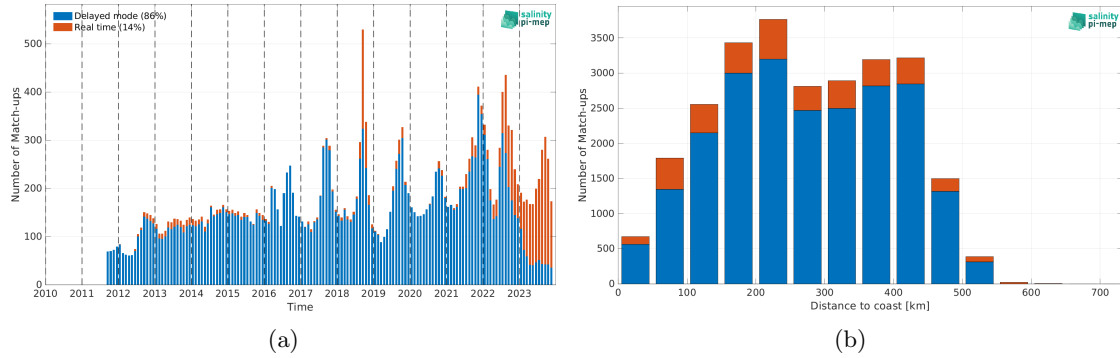
Figure 2: Number of match-ups between Argo and SMAP SSS L4 OI v3 - Monthly (ESR) SSS as a function of time (a) and as function of the distance to coast (b) over the Arctic Ocean Pi-MEP region and for the full satellite product period.
