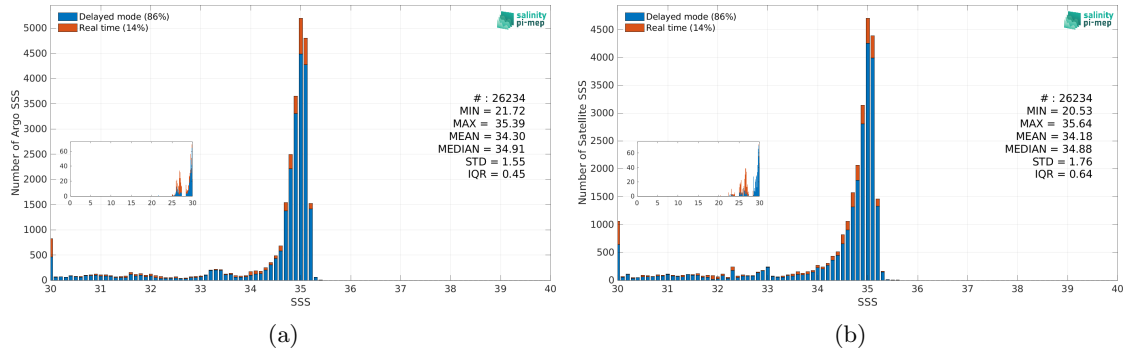
Figure 3: Histograms of SSS from Argo (a) and SMAP SSS L4 OI v3 - Monthly (ESR) (b) considering all match-up pairs per bins of 0.1 over the Arctic Ocean Pi-MEP region and for the full satellite product period.
