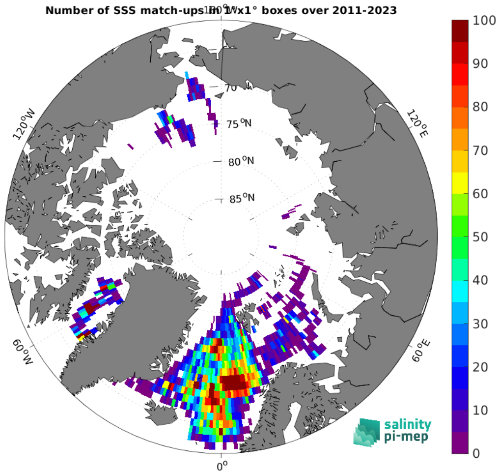
Figure 5: Number of SSS match-ups between Argo SSS and the SMAP SSS L4 OI v3 - Monthly (ESR) SSS product for the Arctic Ocean Pi-MEP region over 1^\circ \times 1^\circ boxes and for the full satellite product period.
