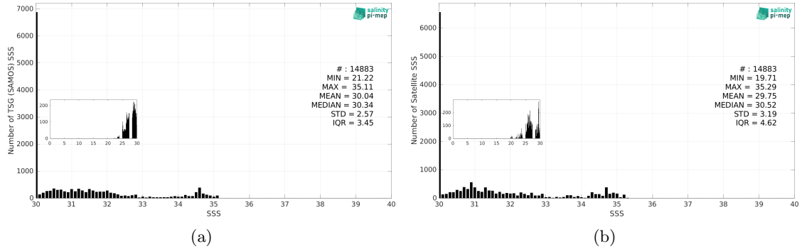
Figure 3: Histograms of SSS from TSG (SAMOS) (a) and SMAP SSS L4 OI v3 - Daily (ESR) (b) considering all match-up pairs per bins of 0.1 over the Arctic Ocean Pi-MEP region and for the full satellite product period.
