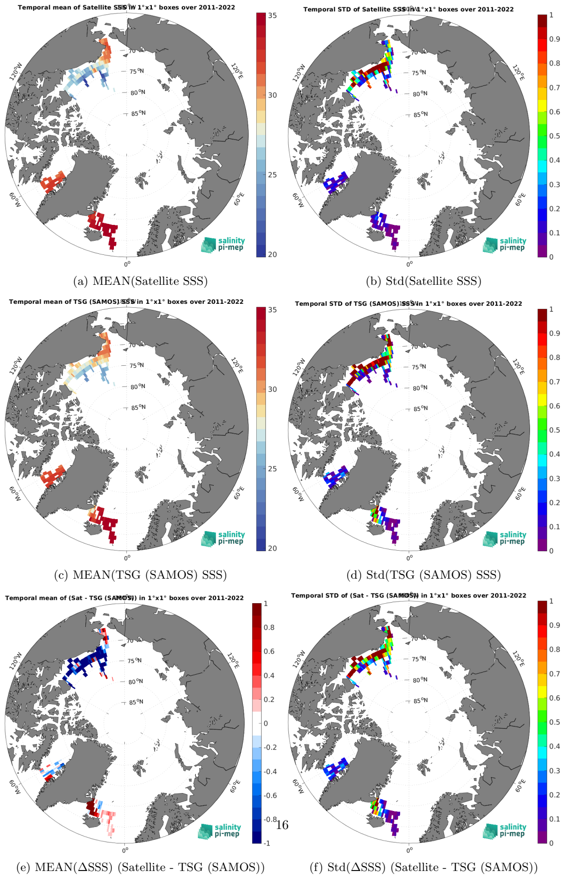
Figure 7: Temporal mean (left) and Std (right) of SSS from SMAP SSS L4 OI v3 - Daily (ESR) (top), TSG (SAMOS) (middle), and of \Delta SSS (Satellite - TSG (SAMOS)). Only match-up pairs are used to generate these maps.
