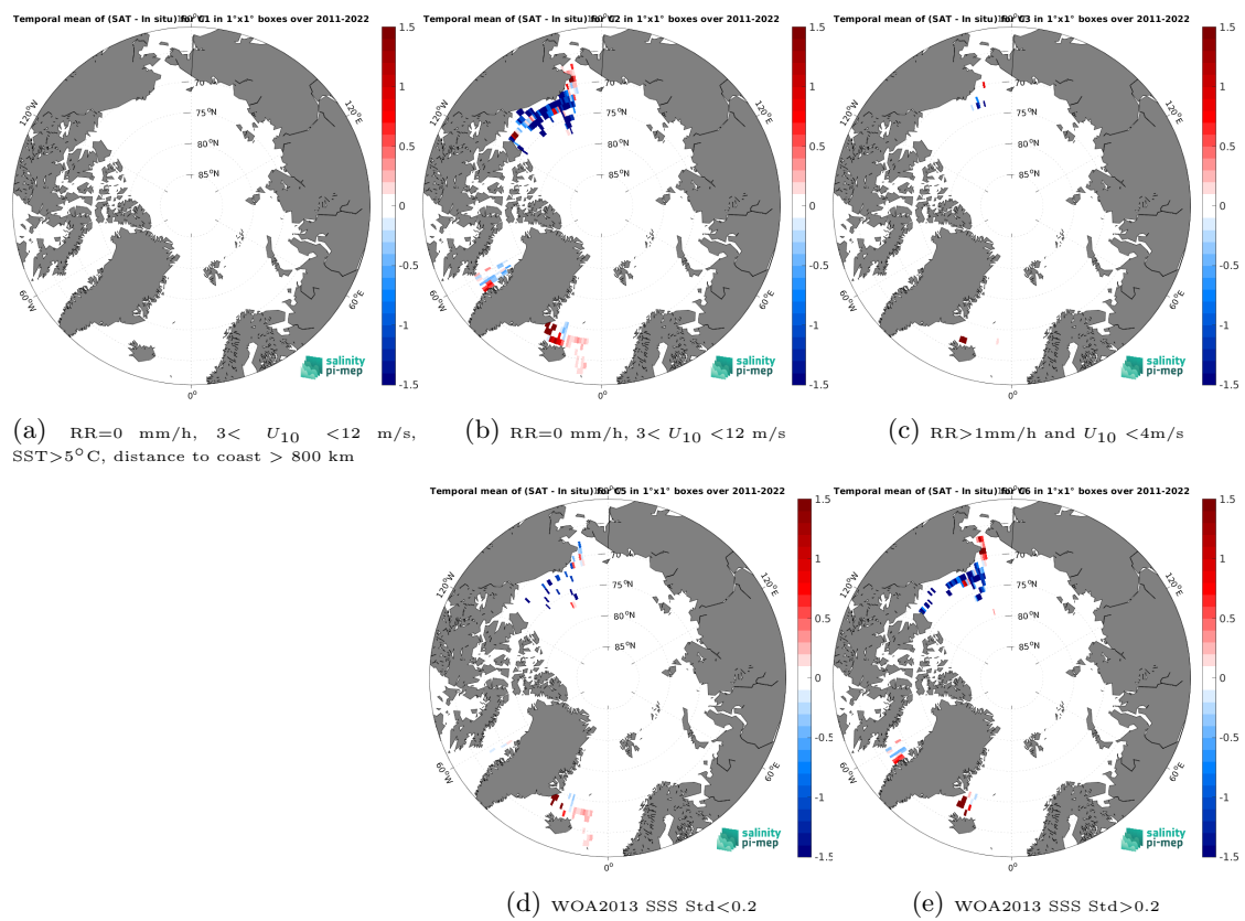
Figure 14: Temporal mean gridded over spatial boxes of size 1^\circ \times 1^\circ of \Delta SSS (SMAP SSS L4 OI v3 - Daily (ESR) - TSG (SAMOS)) for 5 different subdatasets corresponding to: RR=0 mm/h, 3 < U_{10} < 12 m/s, SST > 5°C, distance to coast > 800 km (a), RR=0 mm/h, 3 < U_{10} < 12 m/s (b), RR > 1mm/h and U_{10} < 4 m/s (c), WOA2013 SSS Std < 0.2 (d), WOA2013 SSS Std > 0.2 (e).
