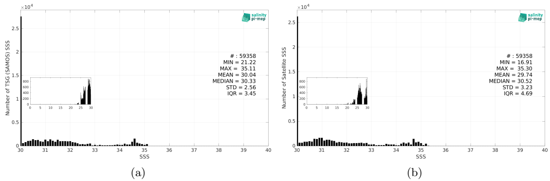
Figure 3: Histograms of SSS from TSG (SAMOS) (a) and SMAP SSS L4 OI v3 - Daily (ESR) (b) considering all match-up pairs per bins of 0.1 over the Arctic Ocean Pi-MEP region and for the full satellite product period.
