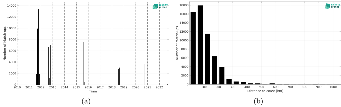
Figure 2: Number of match-ups between TSG (SAMOS) and SMAP SSS L4 OI v3 - Daily (ESR) SSS as a function of time (a) and as function of the distance to coast (b) over the Arctic Ocean Pi-MEP region and for the full satellite product period.
