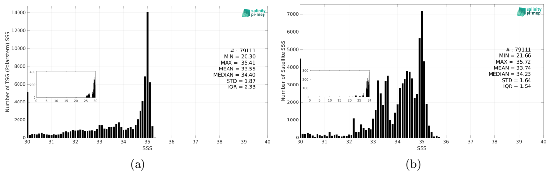
Figure 3: Histograms of SSS from TSG (Polarstern) (a) and SMAP SSS L4 OI v3 - Daily (ESR) (b) considering all match-up pairs per bins of 0.1 over the Arctic Ocean Pi-MEP region and for the full satellite product period.
