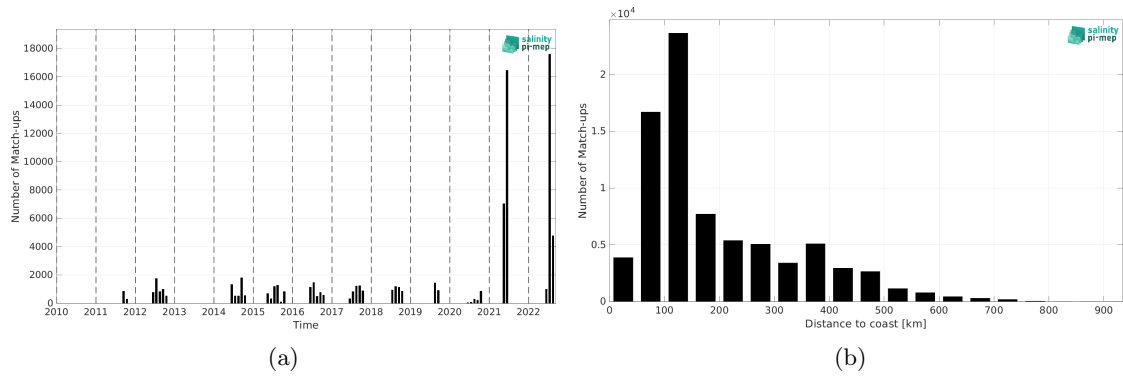
Figure 2: Number of match-ups between TSG (Polarstern) and SMAP SSS L4 OI v3 - Daily (ESR) SSS as a function of time (a) and as function of the distance to coast (b) over the Arctic Ocean Pi-MEP region and for the full satellite product period.
