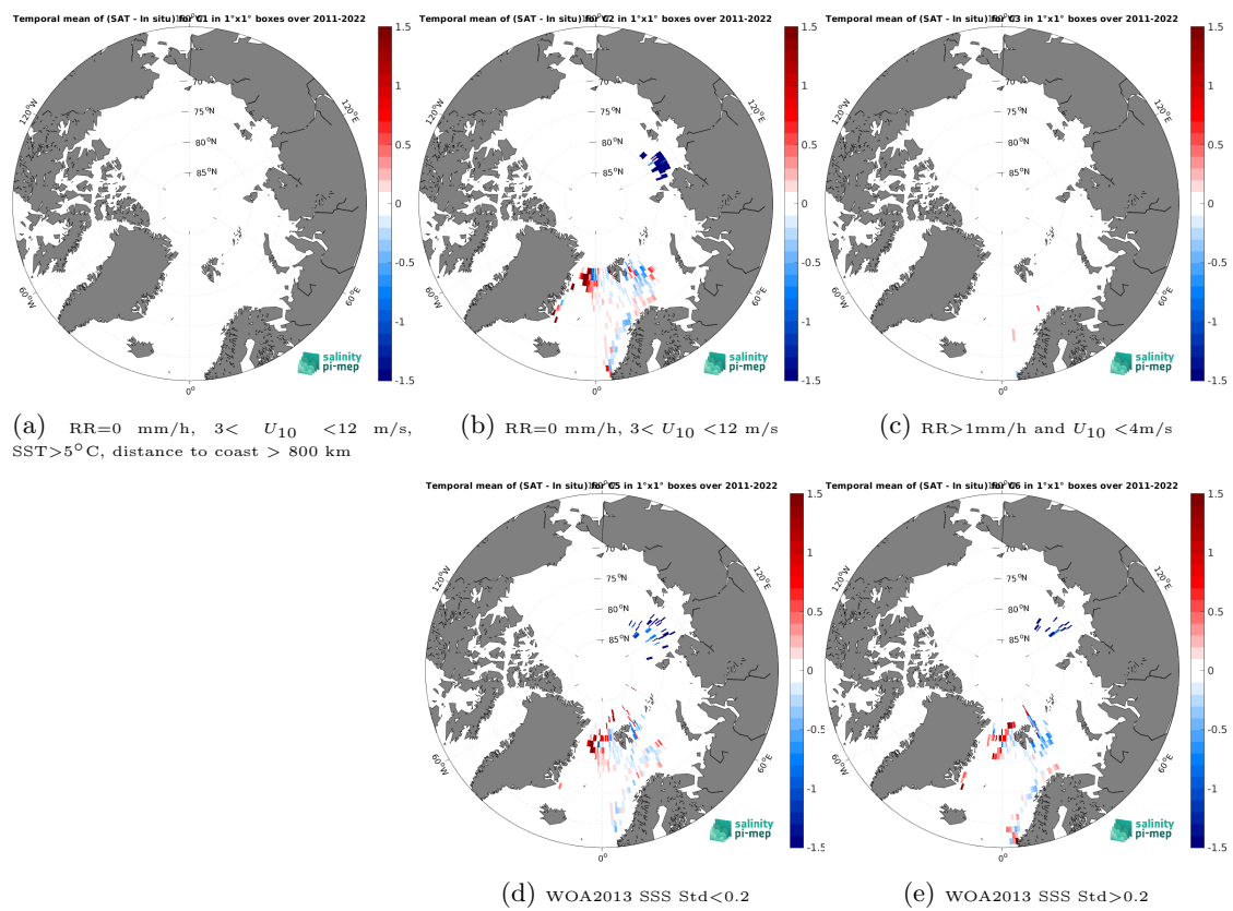
Figure 14: Temporal mean gridded over spatial boxes of size 1^\circ \times 1^\circ of \Delta SSS (SMAP SSS L4 OI v3 - Daily (ESR) - TSG (Polarstern)) for 5 different subdatasets corresponding to: RR=0 mm/h, 3 < U_{10} < 12 m/s, SST > 5°C, distance to coast > 800 km (a), RR=0 mm/h, 3 < U_{10} < 12 m/s (b), RR > 1mm/h and U_{10} < 4 m/s (c), WOA2013 SSS Std < 0.2 (d), WOA2013 SSS Std > 0.2 (e).
