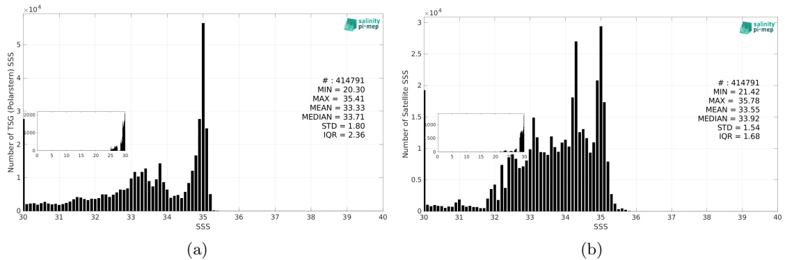
Figure 3: Histograms of SSS from TSG (Polarstern) (a) and SMAP SSS L4 OI v3 - Daily (ESR) (b) considering all match-up pairs per bins of 0.1 over the Arctic Ocean Pi-MEP region and for the full satellite product period.
