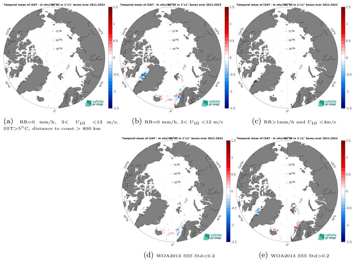
Figure 14: Temporal mean gridded over spatial boxes of size 1^\circ \times 1^\circ of \Delta SSS (SMAP SSS L4 OI v3 - Daily (ESR) - TSG (LEGOS-DM)) for 5 different subdatasets corresponding to:RR=0 mm/h, 3 < U_{10} < 12 m/s, SST > 5°C, distance to coast > 800 km (a), RR=0 mm/h, 3 < U_{10} < 12 m/s (b), RR > 1mm/h and U_{10} < 4 m/s (c), WOA2013 SSS Std < 0.2 (d), WOA2013 SSS Std > 0.2 (e).
