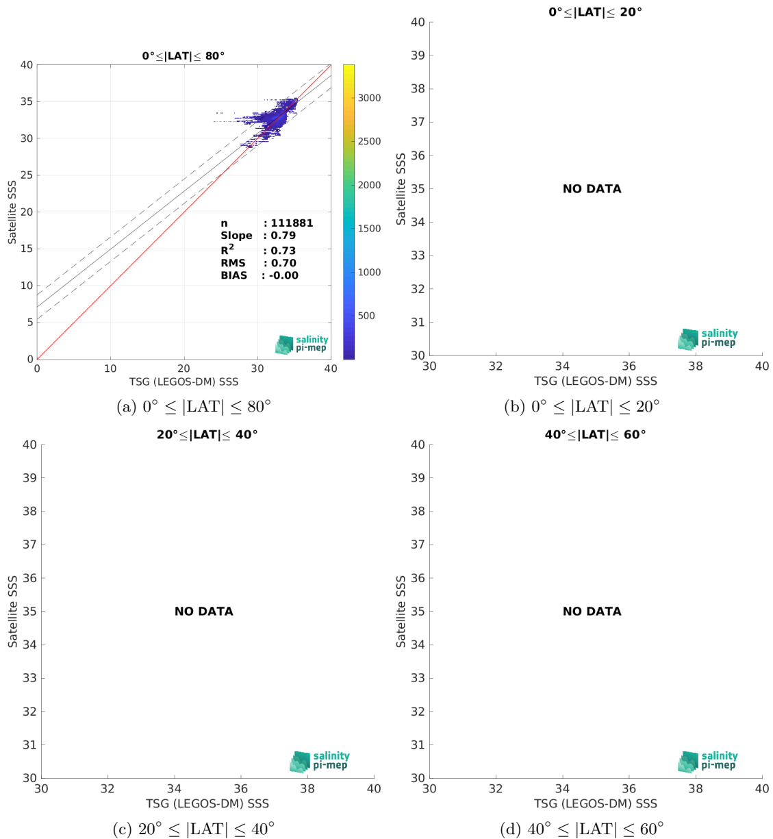
Figure 10: Contour maps of the concentration of SMAP SSS L4 OI v3 - Daily (ESR) SSS (y-axis) versus TSG (LEGOS-DM) SSS (x-axis) at match-up pairs for different latitude bands. For each plot, the red line shows x=y . The black thin and dashed lines indicate a linear fit through the data cloud and the \pm 95\% confidence levels, respectively. The number match-up pairs n , the slope and R^2 coefficient of the linear fit, the root mean square (RMS) and the mean bias between satellite and in situ data are indicated for each latitude band in each plots.
