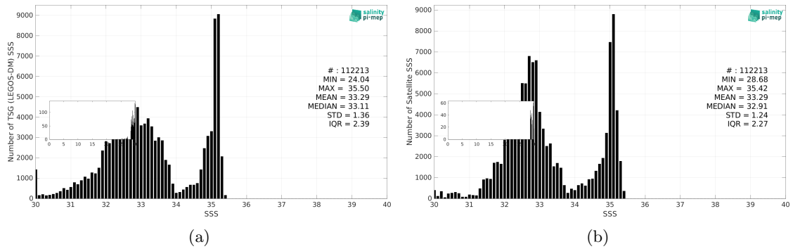
Figure 3: Histograms of SSS from TSG (LEGOS-DM) (a) and SMAP SSS L4 OI v3 - Daily (ESR) (b) considering all match-up pairs per bins of 0.1 over the Arctic Ocean Pi-MEP region and for the full satellite product period.
