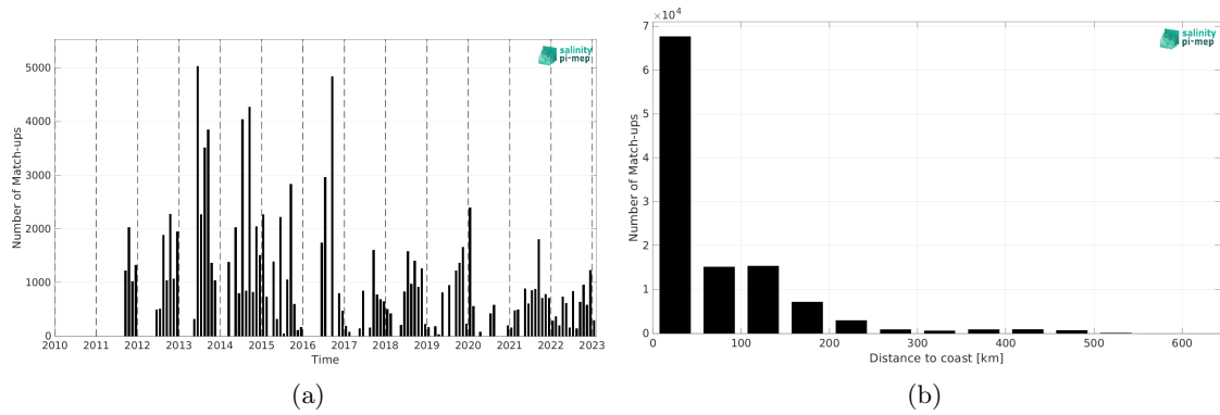
Figure 2: Number of match-ups between TSG (LEGOS-DM) and SMAP SSS L4 OI v3 - Daily (ESR) SSS as a function of time (a) and as function of the distance to coast (b) over the Arctic Ocean Pi-MEP region and for the full satellite product period.
