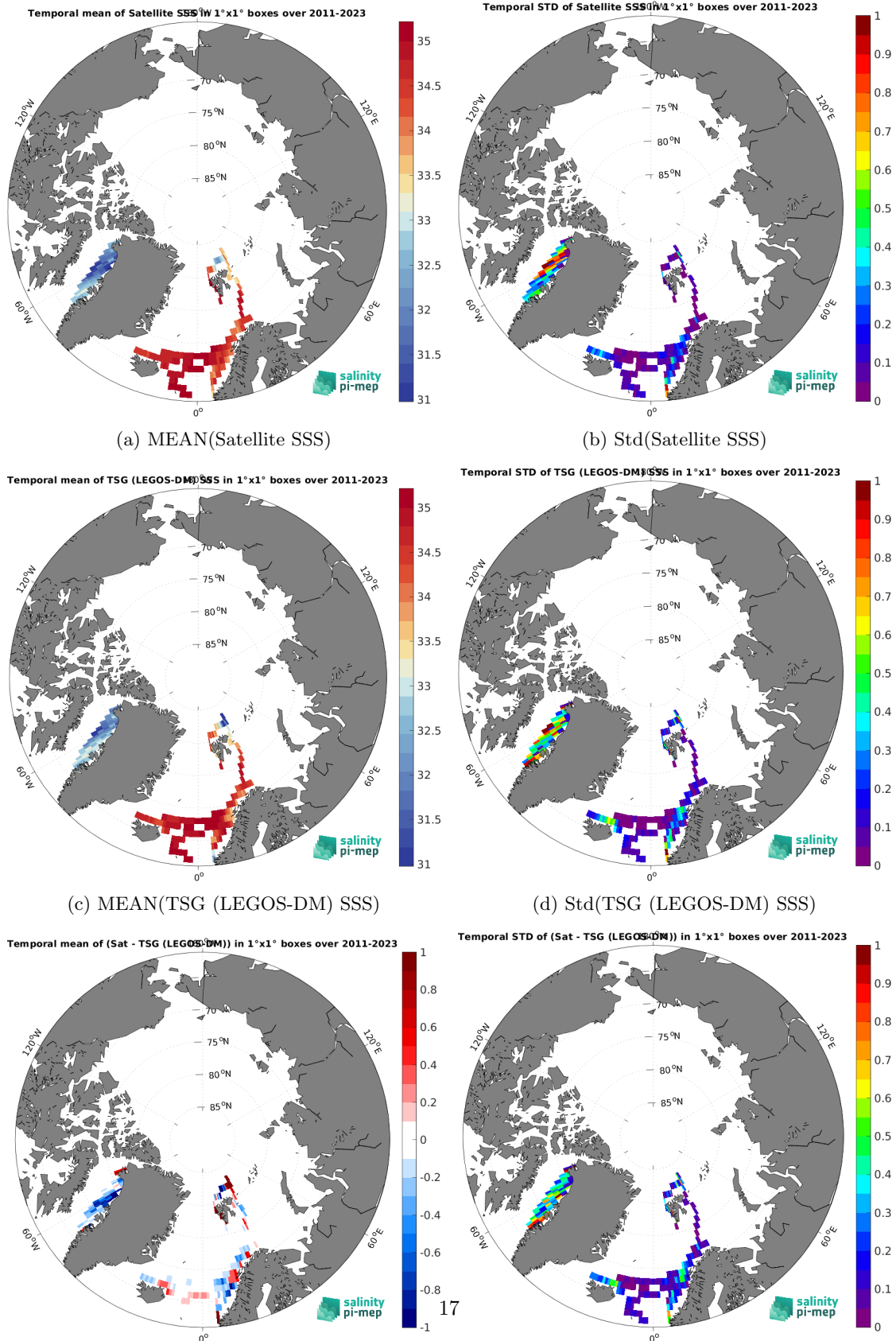
(e) MEAN( \Delta SSS) (Satellite - TSG (LEGOS-DM)) (f) Std( \Delta SSS) (Satellite - TSG (LEGOS-DM)) Figure 7: Temporal mean (left) and Std (right) of SSS from SMAP SSS L4 OI v3 - Daily (ESR) (top), TSG (LEGOS-DM) (middle), and of \Delta SSS (Satellite - TSG (LEGOS-DM)). Only match-up pairs are used to generate these maps.
