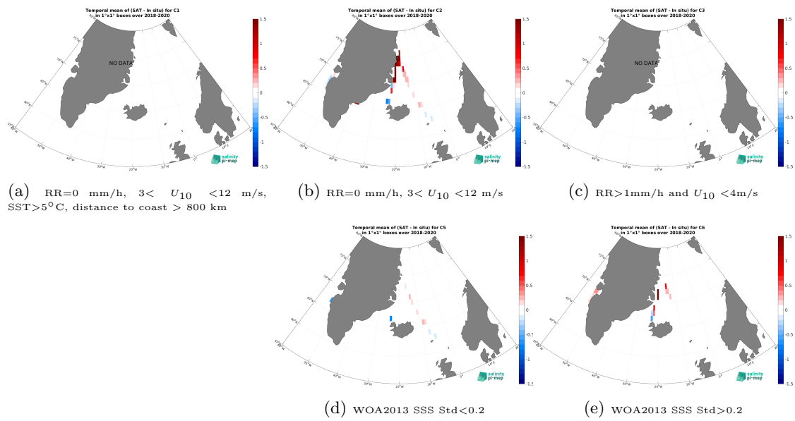
Figure 14: Temporal mean gridded over spatial boxes of size 1^\circ \times 1^\circ of \Delta SSS (SMAP SSS L4 OI v3 - Daily (ESR) - TSG (Lauge-Koch)) for 5 different subdatasets corresponding to:RR=0 mm/h, 3 < U_{10} < 12 m/s, SST > 5^\circ\text{C} , distance to coast > 800 km (a), RR=0 mm/h, 3 < U_{10} < 12 m/s (b), RR > 1 mm/h and U_{10} < 4 m/s (c), WOA2013 SSS Std < 0.2 (d), WOA2013 SSS Std > 0.2 (e).
