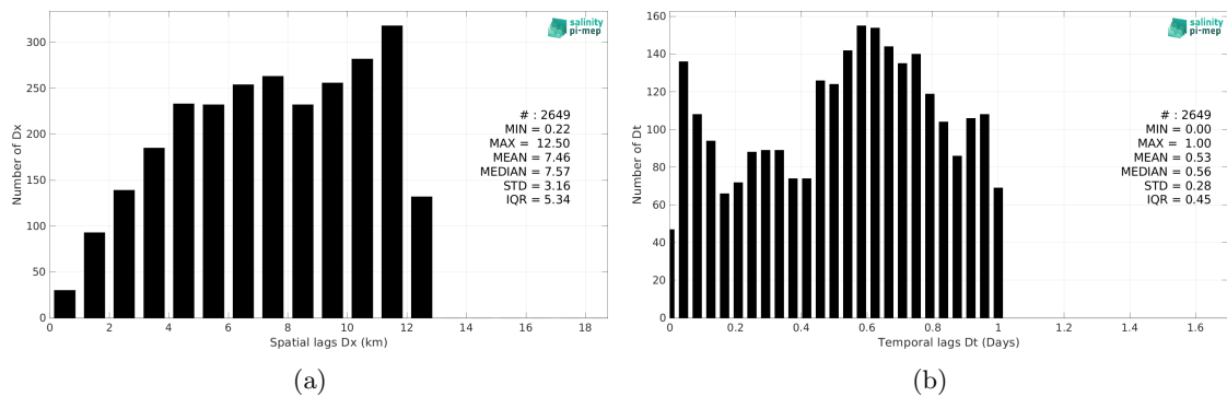
Figure 6: Histograms of the spatial (a) and temporal (b) lags between the location/time of the TSG (Laue-Koch) measurement and the date of the corresponding SMAP SSS L4 OI v3 - Daily (ESR) SSS pixel.
