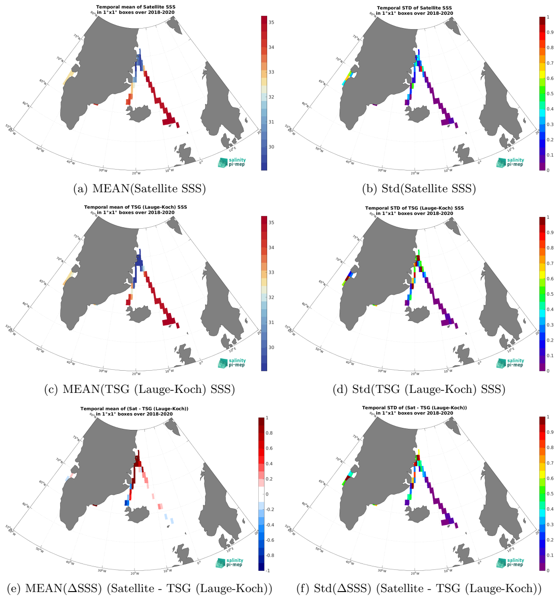
Figure 7: Temporal mean (left) and Std (right) of SSS from SMAP SSS L4 OI v3 - Daily (ESR) (top), TSG (Lauge-Koch) (middle), and of \Delta SSS (Satellite - TSG (Lauge-Koch)). Only match-up pairs are used to generate these maps.
