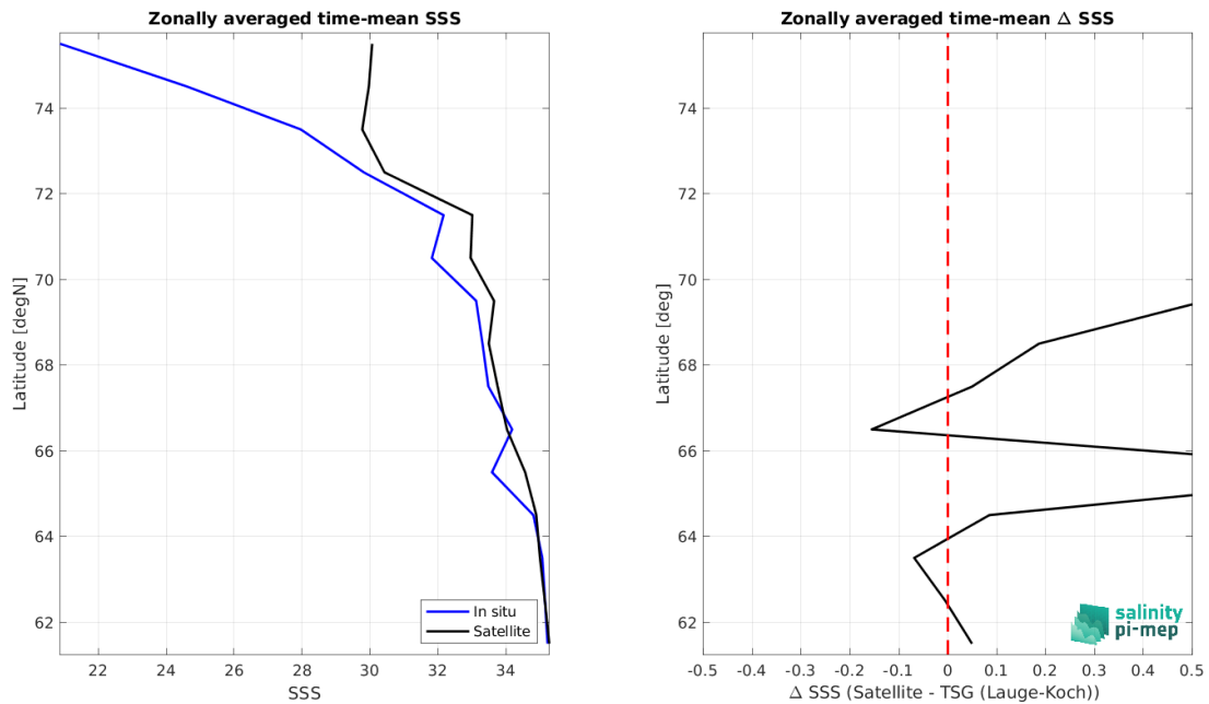
Figure 9: Left panel: Zonal mean SSS from SMAP SSS L4 OI v3 - Daily (ESR) satellite product (black) and from TSG (Lauge-Koch) (blue). Right panel: Zonal mean of \Delta SSS (Satellite - TSG (Lauge-Koch)) for all the collected Pi-MEP match-up pairs estimated over the full satellite product period.
