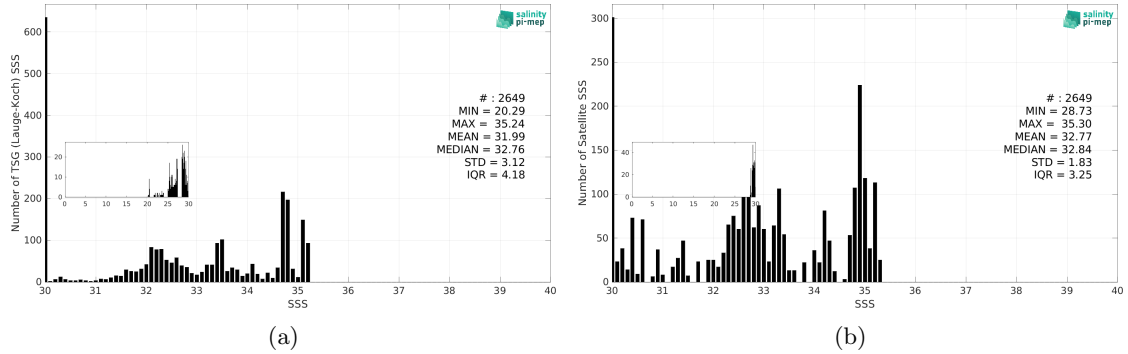
Figure 3: Histograms of SSS from TSG (Lauge-Koch) (a) and SMAP SSS L4 OI v3 - Daily (ESR) (b) considering all match-up pairs per bins of 0.1 over the Arctic Ocean Pi-MEP region and for the full satellite product period.
