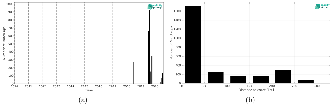
Figure 2: Number of match-ups between TSG (Lauge-Koch) and SMAP SSS L4 OI v3 - Daily (ESR) SSS as a function of time (a) and as function of the distance to coast (b) over the Arctic Ocean Pi-MEP region and for the full satellite product period.
