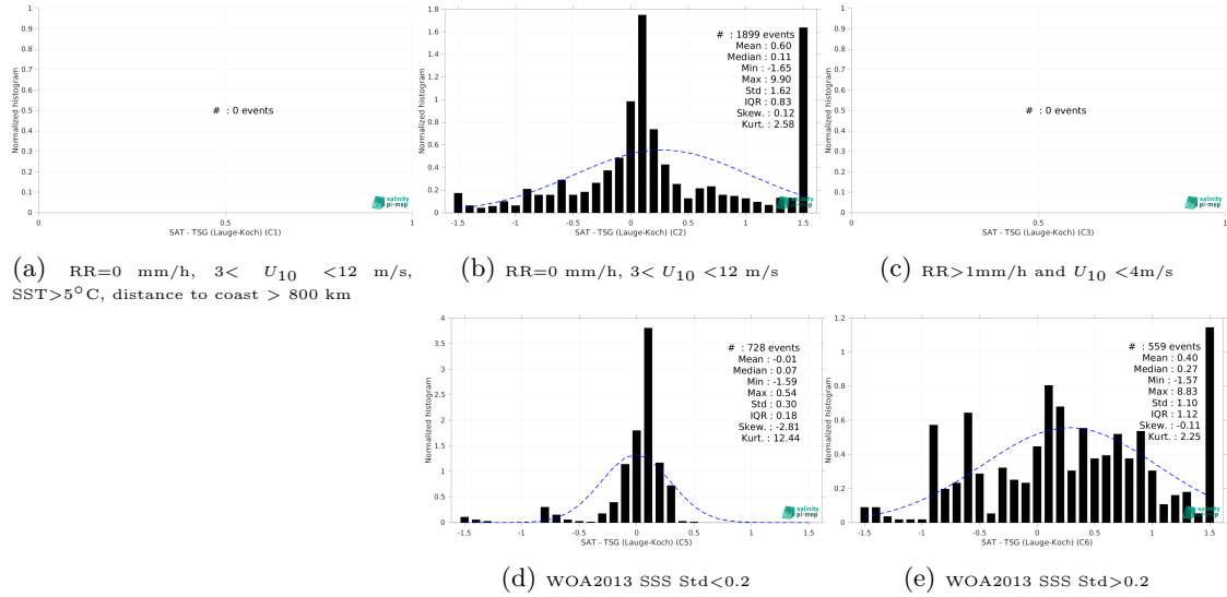
Figure 15: Normalized histogram of \Delta SSS (SMAP SSS L4 OI v3 - Daily (ESR) - TSG (Lauge-Koch)) for 5 different subdatasets corresponding to: RR=0 mm/h, 3 < U_{10} < 12 m/s, SST > 5°C, distance to coast > 800 km (a), RR=0 mm/h, 3 < U_{10} < 12 m/s (b), RR > 1mm/h and U_{10} < 4 m/s (c), WOA2013 SSS Std < 0.2 (d), WOA2013 SSS Std > 0.2 (e).
