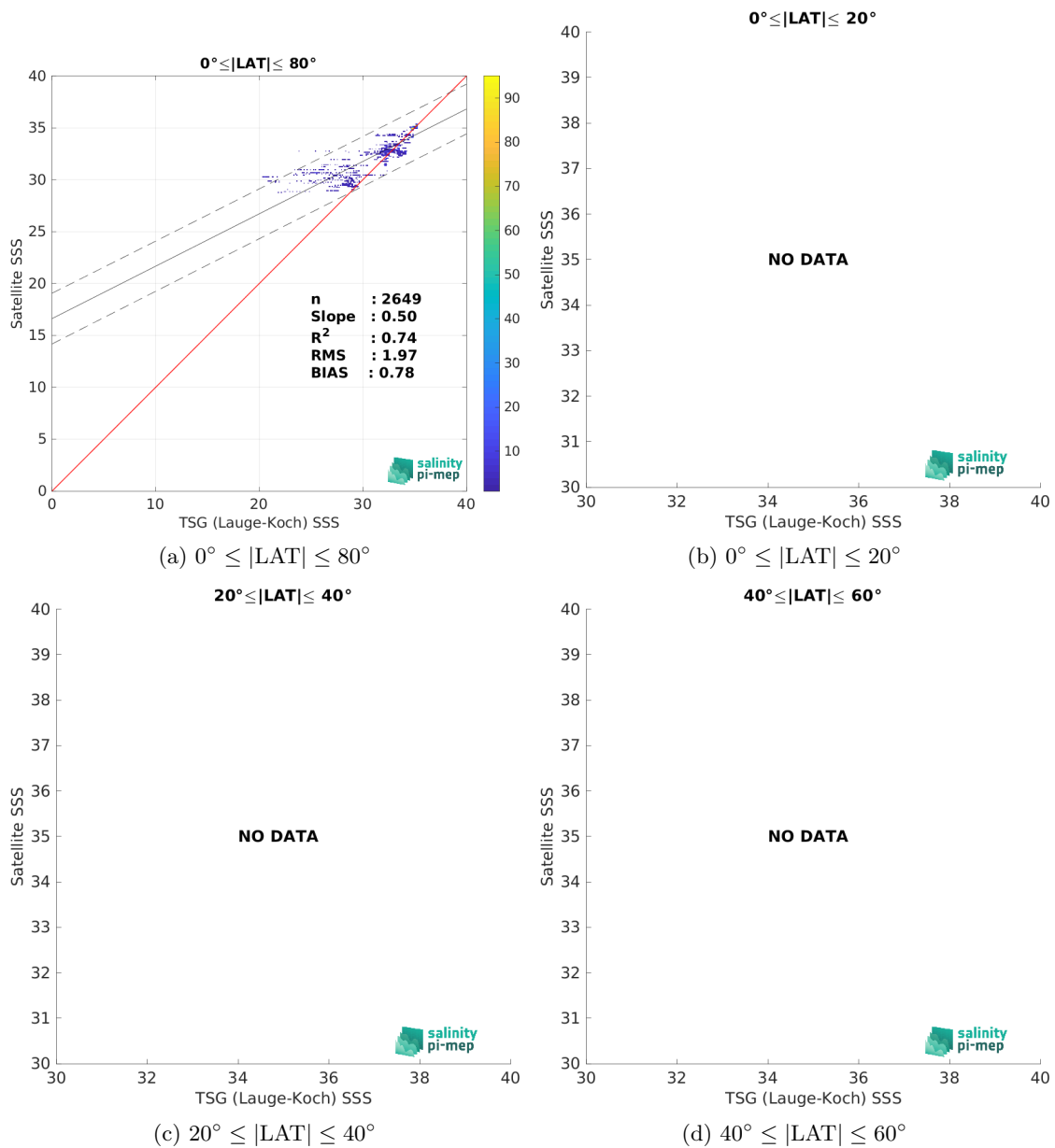
Figure 10: Contour maps of the concentration of SMAP SSS L4 OI v3 - Daily (ESR) SSS (y-axis) versus TSG (Lauge-Koch) SSS (x-axis) at match-up pairs for different latitude bands. For each plot, the red line shows x=y . The black thin and dashed lines indicate a linear fit through the data cloud and the \pm 95\% confidence levels, respectively. The number match-up pairs n , the slope and R^2 coefficient of the linear fit, the root mean square (RMS) and the mean bias between satellite and in situ data are indicated for each latitude band in each plots.
