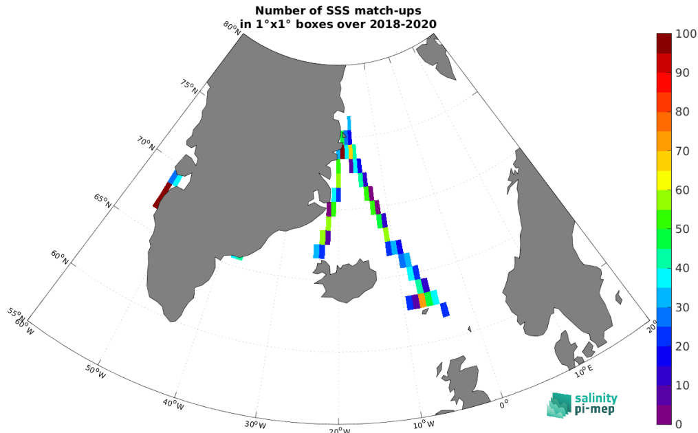
Figure 5: Number of SSS match-ups between TSG (Laue-Koch) SSS and the SMAP SSS L4 OI v3 - Daily (ESR) SSS product for the Arctic Ocean Pi-MEP region over 1°x1° boxes and for the full satellite product period.
