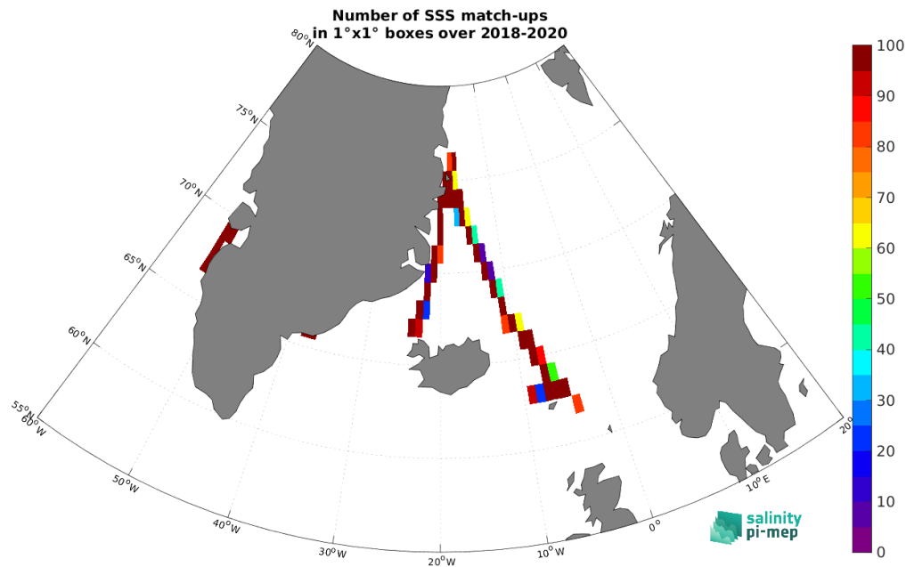
Figure 5: Number of SSS match-ups between TSG (Lauge-Koch) SSS and the SMAP SSS L4 OI v3 - Daily (ESR) SSS product for the Arctic Ocean Pi-MEP region over 1^\circ \times 1^\circ boxes and for the full satellite product period.
