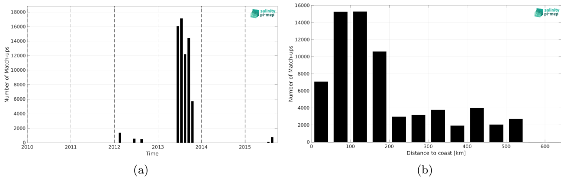
Figure 2: Number of match-ups between TSG (GOSUD-Sailing-ship) and SMAP SSS L4 OI v3 - Daily (ESR) SSS as a function of time (a) and as function of the distance to coast (b) over the Arctic Ocean Pi-MEP region and for the full satellite product period.
