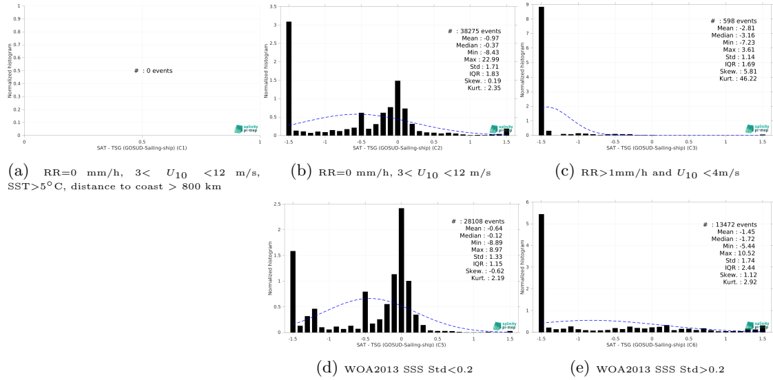
Figure 15: Normalized histogram of \Delta SSS (SMAP SSS L4 OI v3 - Daily (ESR) - TSG (GOSUD-Sailing-ship)) for 5 different subdatasets corresponding to: RR=0 mm/h, 3 < U_{10} < 12 m/s, SST > 5°C, distance to coast > 800 km (a), RR=0 mm/h, 3 < U_{10} < 12 m/s (b), RR > 1mm/h and U_{10} < 4 m/s (c), WOA2013 SSS Std < 0.2 (d), WOA2013 SSS Std > 0.2 (e).
