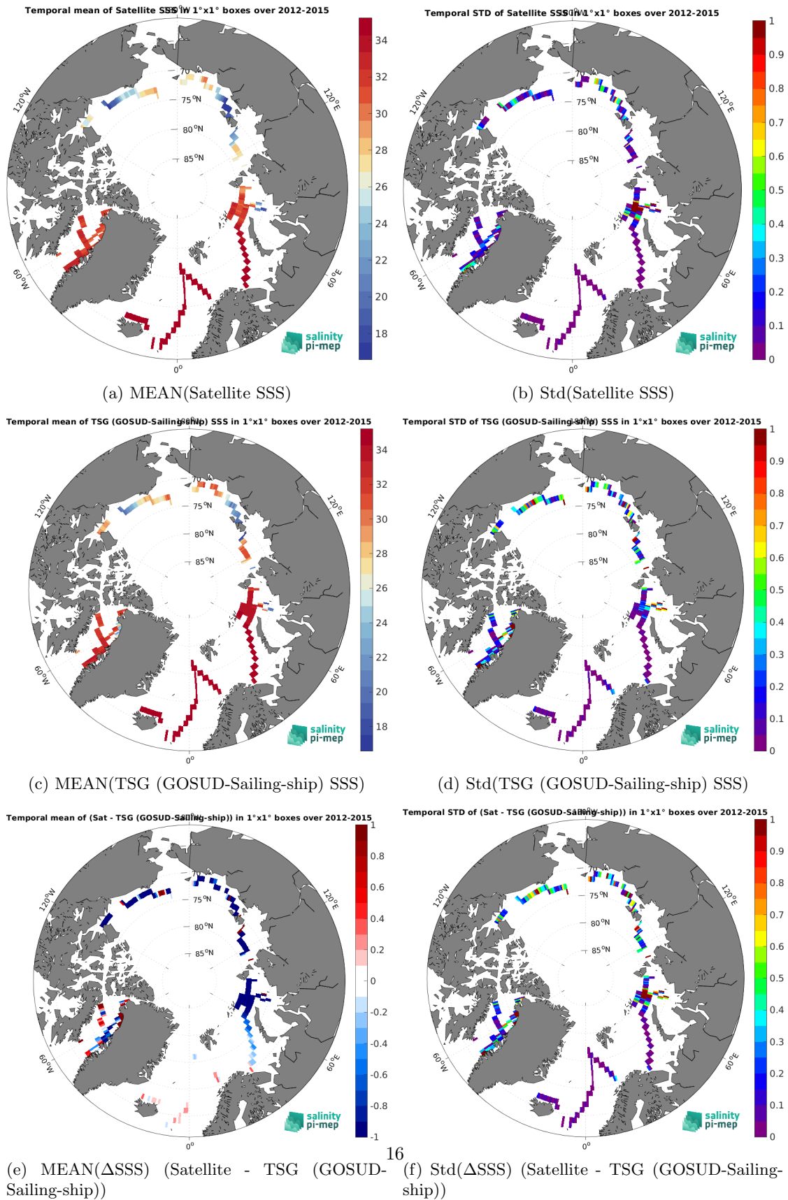
Figure 7: Temporal mean (left) and Std (right) of SSS from SMAP SSS L4 OI v3 - Daily (ESR) (top), TSG (GOSUD-Sailing-ship) (middle), and of \Delta SSS (Satellite - TSG (GOSUD-Sailing-ship)). Only match-up pairs are used to generate these maps.
