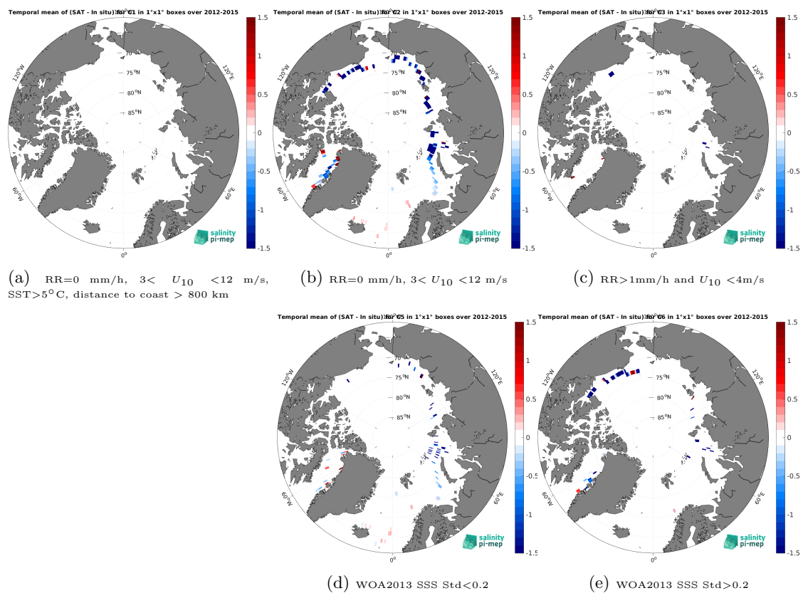
Figure 14: Temporal mean gridded over spatial boxes of size 1^\circ \times 1^\circ of \Delta SSS (SMAP SSS L4 OI v3 - Daily (ESR) - TSG (GOSUD-Sailing-ship)) for 5 different subdatasets corresponding to: RR=0 mm/h, 3 < U_{10} < 12 m/s, SST > 5^\circ\text{C} , distance to coast > 800 km (a), RR=0 mm/h, 3 < U_{10} < 12 m/s (b), RR > 1 mm/h and U_{10} < 4 m/s (c), WOA2013 SSS Std < 0.2 (d), WOA2013 SSS Std > 0.2 (e).
