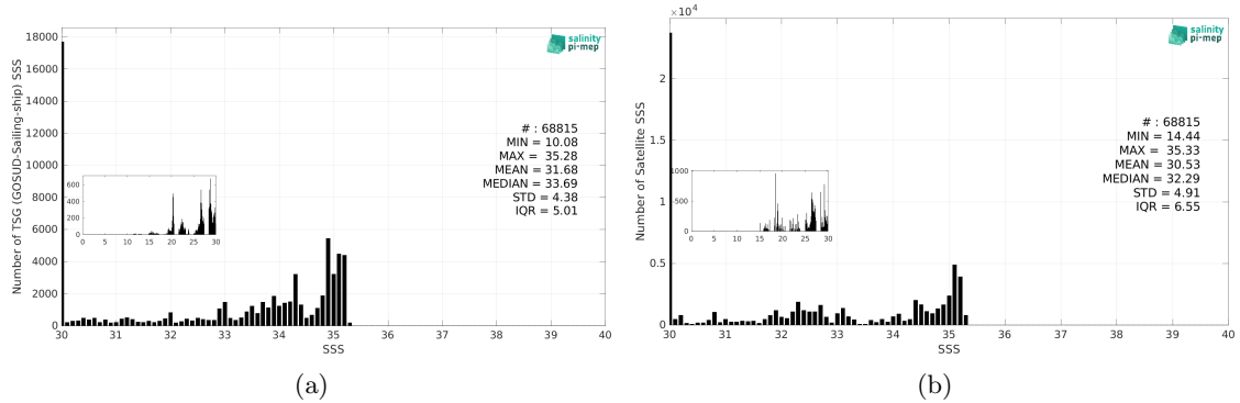
Figure 3: Histograms of SSS from TSG (GOSUD-Sailing-ship) (a) and SMAP SSS L4 OI v3 - Daily (ESR) (b) considering all match-up pairs per bins of 0.1 over the Arctic Ocean Pi-MEP region and for the full satellite product period.
