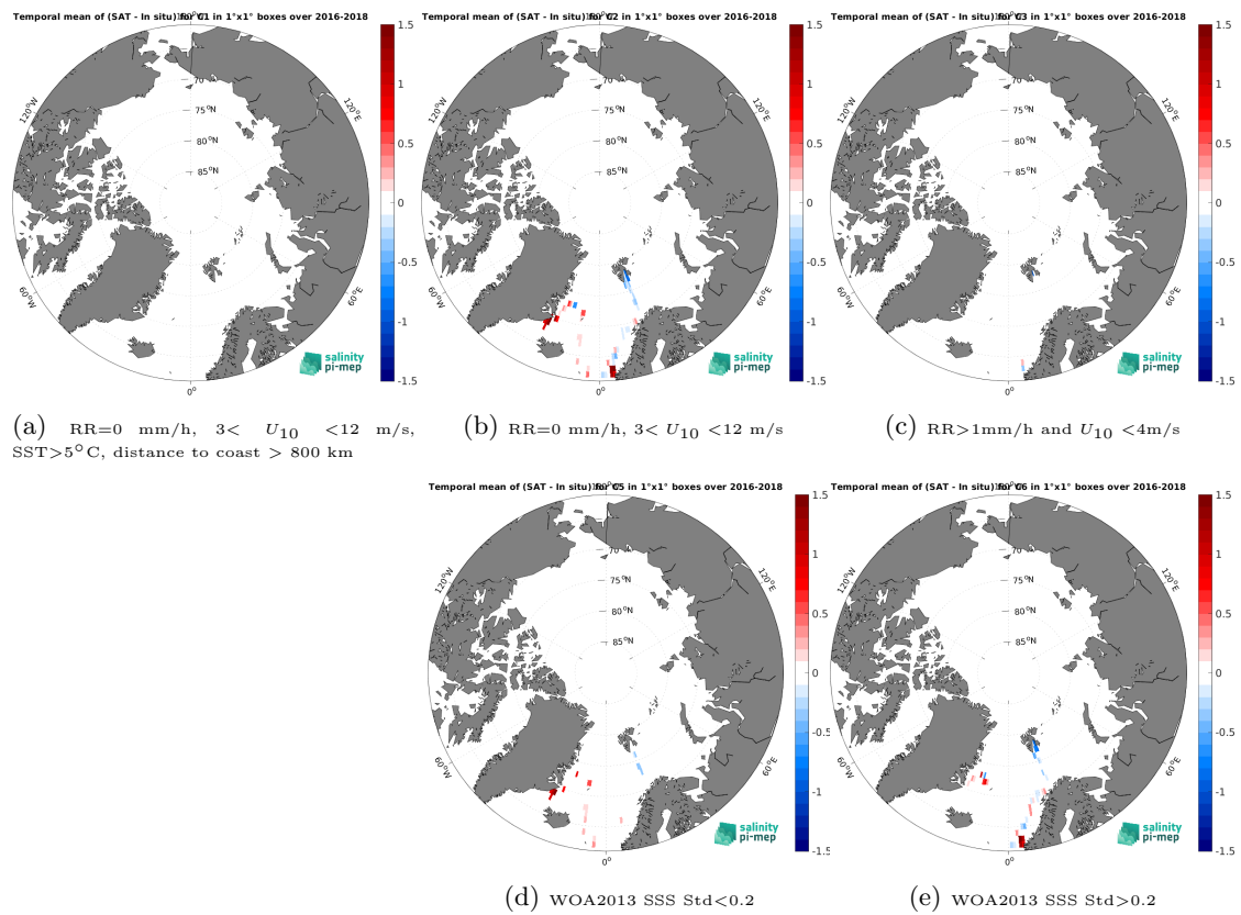
Figure 14: Temporal mean gridded over spatial boxes of size 1^\circ \times 1^\circ of \Delta SSS (SMAP SSS L4 OI v3 - Daily (ESR) - TSG (GOSUD-Research-vessel)) for 5 different subdatasets corresponding to: RR=0 mm/h, 3 < U_{10} < 12 m/s, SST > 5°C, distance to coast > 800 km (a), RR=0 mm/h, 3 < U_{10} < 12 m/s (b), RR > 1mm/h and U_{10} < 4 m/s (c), WOA2013 SSS Std < 0.2 (d), WOA2013 SSS Std > 0.2 (e).
