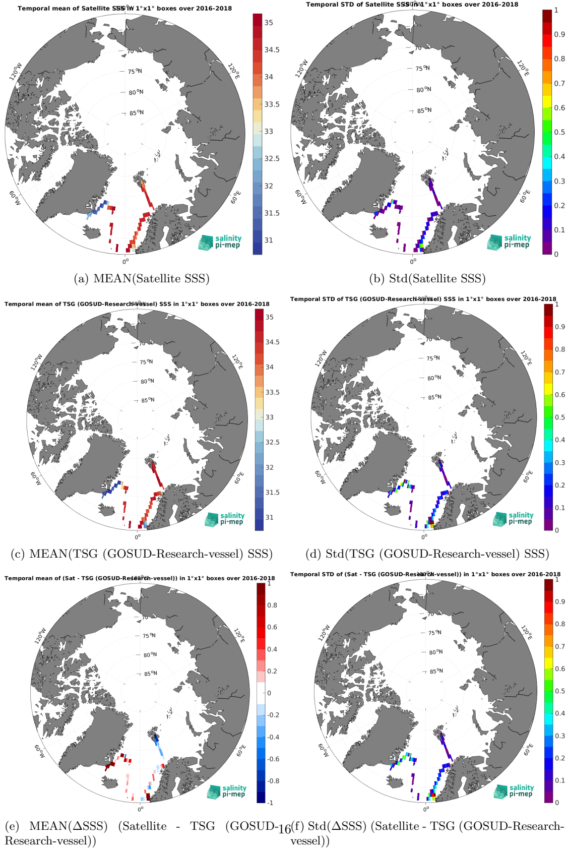
Figure 7: Temporal mean (left) and Std (right) of SSS from SMAP SSS L4 OI v3 - Daily (ESR) (top), TSG (GOSUD-Research-vessel) (middle), and of \Delta SSS (Satellite - TSG (GOSUD-Research-vessel)). Only match-up pairs are used to generate these maps.
