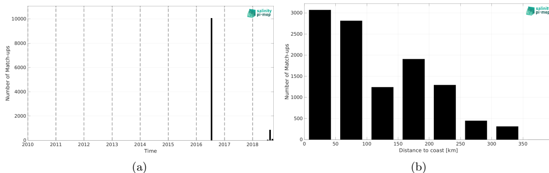
Figure 2: Number of match-ups between TSG (GOSUD-Research-vessel) and SMAP SSS L4 OI v3 - Daily (ESR) SSS as a function of time (a) and as function of the distance to coast (b) over the Arctic Ocean Pi-MEP region and for the full satellite product period.
