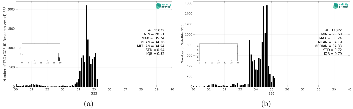
Figure 3: Histograms of SSS from TSG (GOSUD-Research-vessel) (a) and SMAP SSS L4 OI v3 - Daily (ESR) (b) considering all match-up pairs per bins of 0.1 over the Arctic Ocean Pi-MEP region and for the full satellite product period.
