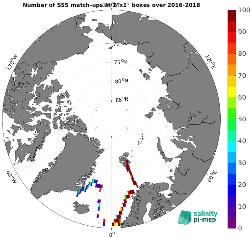
Figure 5: Number of SSS match-ups between TSG (GOSUD-Research-vessel) SSS and the SMAP SSS L4 OI v3 - Daily (ESR) SSS product for the Arctic Ocean Pi-MEP region over 1^\circ \times 1^\circ boxes and for the full satellite product period.
