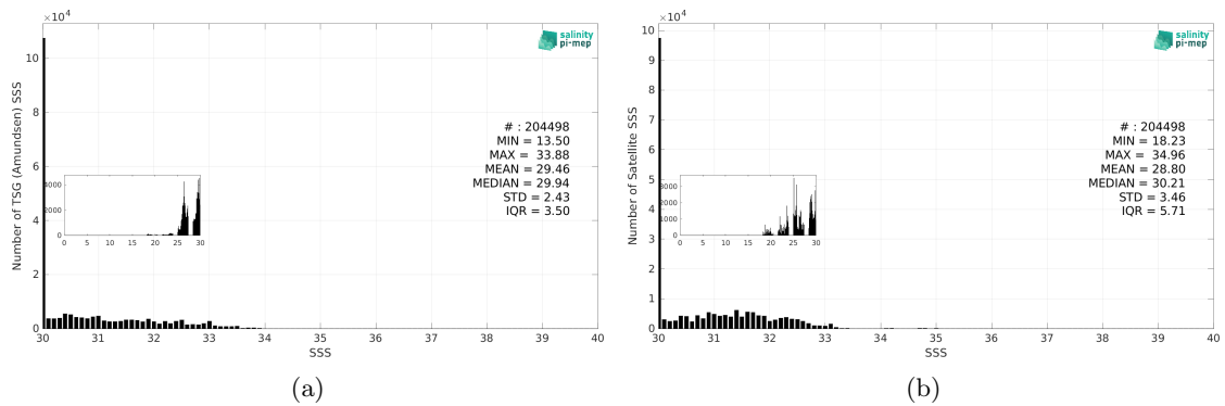
Figure 3: Histograms of SSS from TSG (Amundsen) (a) and SMAP SSS L4 OI v3 - Daily (ESR) (b) considering all match-up pairs per bins of 0.1 over the Arctic Ocean Pi-MEP region and for the full satellite product period.
