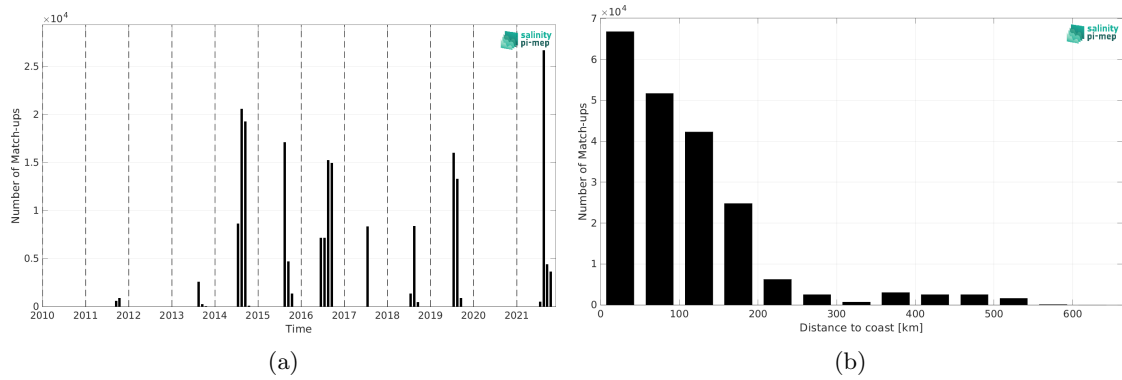
Figure 2: Number of match-ups between TSG (Amundsen) and SMAP SSS L4 OI v3 - Daily (ESR) SSS as a function of time (a) and as function of the distance to coast (b) over the Arctic Ocean Pi-MEP region and for the full satellite product period.
