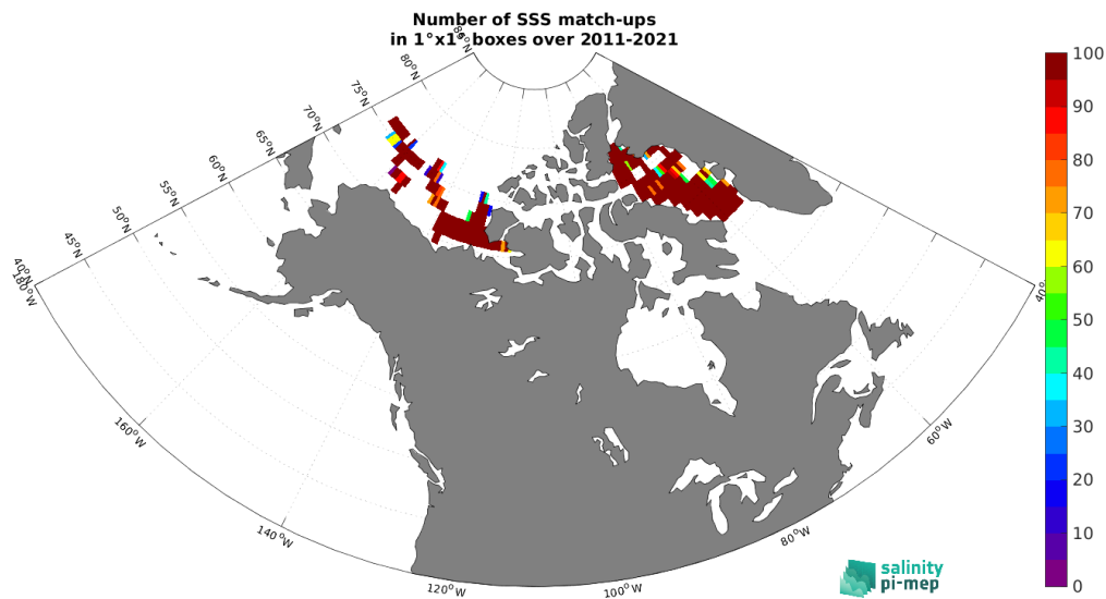
Figure 5: Number of SSS match-ups between TSG (Amundsen) SSS and the SMAP SSS L4 OI v3 - Daily (ESR) SSS product for the Arctic Ocean Pi-MEP region over 1^\circ \times 1^\circ boxes and for the full satellite product period.
