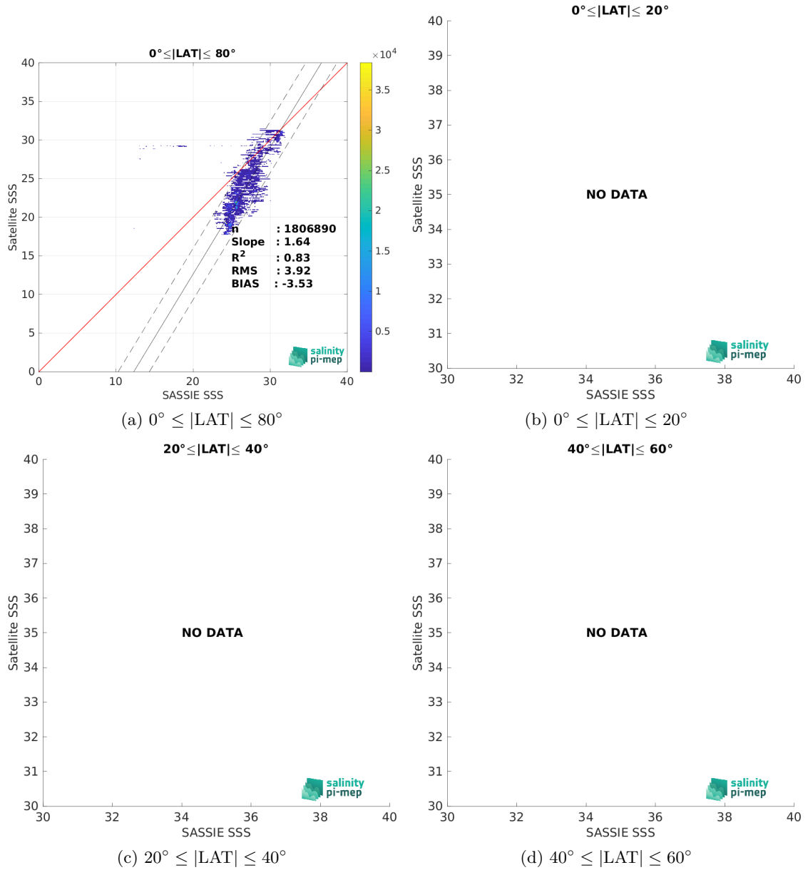
Figure 10: Contour maps of the concentration of SMAP SSS L4 OI v3 - Daily (ESR) SSS (y-axis) versus SASSIE SSS (x-axis) at match-up pairs for different latitude bands. For each plot, the red line shows x=y . The black thin and dashed lines indicate a linear fit through the data cloud and the \pm 95\% confidence levels, respectively. The number match-up pairs n , the slope and R^2 coefficient of the linear fit, the root mean square (RMS) and the mean bias between satellite and in situ data are indicated for each latitude band in each plots.
