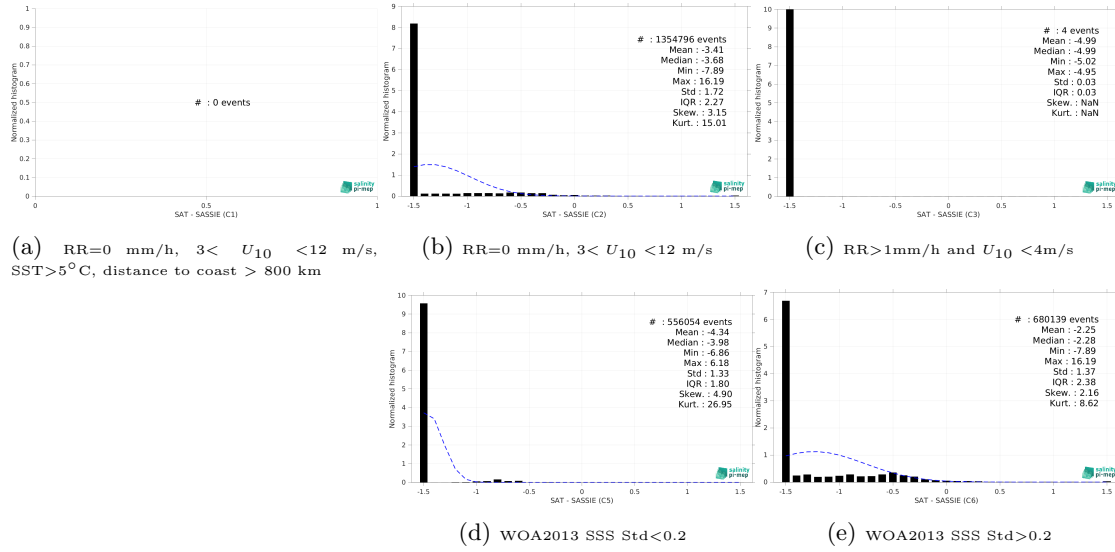
Figure 15: Normalized histogram of \Delta SSS (SMAP SSS L4 OI v3 - Daily (ESR) - SASSIE) for 5 different subdatasets corresponding to: RR=0 mm/h, 3 < U_{10} < 12 m/s, SST>5°C, distance to coast > 800 km (a), RR=0 mm/h, 3 < U_{10} < 12 m/s (b), RR>1mm/h and U_{10} < 4 m/s (c), WOA2013 SSS Std<0.2 (d), WOA2013 SSS Std>0.2 (e).
