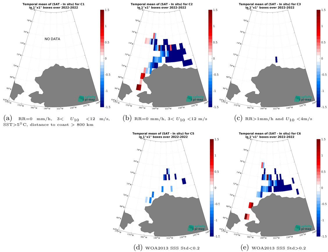
Figure 14: Temporal mean gridded over spatial boxes of size 1^\circ \times 1^\circ of \Delta SSS (SMAP SSS L4 OI v3 - Daily (ESR) - SASSIE) for 5 different subdatasets corresponding to:RR=0 mm/h, 3 < U_{10} < 12 m/s, SST >5^\circ\text{C} , distance to coast > 800 km (a), RR=0 mm/h, 3 < U_{10} < 12 m/s (b), RR >1 mm/h and U_{10} < 4 m/s (c), WOA2013 SSS Std <0.2 (d), WOA2013 SSS Std >0.2 (e).
