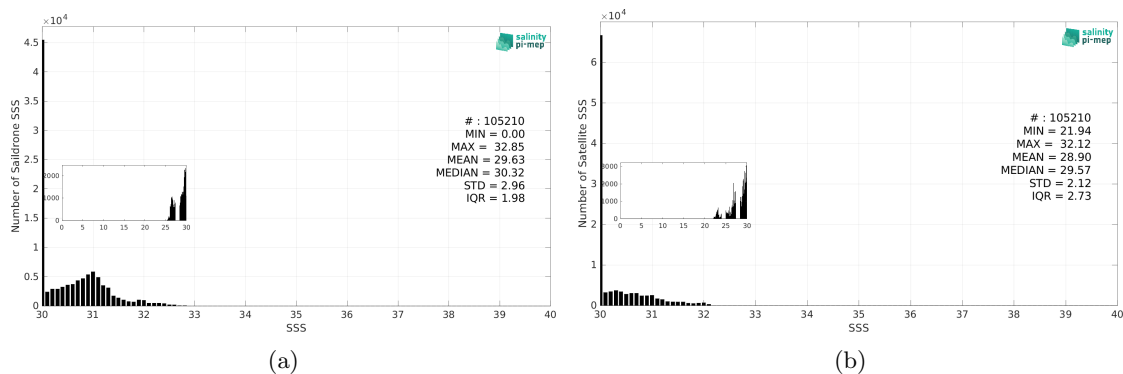
Figure 3: Histograms of SSS from Saildrone (a) and SMAP SSS L4 OI v3 - Daily (ESR) (b) considering all match-up pairs per bins of 0.1 over the Arctic Ocean Pi-MEP region and for the full satellite product period.
