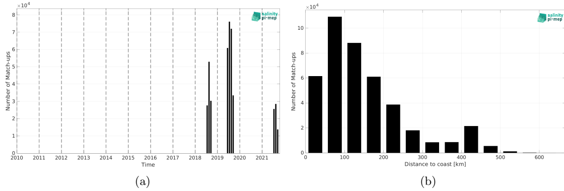
Figure 2: Number of match-ups between Sailldrone and SMAP SSS L4 OI v3 - Daily (ESR) SSS as a function of time (a) and as function of the distance to coast (b) over the Arctic Ocean Pi-MEP region and for the full satellite product period.
