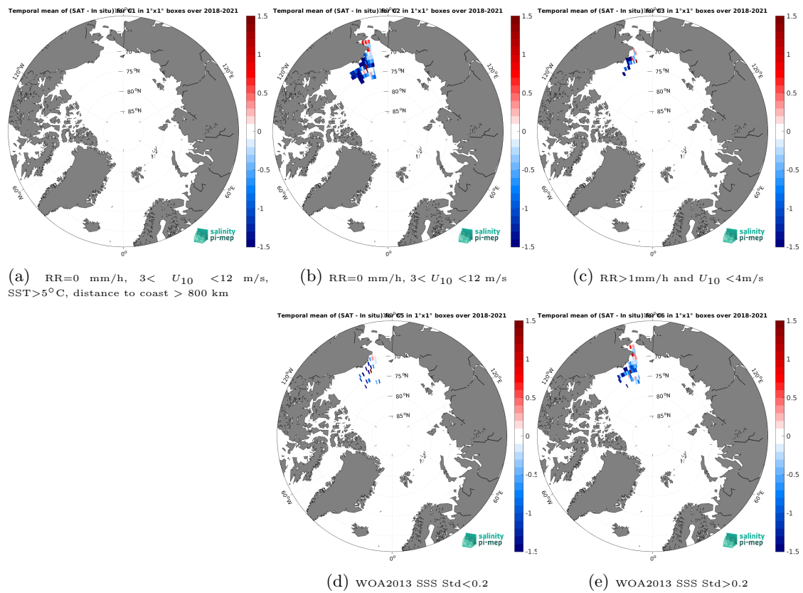
Figure 14: Temporal mean gridded over spatial boxes of size 1^\circ \times 1^\circ of \Delta SSS (SMAP SSS L4 OI v3 - Daily (ESR) - Saildrone) for 5 different subdatasets corresponding to: RR=0 mm/h, 3 < U_{10} < 12 m/s, SST > 5°C, distance to coast > 800 km (a), RR=0 mm/h, 3 < U_{10} < 12 m/s (b), RR > 1mm/h and U_{10} < 4 m/s (c), WOA2013 SSS Std < 0.2 (d), WOA2013 SSS Std > 0.2 (e).
