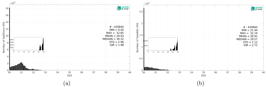
Figure 3: Histograms of SSS from Sailldrone (a) and SMAP SSS L4 OI v3 - Daily (ESR) (b) considering all match-up pairs per bins of 0.1 over the Arctic Ocean Pi-MEP region and for the full satellite product period.
