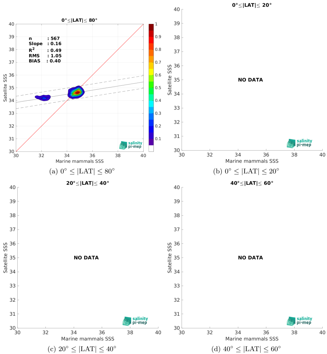
Figure 10: Contour maps of the concentration of SMAP SSS L4 OI v3 - Daily (ESR) SSS (y-axis) versus Marine mammals SSS (x-axis) at match-up pairs for different latitude bands. For each plot, the red line shows x=y . The black thin and dashed lines indicate a linear fit through the data cloud and the \pm 95\% confidence levels, respectively. The number match-up pairs n , the slope and R^2 coefficient of the linear fit, the root mean square (RMS) and the mean bias between satellite and in situ data are indicated for each latitude band in each plots.
