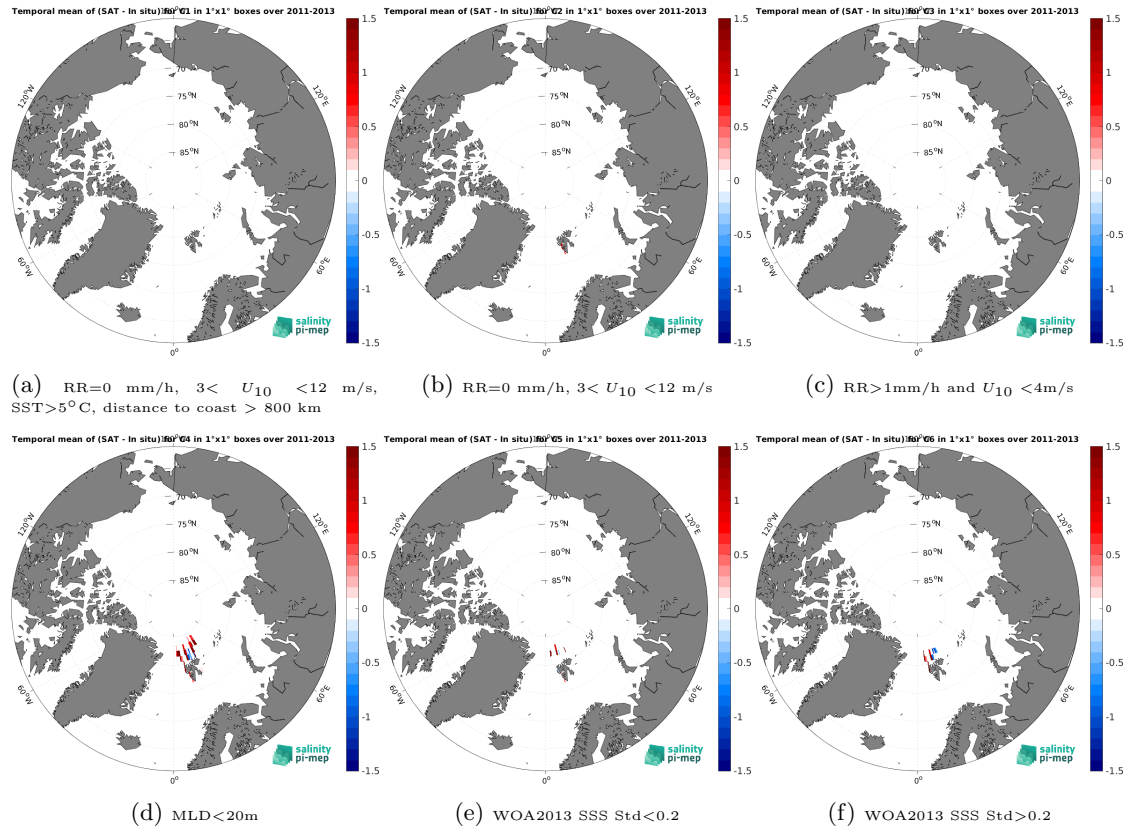
Figure 14: Temporal mean gridded over spatial boxes of size 1^\circ \times 1^\circ of \Delta SSS (SMAP SSS L4 OI v3 - Daily (ESR) - Marine mammals) for 6 different subdatasets corresponding to:RR=0 mm/h, 3 < U_{10} < 12 m/s, SST>5°C, distance to coast > 800 km (a), RR=0 mm/h, 3 < U_{10} < 12 m/s (b), RR>1mm/h and U_{10} < 4 m/s (c),MLD<20m (d),WOA2013 SSS Std<0.2 (e),WOA2013 SSS Std>0.2 (f).
