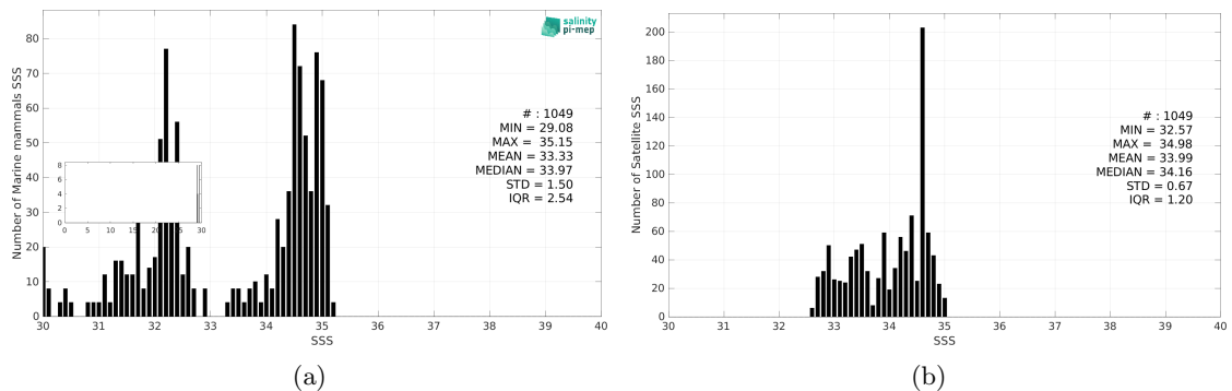
Figure 3: Histograms of SSS from Marine mammals (a) and SMAP SSS L4 OI v3 - Daily (ESR) (b) considering all match-up pairs per bins of 0.1 over the Arctic Ocean Pi-MEP region and for the full satellite product period.
