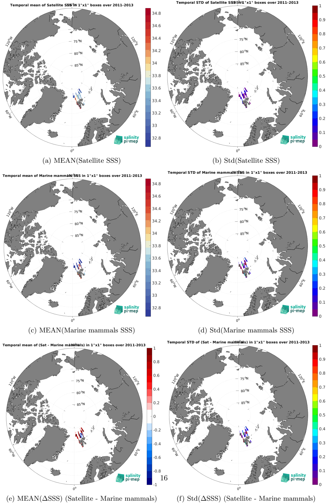
Figure 7: Temporal mean (left) and Std (right) of SSS from SMAP SSS L4 OI v3 - Daily (ESR) (top), Marine mammals (middle), and of \Delta SSS (Satellite - Marine mammals). Only match-up pairs are used to generate these maps.
