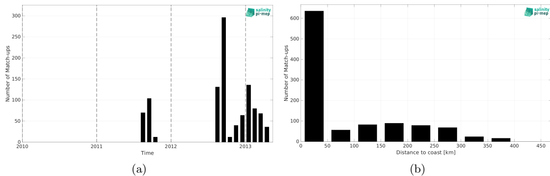
Figure 2: Number of match-ups between Marine mammals and SMAP SSS L4 OI v3 - Daily (ESR) SSS as a function of time (a) and as function of the distance to coast (b) over the Arctic Ocean Pi-MEP region and for the full satellite product period.
